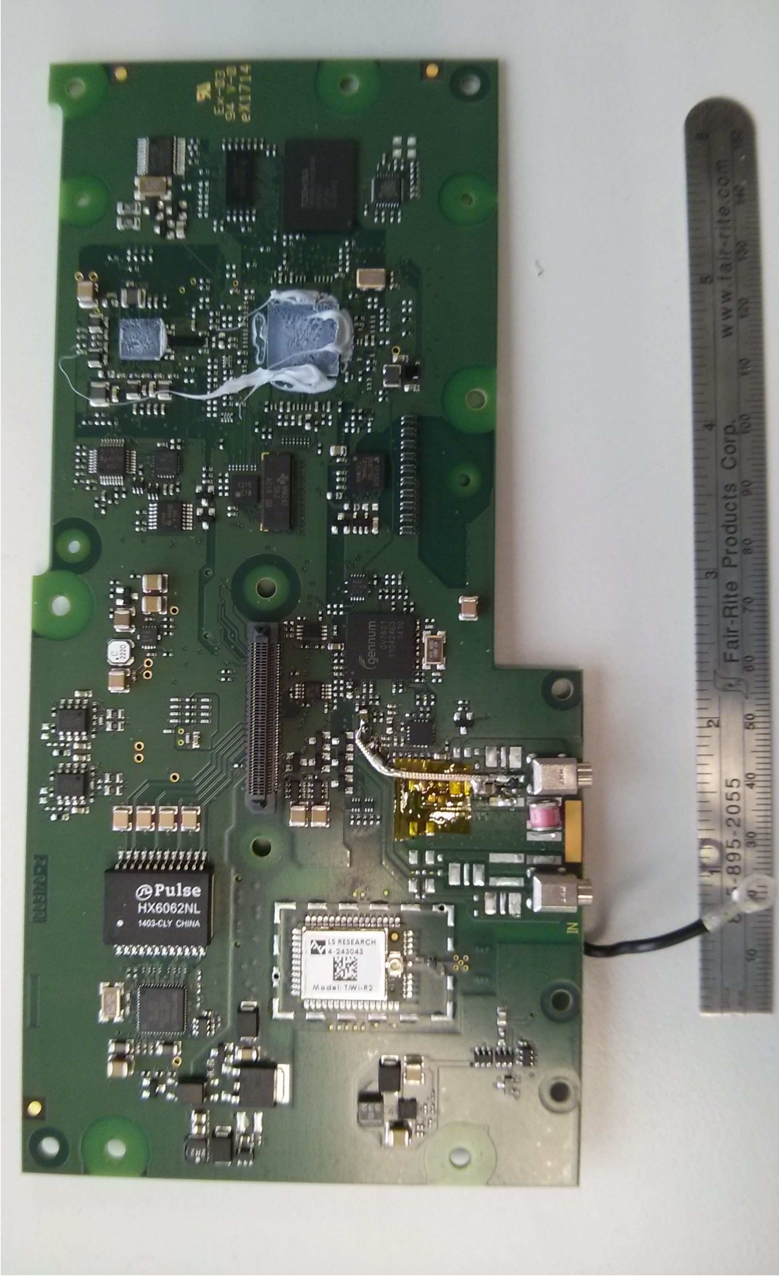
Figure 7 – CPU PCB Top – heat sink removed
