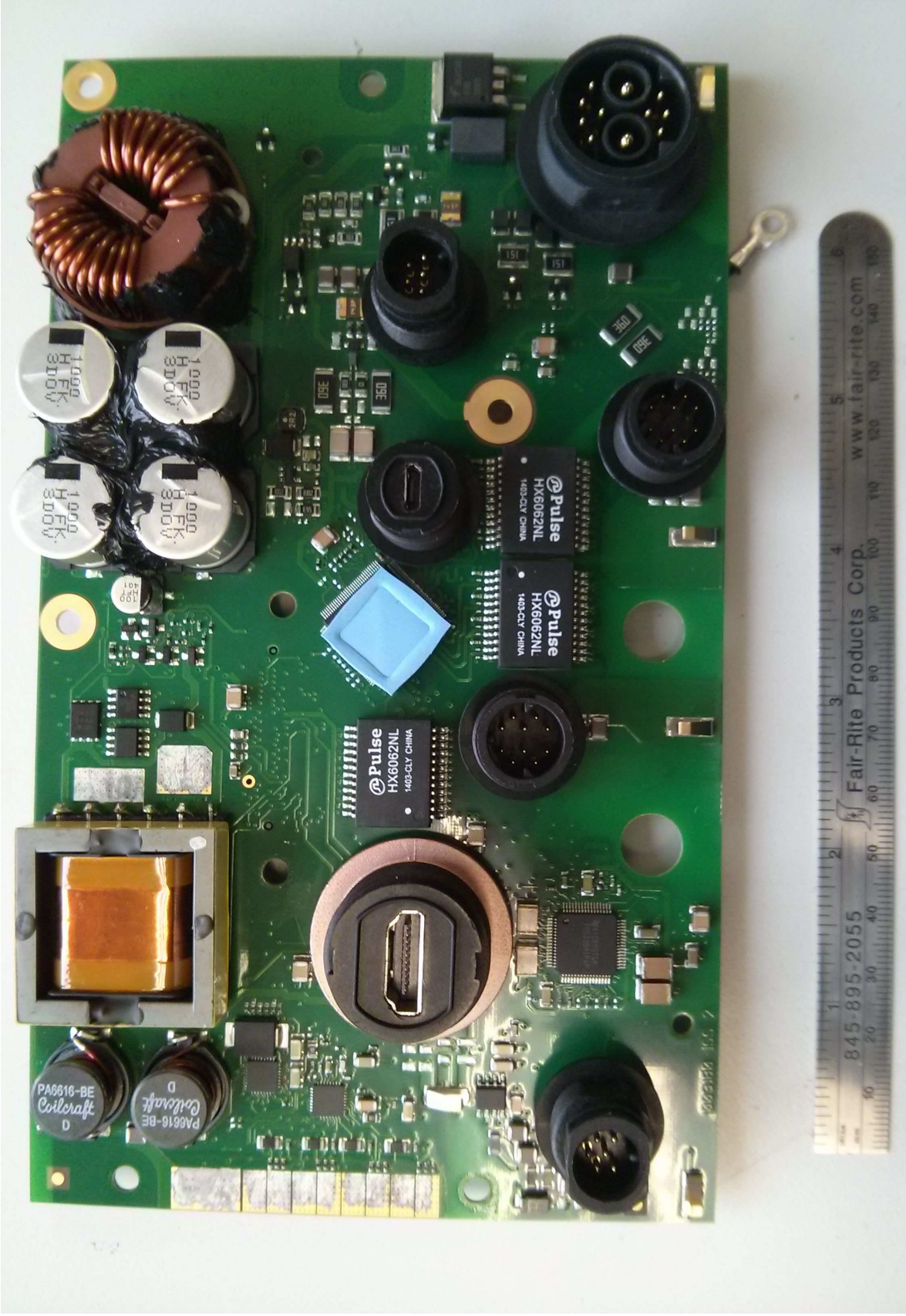
Figure 10 – I/O PCB Top – Gasket removed
