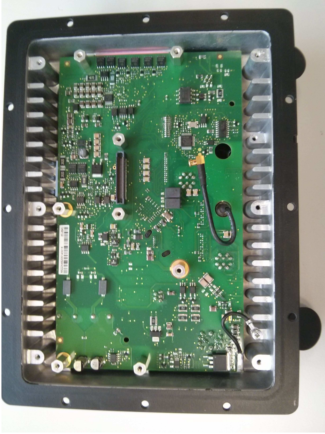
Figure 8 – I/O PCB Bottom
