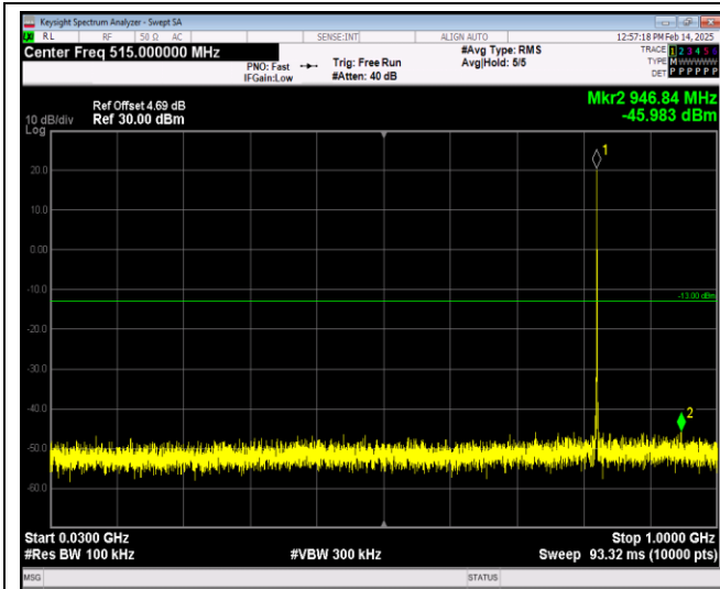
Band26-1.4MHz-16QAM-26915-1RB#0-Range1:30~1000MHz
