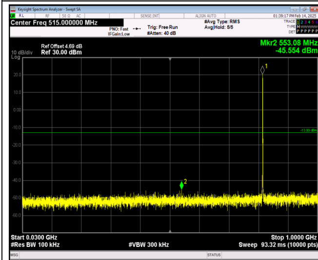
Band26-1.4MHz-QPSK-26740-1RB#0-Range1:30~1000MHz
