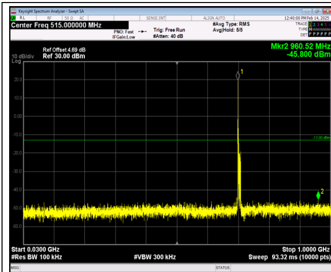
Band26-1.4MHz-QPSK-26697-1RB#0-Range1:30~1000MHz
