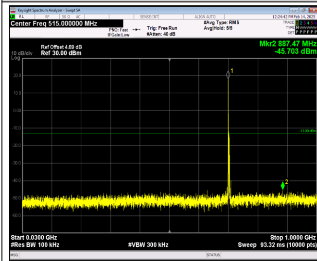
Band17-5MHz-16QAM-23790-1RB#0-Range1:30~1000MHz
