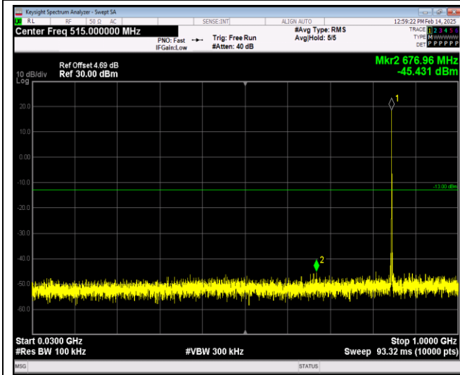
Band26-1.4MHz-16QAM-27033-1RB#0-Range1:30~1000MHz
