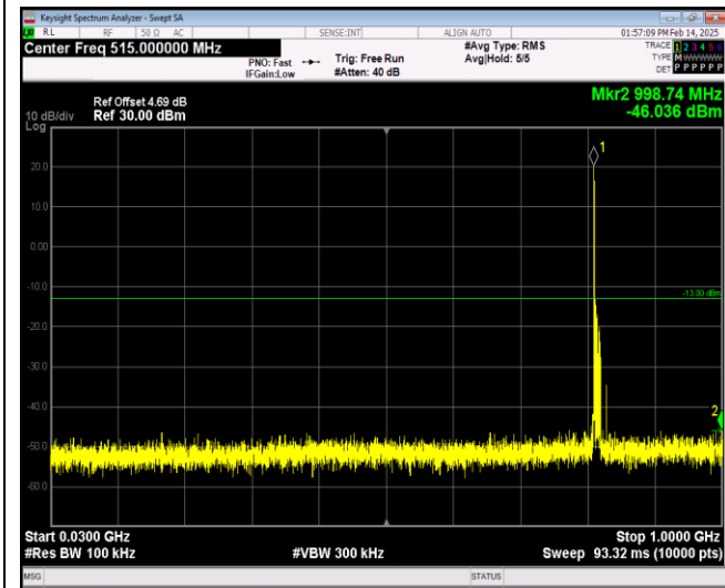
Band26-15MHz-QPSK-26865-1RB#0-Range1:30~1000MHz
