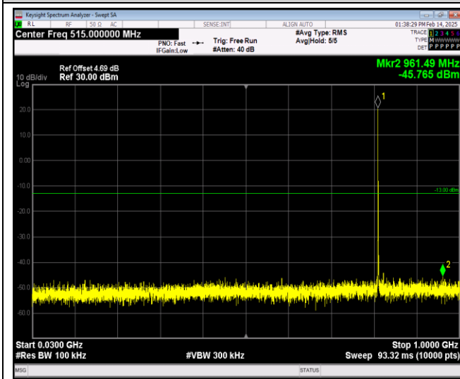
Band26-1.4MHz-16QAM-26697-1RB#0-Range1:30~1000MHz
