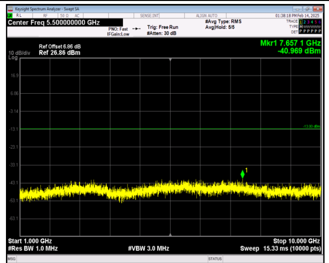
Band26-1.4MHz-QPSK-26740-1RB#0-Range2:1000~10000MHz
