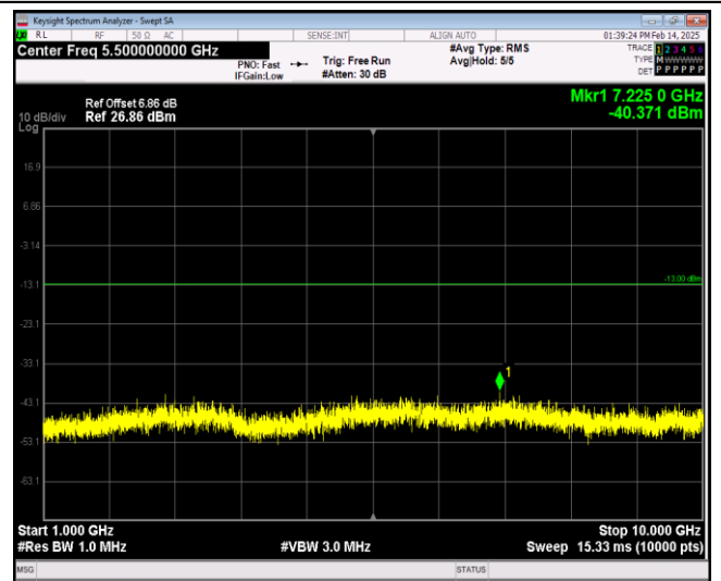
Band26-1.4MHz-QPSK-26740-1RB#0-Range2:1000~10000MHz
