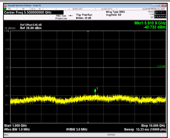
Band17-5MHz-16QAM-23790-1RB#0-Range2:1000~10000MHz
