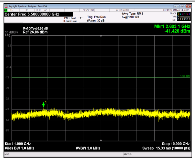
Band26-1.4MHz-16QAM-26697-1RB#0-Range2:1000~10000MHz
