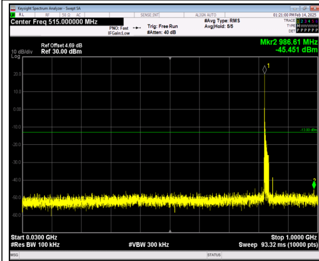
Band26-15MHz-QPSK-26865-1RB#0-Range1:30~1000MHz
