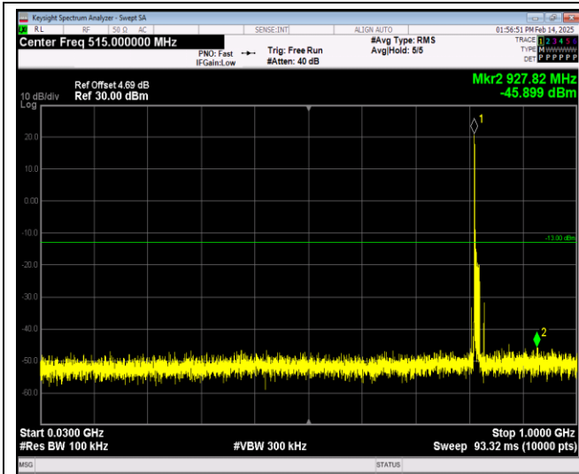
Band26-10MHz-64QAM-26740-1RB#0-Range1:30~1000MHz
