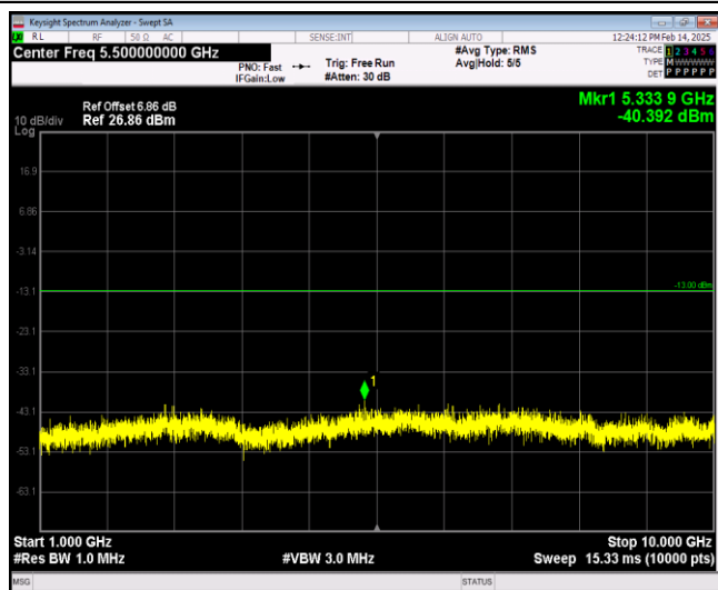
Band17-5MHz-64QAM-23790-1RB#0-Range2:1000~10000MHz
