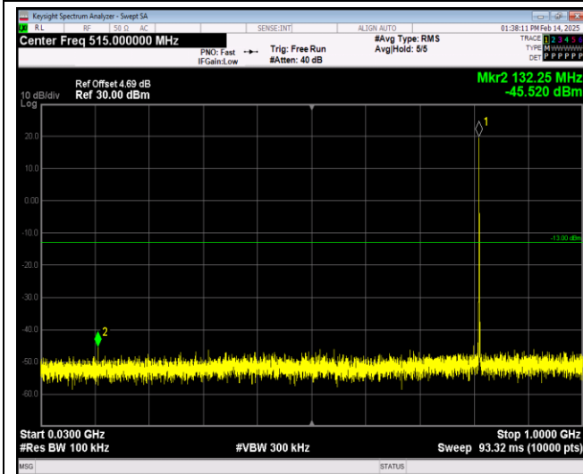
Band26-1.4MHz-QPSK-26740-1RB#0-Range1:30~1000MHz
