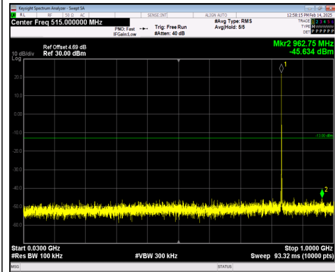
Band26-1.4MHz-16QAM-27033-1RB#0-Range1:30~1000MHz
