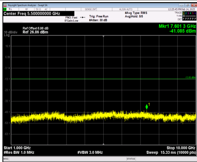
Band17-5MHz-64QAM-23755-1RB#0-Range2:1000~10000MHz
