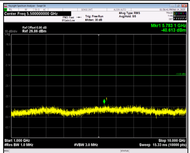
Band26-10MHz-16QAM-26740-1RB#0-Range2:1000 ~10000MHz
