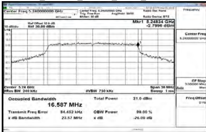
FCC_802.11a_20MHz_AUX1_5240MHz
