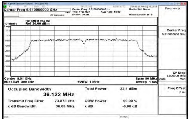
IC_802.11n_40MHz_AUX1_5510MHz
