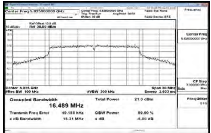
FCC_802.11a_20MHz_Main_5825MHz
