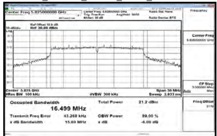
FCC_802.11a_20MHz_AUX1_5825MHz
