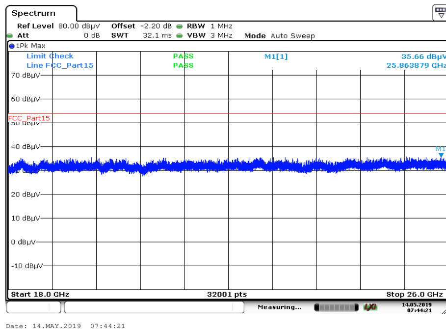
Plot 2: 18 GHz to 26 GHz, RX / idle – mode, vertical & horizontal polarization, antenna 1
