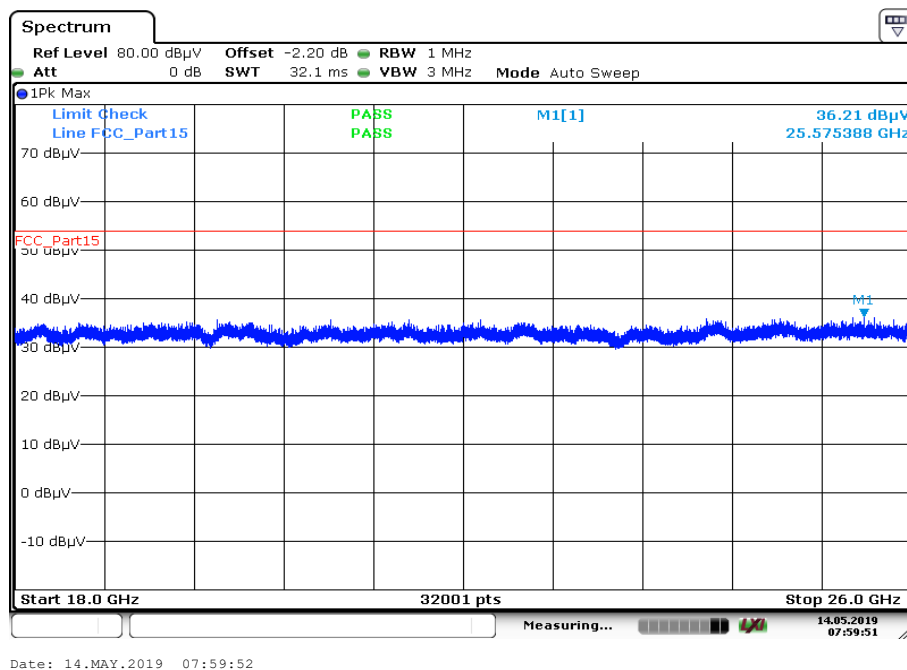
Plot 10: 18 GHz to 26 GHz, TX mode, 2443 MHz, vertical & horizontal polarization, antenna 2
