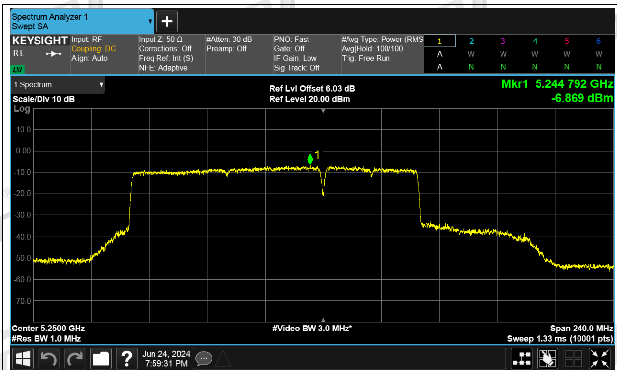
PSD NVNT be160 996+484-tone in a non-OFDMA MRU4 5250MHz Ant3
