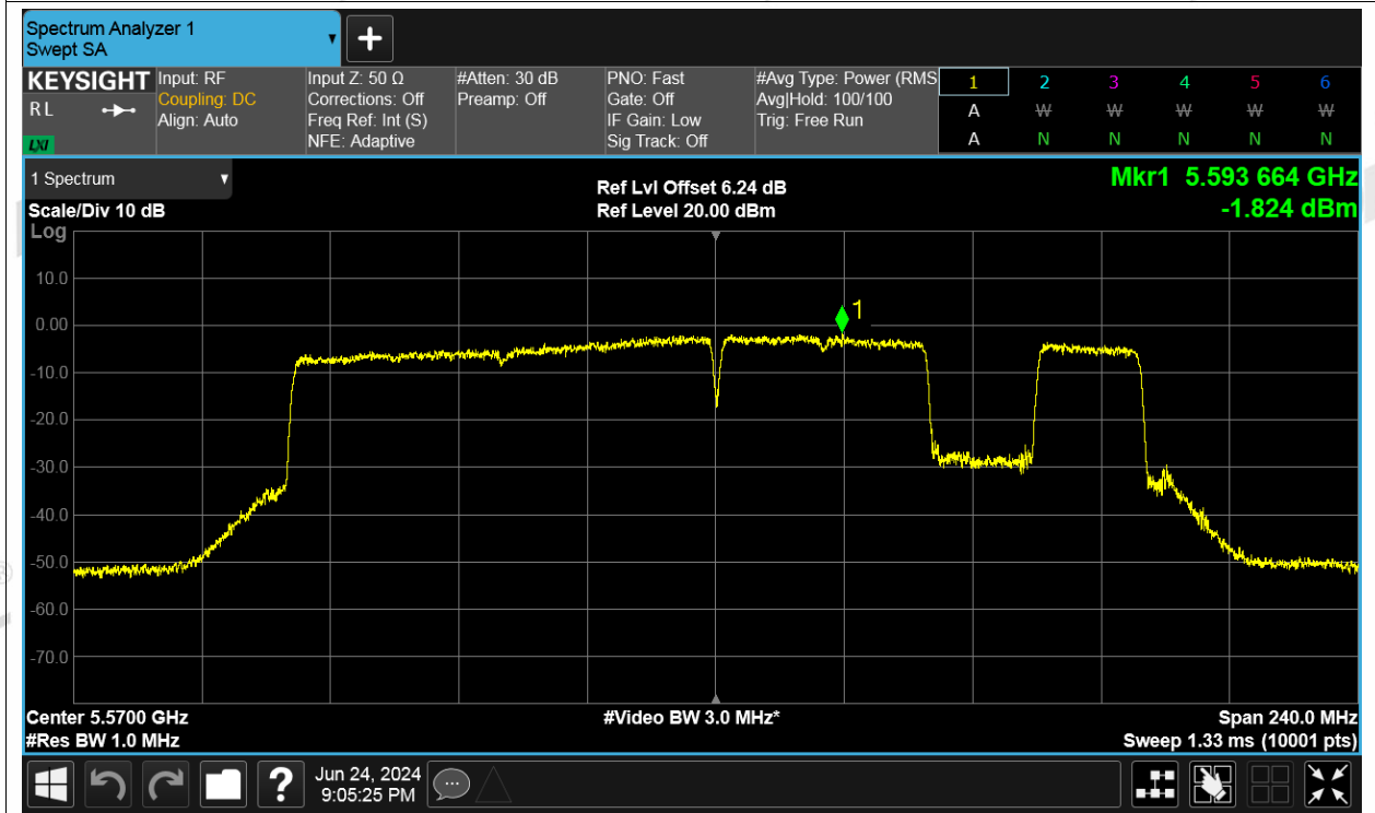
PSD NVNT be160 996+484+242-tone in a non-OFDMA MRU7 5570MHz Ant3
