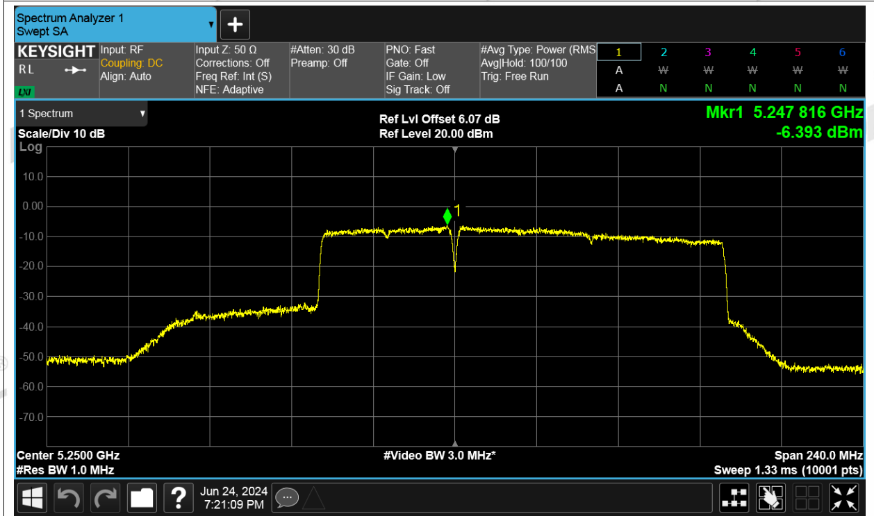
PSD NVNT be160 996+484-tone in a non-OFDMA MRU1 5250MHz Ant2
