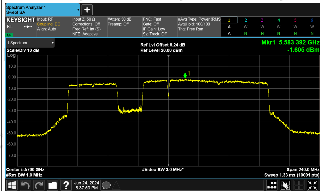
PSD NVNT be160 996+484+242-tone in a non-OFDMA MRU3 5570MHz Ant3
