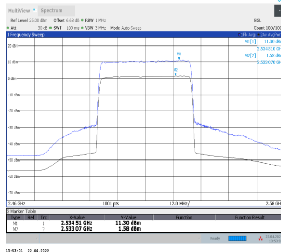
1-N7--15-40-L-2-CP-256QAM-Outer_Full-216@0-An t0-9.72-100%-0.00-9.72-PASS-≤13
