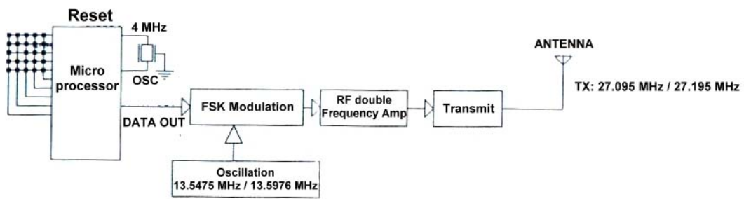
Transmitter (Keyboard) Block Diagram
