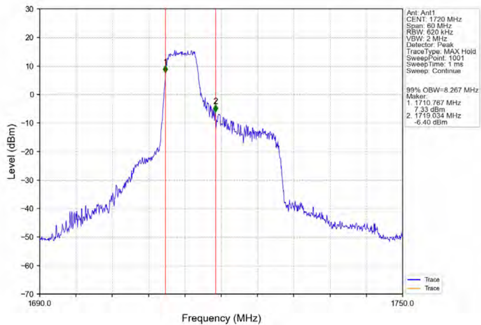
Band66_20MHz_16QAM_LCH_1720MHz_RB_27_0_NTNV
