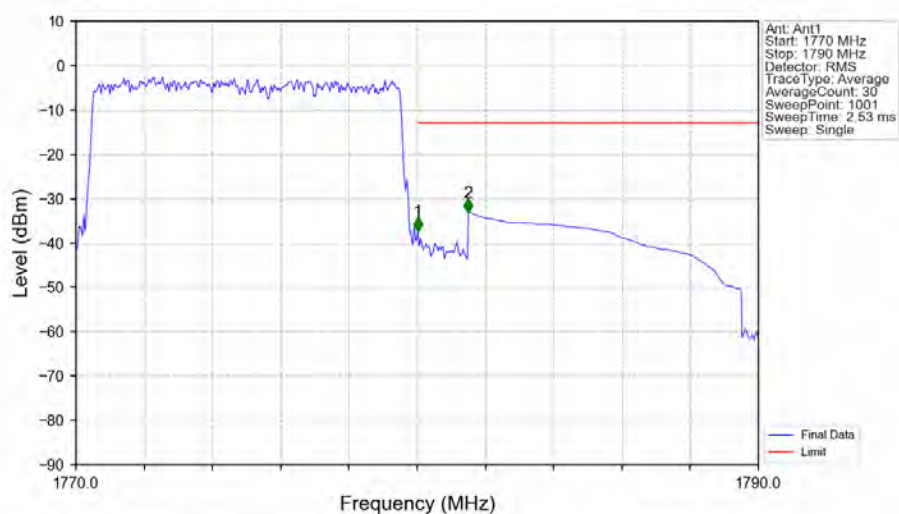
Band66_10MHz_QPSK_HCH_1775MHz_RB_50_0_NTNV
