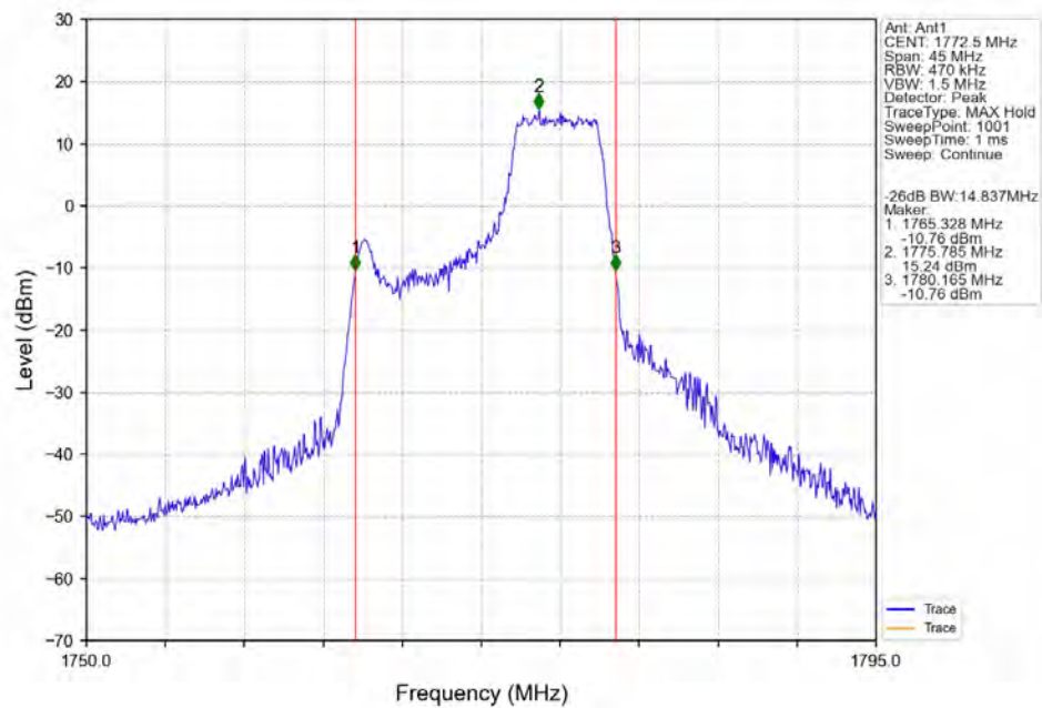
Band66_15MHz_16QAM_HCH_1772.5MHz_RB_27_48_NTNV
