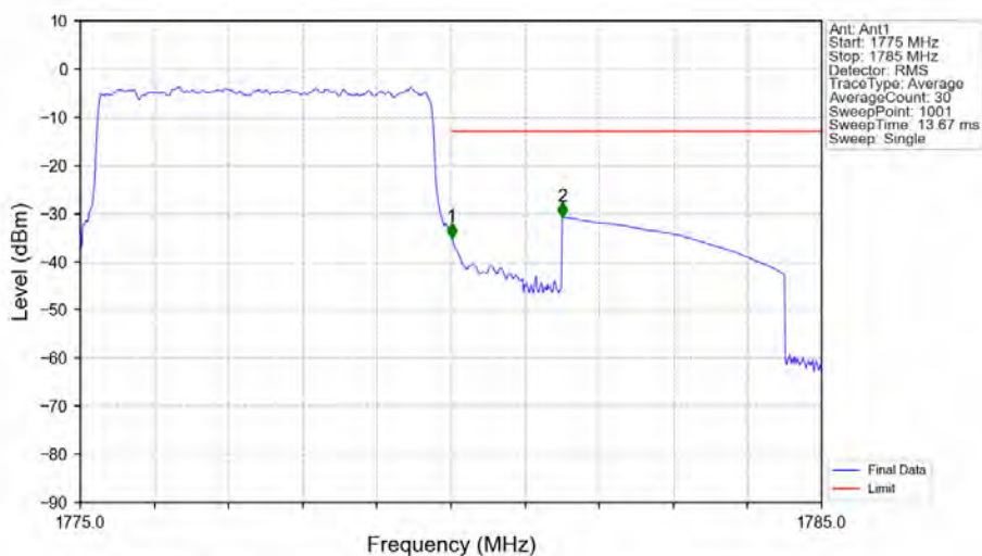
Band66_5MHz_QPSK_HCH_1777.5MHz_RB_25_0_NTNV
