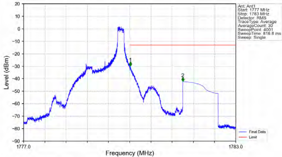
Band66 1.4MHz QPSK HCH 1779.3MHz RB 1 5 NTNV
