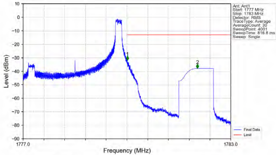
Band66_3MHz_16QAM_HCH_1778.5MHz_RB_1_14_NTNV
