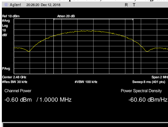
Plot 6. Maximum Conducted Output Power, 2480 MHz, Integrated Band Power
