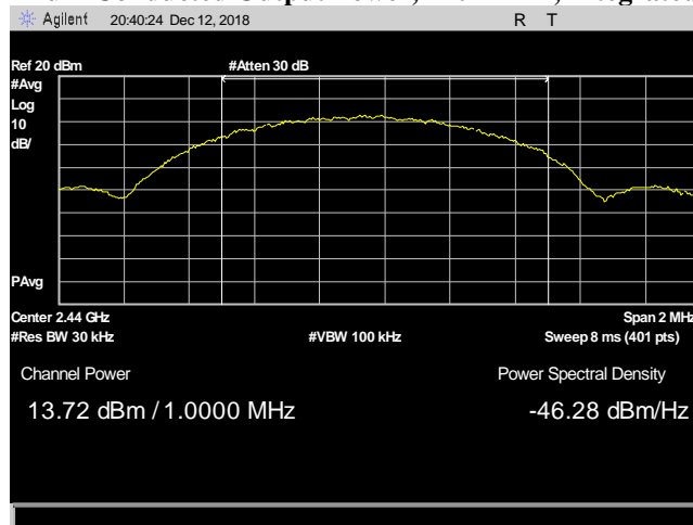
Plot 5. Maximum Conducted Output Power, 2440 MHz, Integrated Band Power
