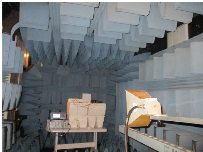
Figure 5. Radiated Emission Test 1.0 - 8.0GHz
