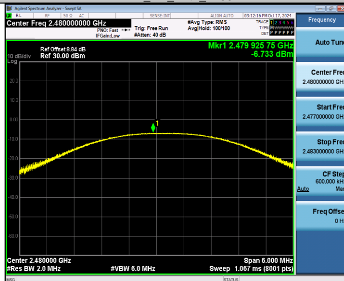
BLE_1M_Ant1_2480
