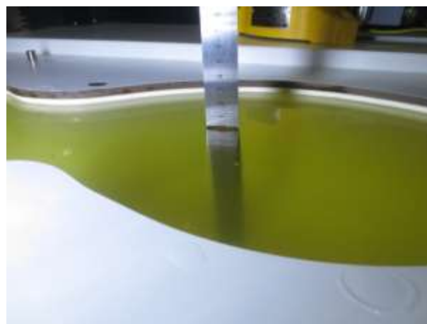
Fig. 9.2 Photo of Liquid Height for Body SAR of (700MHz~1000MHz) (depth>15cm)
