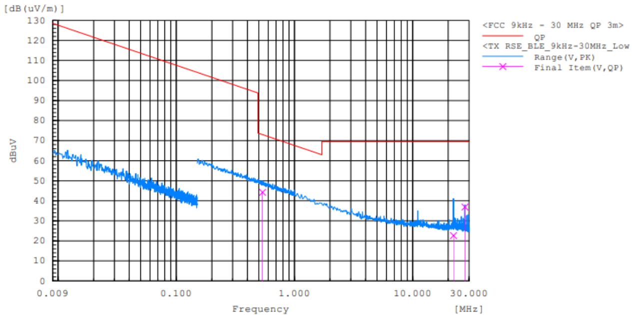
Radiated Spurious Emission 9 kHz – 30 MHz (Antenna Position 180°) : CH 0
