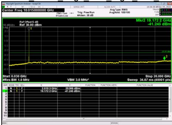
N7(10M)_DFT-s- OFDM BPSK Edge 1RB Right Low CH
