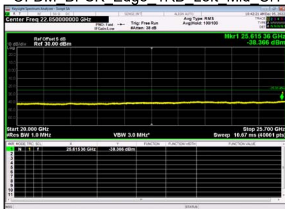
N7(10M)_DFT-s- OFDM BPSK Edge 1RB Left Mid CH
