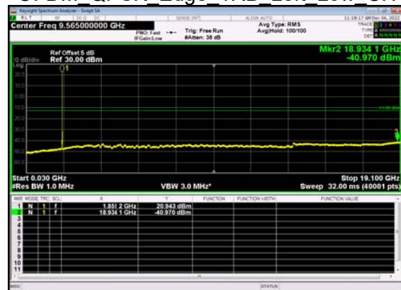
N2(15M)_DFT-s- OFDM QPSK Edge 1RB Left Low CH
