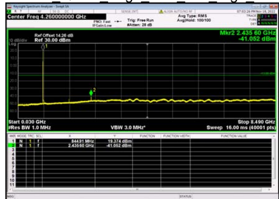
N5(5M)_DFT-s- OFDM QPSK Edge 1RB Left High CH
