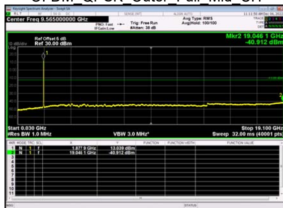
N2(10M)_DFT-s- OFDM QPSK Outer Full Mid CH
