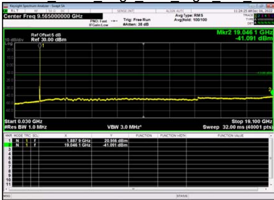
N2(15M)_DFT-s- OFDM BPSK Edge 1RB Right Mid CH
