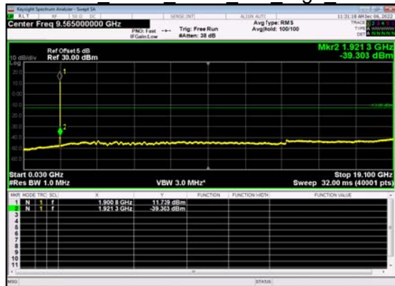
N2(15M)_DFT-s- OFDM BPSK Outer Full High CH
