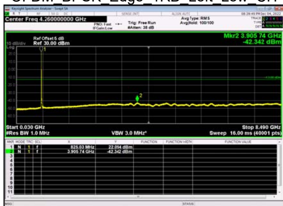
N5(15M)_DFT-s- OFDM BPSK Edge 1RB Left Low CH
