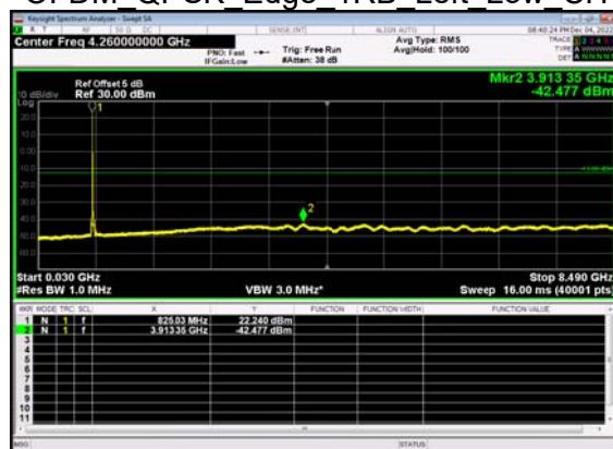
N5(15M)_DFT-s- OFDM QPSK Edge 1RB Left Low CH
