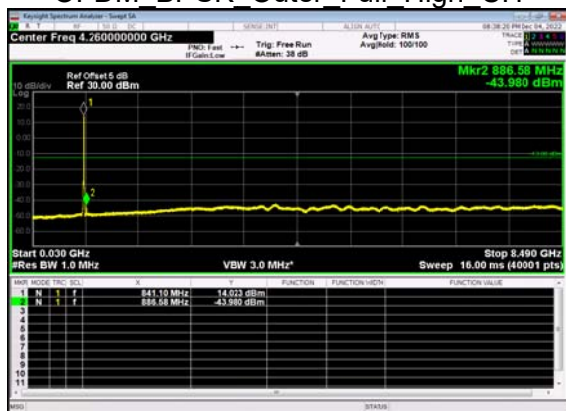
N5(10M)_DFT-s- OFDM BPSK Outer Full High CH
