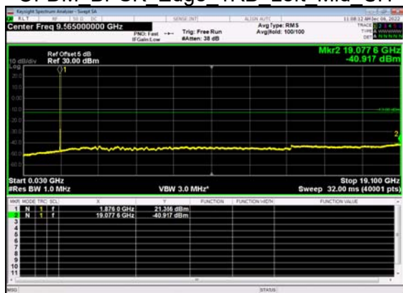
N2(10M)_DFT-s- OFDM BPSK Edge 1RB Left Mid CH
