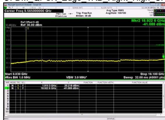
N2(10M)_DFT-s- OFDM QPSK Edge 1RB Right High CH
