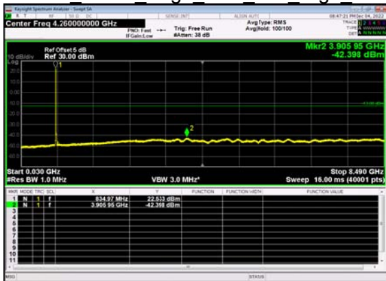
N5(15M)_DFT-s- OFDM BPSK Edge 1RB Left High CH
