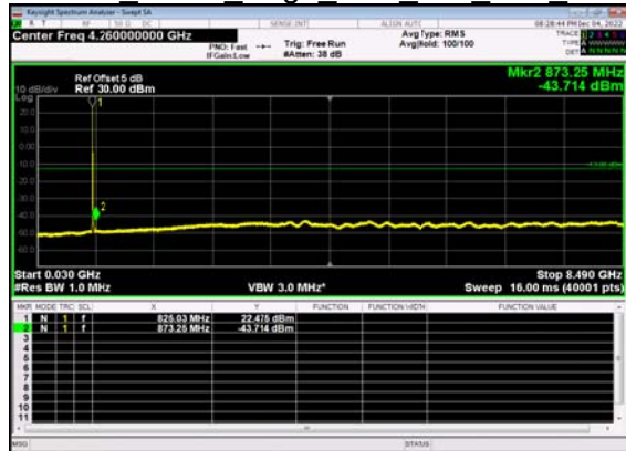
N5(10M)_DFT-s- OFDM BPSK Edge 1RB Left Low CH
