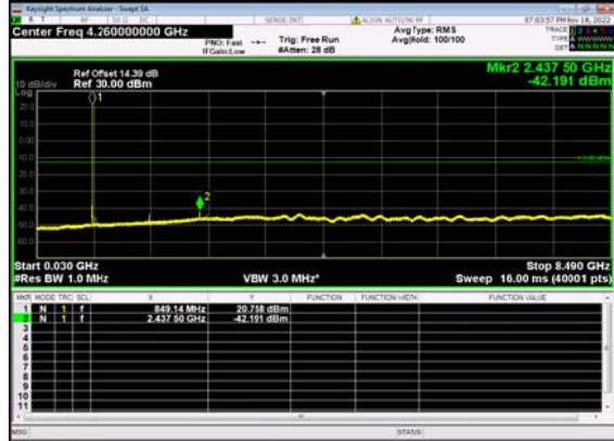
N5(5M)_DFT-s- OFDM BPSK Edge 1RB Right High CH
