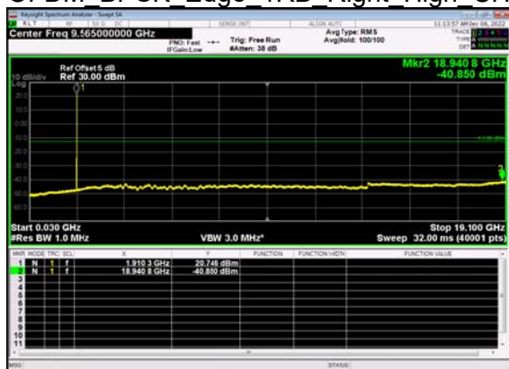
N2(10M)_DFT-s- OFDM BPSK Edge 1RB Right High CH
