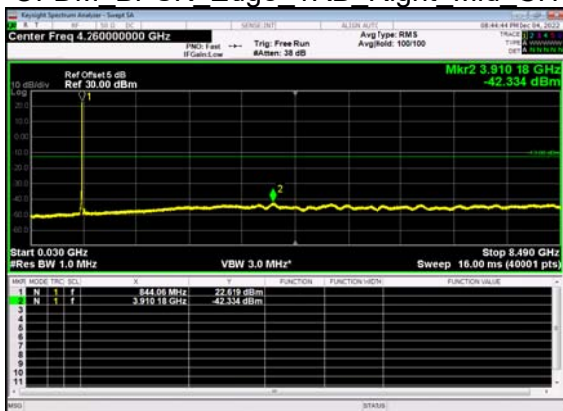
N5(15M)_DFT-s- OFDM BPSK Edge 1RB Right Mid CH
