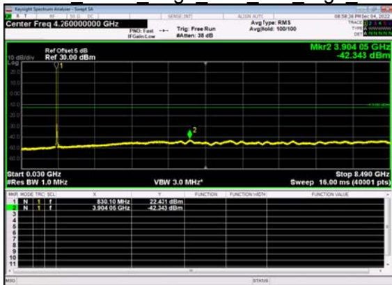
N5(20M)_DFT-s- OFDM BPSK Edge 1RB Left High CH
