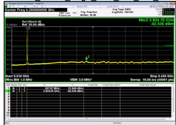
N5(20M)_DFT-s- OFDM QPSK Edge 1RB Left Mid CH
