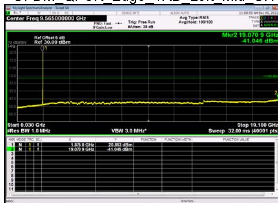
N2(10M)_DFT-s- OFDM QPSK Edge 1RB Left Mid CH
