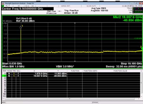
N2(15M)_DFT-s- OFDM BPSK Outer Full Mid CH
