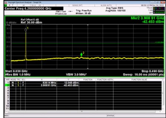
N5(15M)_DFT-s- OFDM QPSK Outer Full High CH
