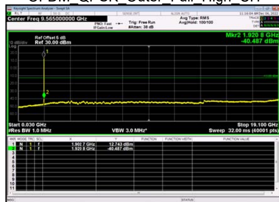
N2(10M)_DFT-s- OFDM QPSK Outer Full High CH
