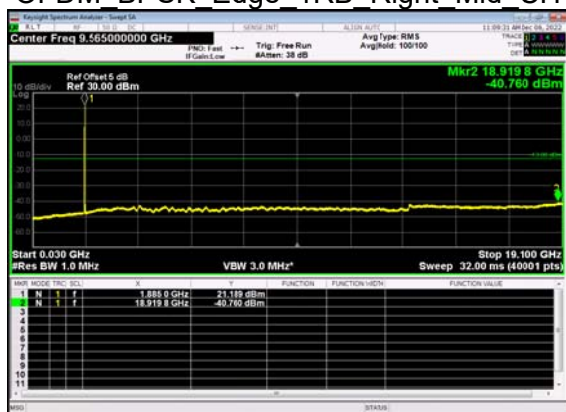
N2(10M)_DFT-s- OFDM BPSK Edge 1RB Right Mid CH
