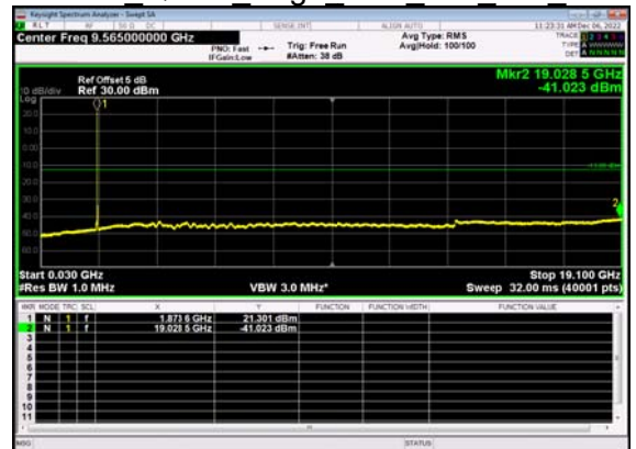
N2(15M)_DFT-s- OFDM QPSK Edge 1RB Left Mid CH
