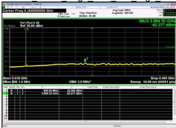
N5(10M)_DFT-s- OFDM BPSK Edge 1RB Left High CH
