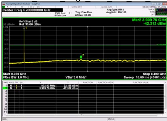
N5(10M)_DFT-s- OFDM BPSK Edge 1RB Left Mid CH
