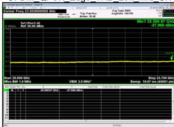
N7(10M)_DFT-s- OFDM QPSK Edge 1RB Left Mid CH
