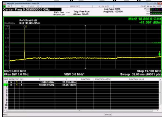
N2(15M)_DFT-s- OFDM BPSK Edge 1RB Right High CH
