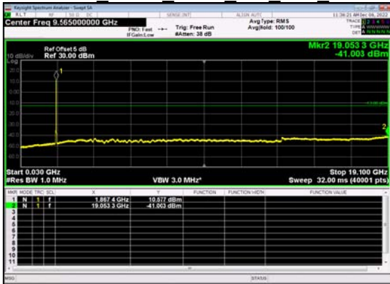
N2(20M)_DFT-s- OFDM BPSK Outer Full Low CH
