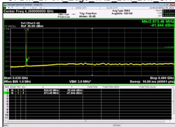
N5(5M)_DFT-s- OFDM BPSK Edge 1RB Left Low CH
