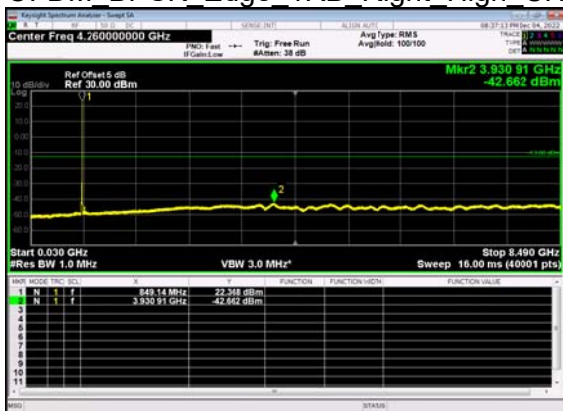
N5(10M)_DFT-s- OFDM BPSK Edge 1RB Right High CH
