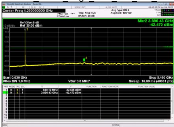
N5(15M)_DFT-s- OFDM BPSK Edge 1RB Left Mid CH
