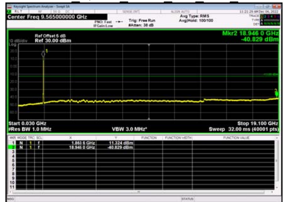
N2(15M)_DFT-s- OFDM QPSK Outer Full Low CH
