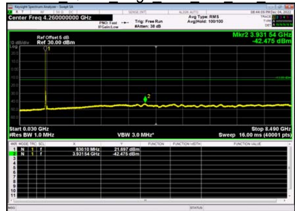
N5(15M)_DFT-s- OFDM QPSK Edge 1RB Left Mid CH
