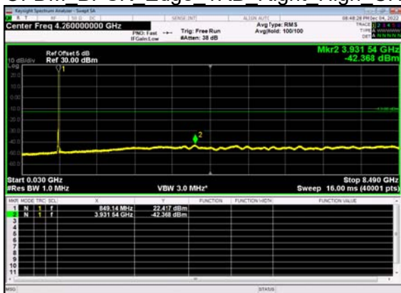
N5(15M)_DFT-s- OFDM BPSK Edge 1RB Right High CH
