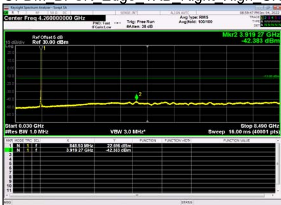
N5(20M)_DFT-s- OFDM BPSK Edge 1RB Right High CH
