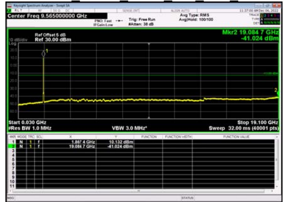
N2(20M)_DFT-s- OFDM QPSK Outer Full Low CH
