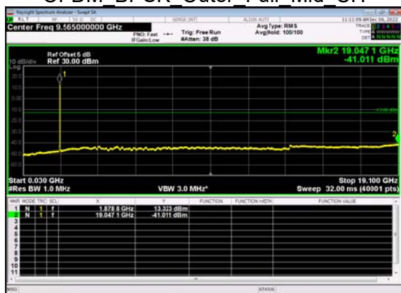
N2(10M)_DFT-s- OFDM BPSK Outer Full Mid CH
