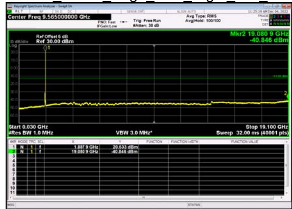
N2(15M)_DFT-s- OFDM QPSK Edge 1RB Right Mid CH
