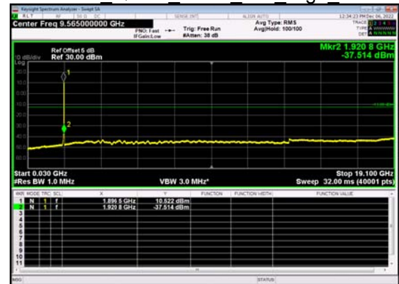
N2(20M)_DFT-s- OFDM QPSK Outer Full High CH
