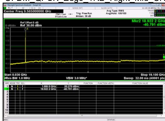
N2(10M)_DFT-s- OFDM QPSK Edge 1RB Right Mid CH
