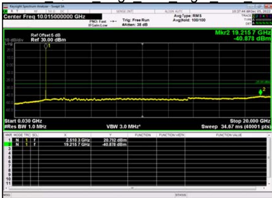
N7(10M)_DFT-s- OFDM QPSK Edge 1RB Right Low CH
