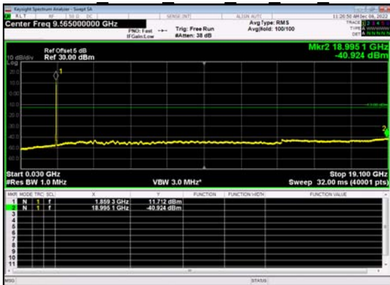
N2(15M)_DFT-s- OFDM BPSK Outer Full Low CH
