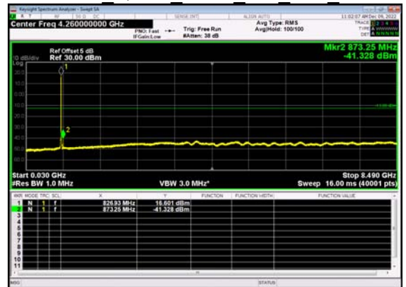
N5(5M)_DFT-s- OFDM QPSK Outer Full Low CH
