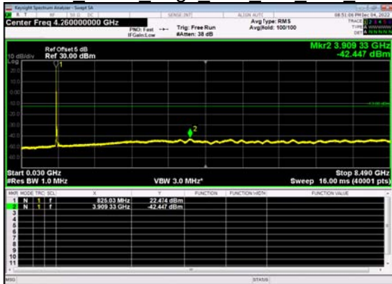
N5(20M)_DFT-s- OFDM BPSK Edge 1RB Left Low CH
