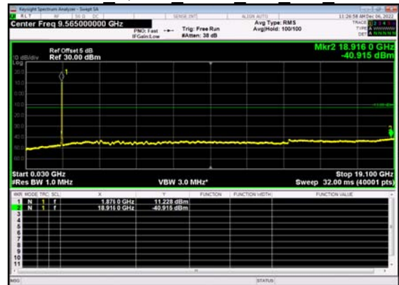
N2(15M)_DFT-s- OFDM QPSK Outer Full Mid CH
