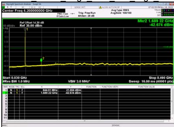
N5(5M)_DFT-s- OFDM BPSK Edge 1RB Left High CH
