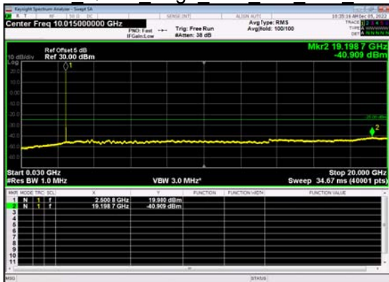
N7(10M)_DFT-s- OFDM QPSK Edge 1RB Left Low CH
