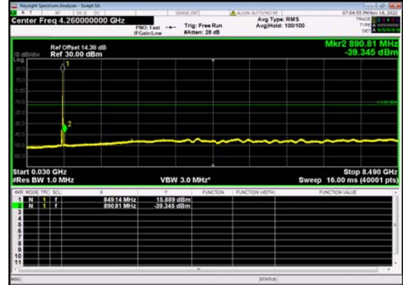
N5(5M)_DFT-s- OFDM BPSK Outer Full High CH
