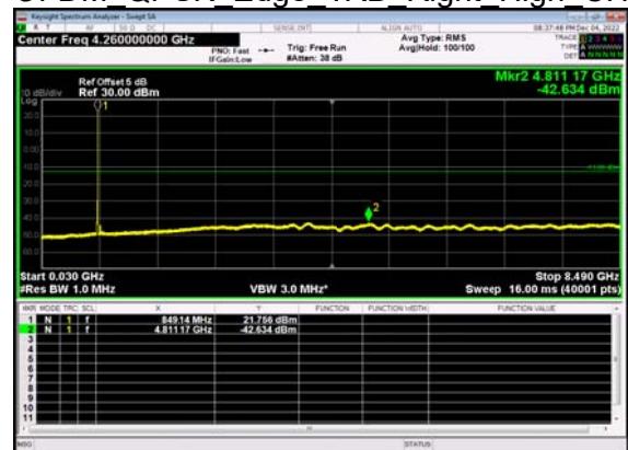
N5(10M)_DFT-s- OFDM QPSK Edge 1RB Right High CH
