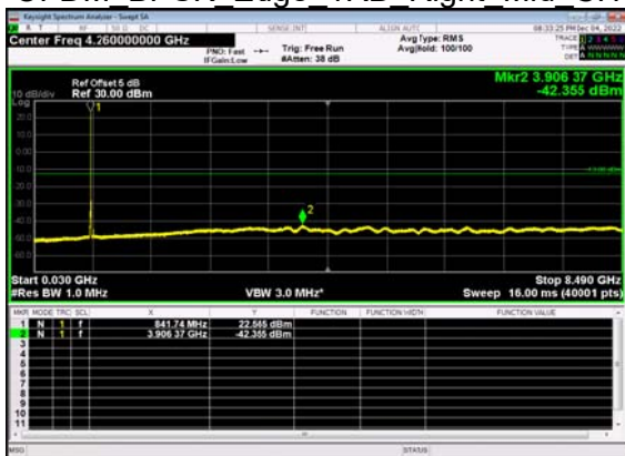
N5(10M)_DFT-s- OFDM BPSK Edge 1RB Right Mid CH
