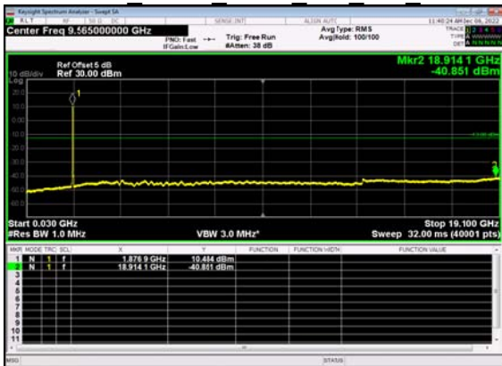
N2(20M)_DFT-s- OFDM BPSK Outer Full Mid CH
