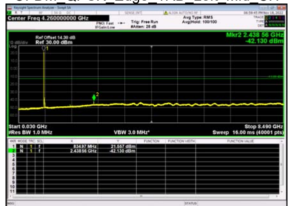
N5(5M)_DFT-s- OFDM QPSK Edge 1RB Left Mid CH
