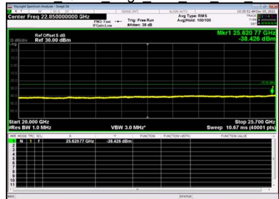
N7(10M)_DFT-s- OFDM QPSK Edge 1RB Left Low CH
