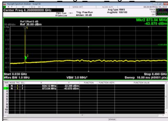
N5(10M)_DFT-s- OFDM BPSK Edge 1RB Right Low CH
