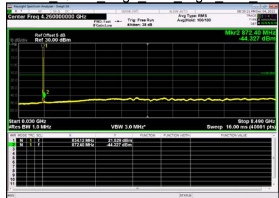
N5(10M)_DFT-s- OFDM QPSK Edge 1RB Right Low CH
