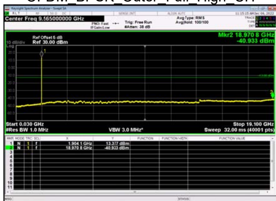
N2(10M)_DFT-s- OFDM BPSK Outer Full High CH
