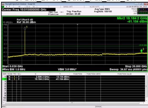
N7(10M)_DFT-s- OFDM BPSK Outer Full Low CH
