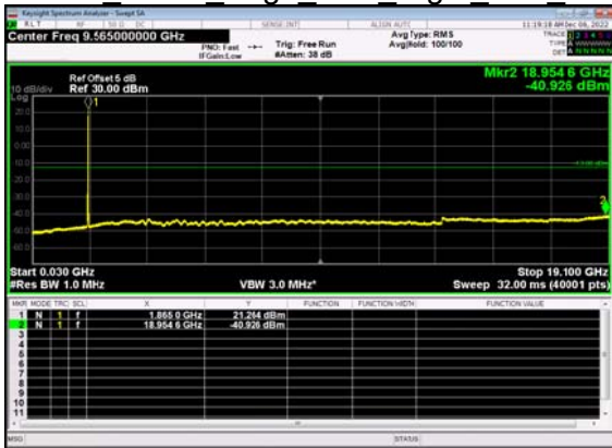
N2(15M)_DFT-s- OFDM BPSK Edge 1RB Right Low CH
