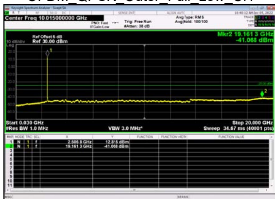
N7(10M)_DFT-s- OFDM QPSK Outer Full Low CH
