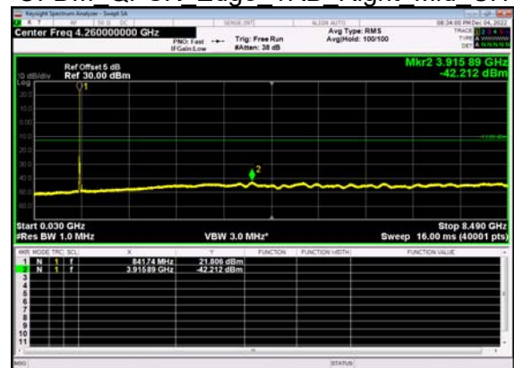
N5(10M)_DFT-s- OFDM QPSK Edge 1RB Right Mid CH
