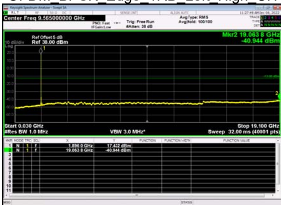
N2(15M)_DFT-s- OFDM BPSK Edge 1RB Left High CH
