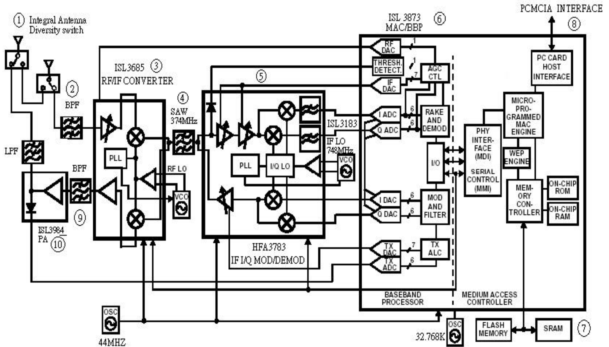
AWL100 PCMCIA wireless LAN Adapter Block Diagram
