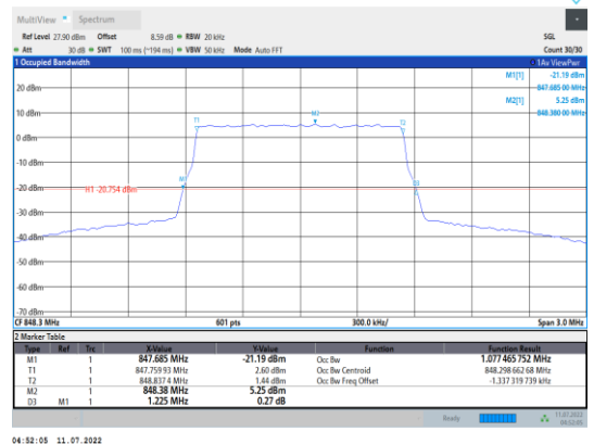
Band5-1.4MHz-16QAM-20643-6RB#0
