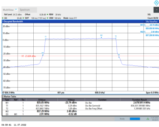
Band5-3MHz-QPSK-20525-15RB#0
