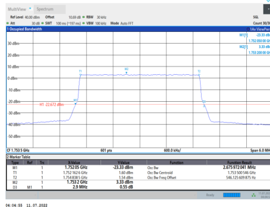
Band4-3MHz-16QAM-20385-15RB#0
