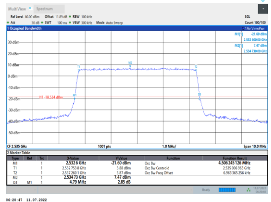
Band7-5MHz-16QAM-21100-25RB#0
