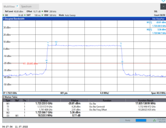
Band4-20MHz-QPSK-20175-100RB#0
