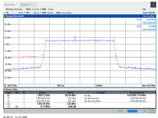
Band2-5MHz-16QAM-18625-25RB#0
