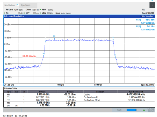
Band2-5MHz-16QAM-18900-25RB#0
