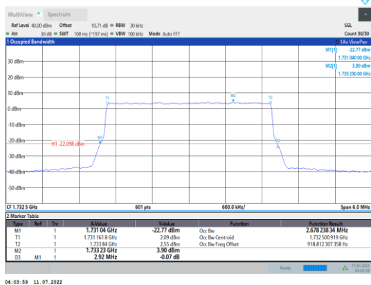
Band4-3MHz-QPSK-20175-15RB#0
