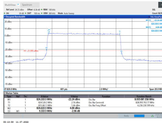
Band5-10MHz-16QAM-20450-50RB#0
