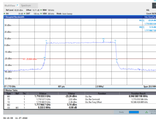
Band4-10MHz-16QAM-20000-50RB#0
