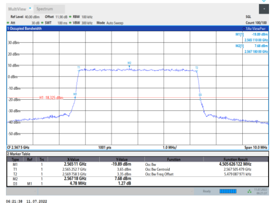
Band7-5MHz-16QAM-21425-25RB#0
