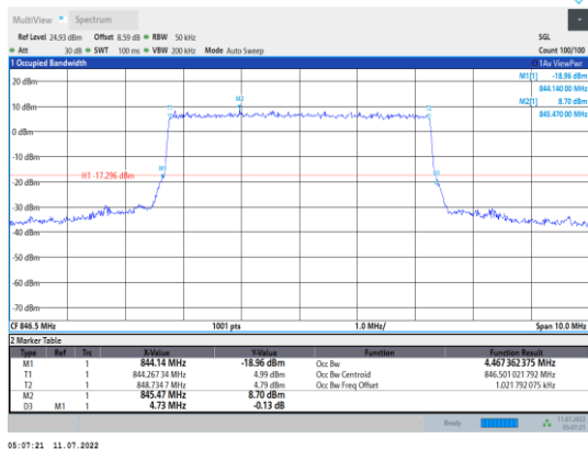
Band5-5MHz-QPSK-20625-25RB#0
