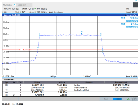
Band7-5MHz-QPSK-20775-25RB#0
