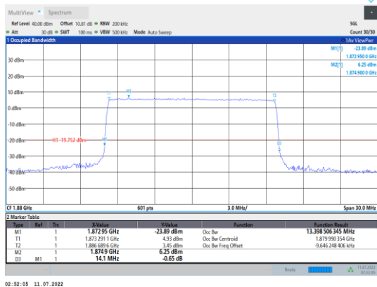
Band2-15MHz-QPSK-18900-75RB#0
