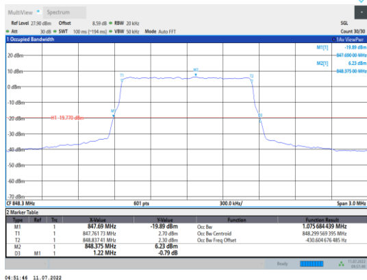
Band5-1.4MHz-QPSK-20643-6RB#0
