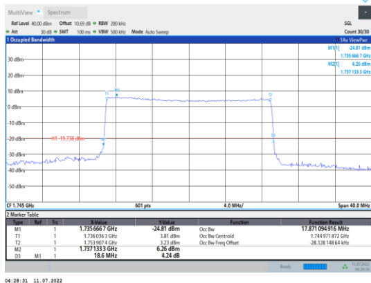
Band4-20MHz-QPSK-20300-100RB#0
