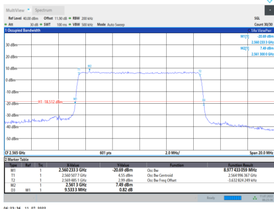
Band7-10MHz-QPSK-21400-50RB#0
