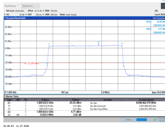
Band2-10MHz-16QAM-18650-50RB#0
