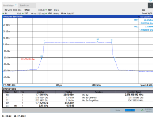
Band4-3MHz-QPSK-19965-15RB#0
