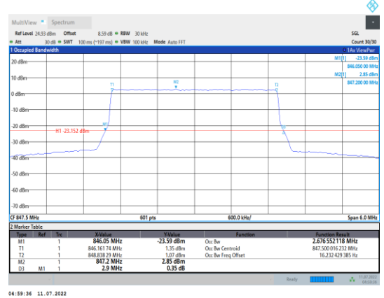
Band5-3MHz-16QAM-20635-15RB#0
