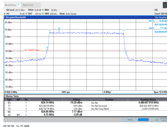
Band5-5MHz-16QAM-20425-25RB#0
