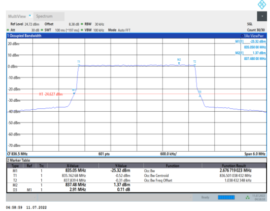
Band5-3MHz-16QAM-20525-15RB#0
