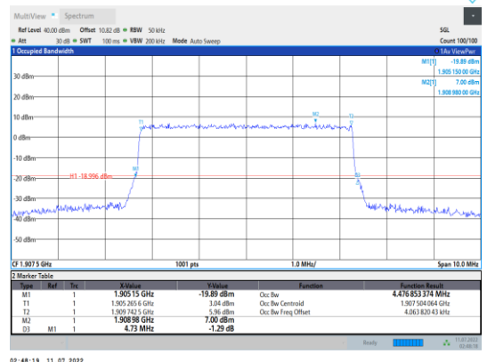
Band2-5MHz-16QAM-19175-25RB#0
