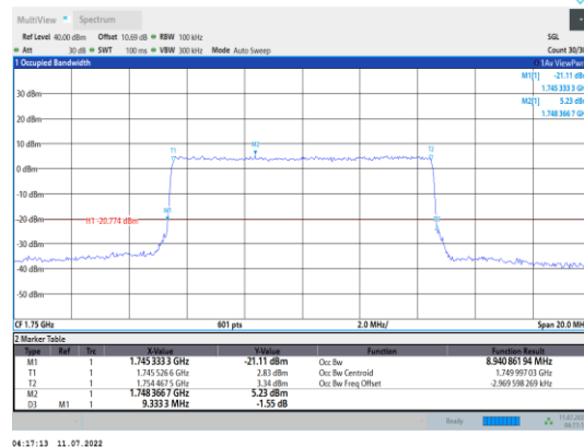
Band4-10MHz-16QAM-20350-50RB#0
