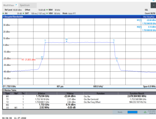
Band4-3MHz-QPSK-20385-15RB#0
