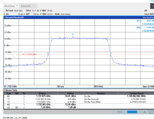
Band4-1.4MHz-16QAM-20175-6RB#0
