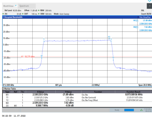
Band7-10MHz-QPSK-21100-50RB#0
