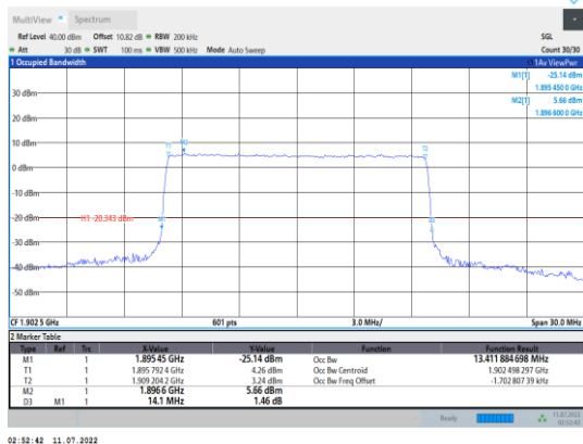
Band2-15MHz-QPSK-19125-75RB#0
