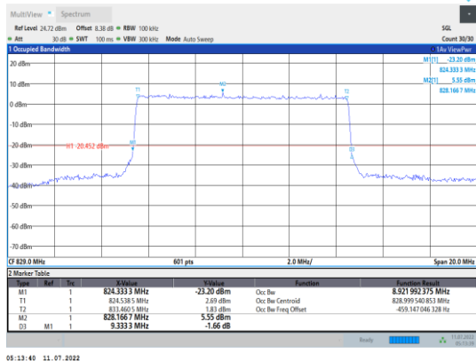
Band5-10MHz-QPSK-20450-50RB#0
