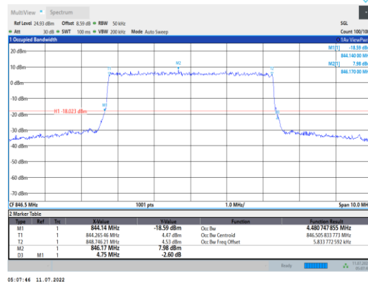
Band5-5MHz-16QAM-20625-25RB#0
