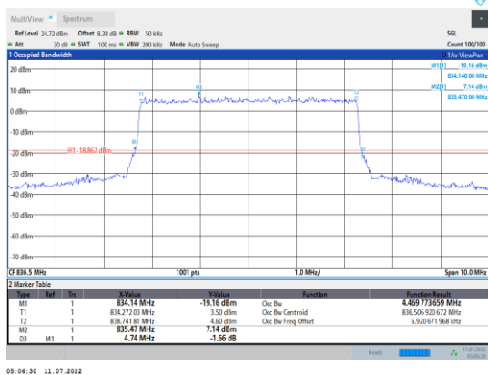
Band5-5MHz-QPSK-20525-25RB#0
