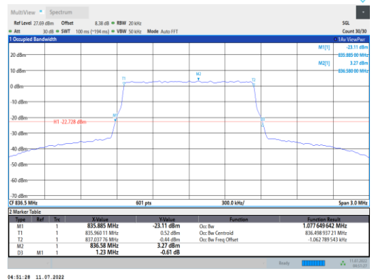
Band5-1.4MHz-16QAM-20525-6RB#0
