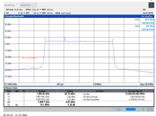
Band2-15MHz-16QAM-19125-75RB#0
