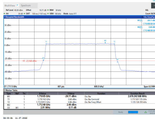
Band4-3MHz-16QAM-19965-15RB#0
