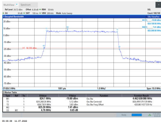
Band5-5MHz-QPSK-20425-25RB#0
