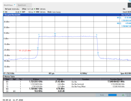
Band4-20MHz-16QAM-20175-100RB#0
