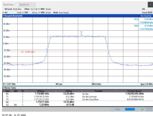
Band4-1.4MHz-QPSK-19957-6RB#0
