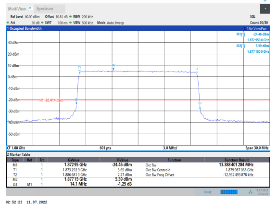
Band2-15MHz-16QAM-18900-75RB#0
