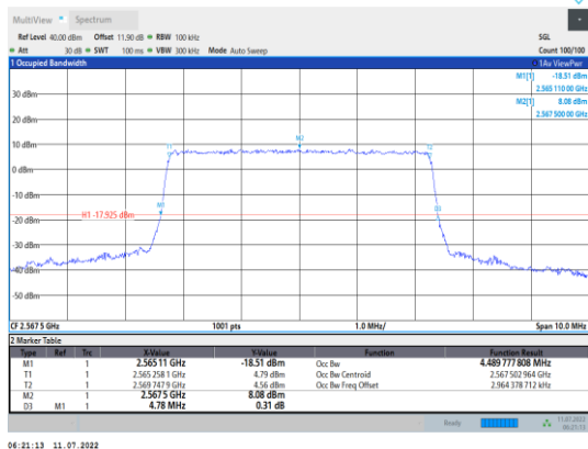
Band7-5MHz-QPSK-21425-25RB#0
