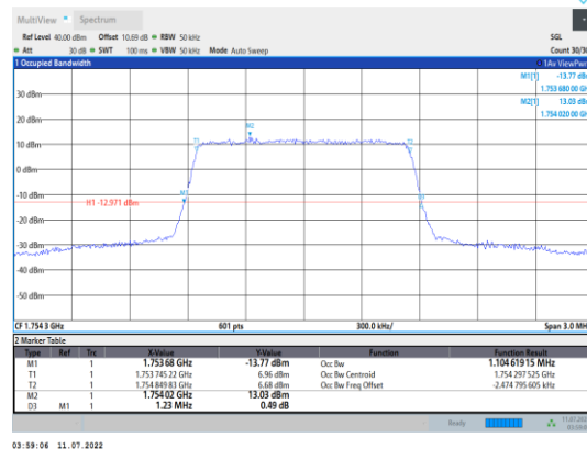
Band4-1.4MHz-16QAM-20393-6RB#0
