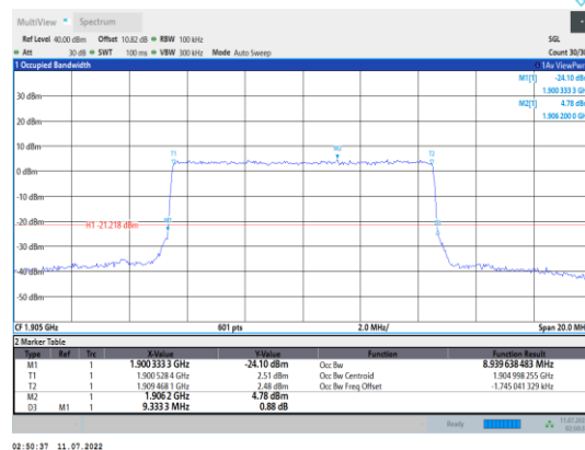
Band2-10MHz-16QAM-19150-50RB#0
