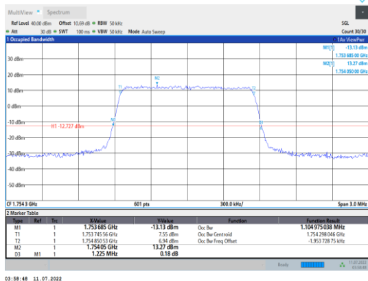
Band4-1.4MHz-QPSK-20393-6RB#0
