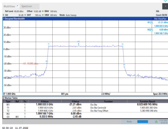
Band2-10MHz-QPSK-19150-50RB#0
