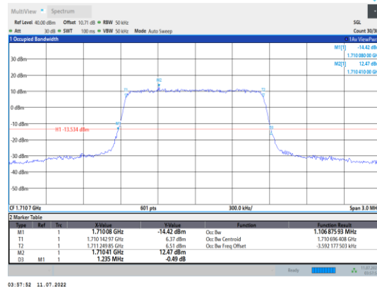
Band4-1.4MHz-16QAM-19957-6RB#0
