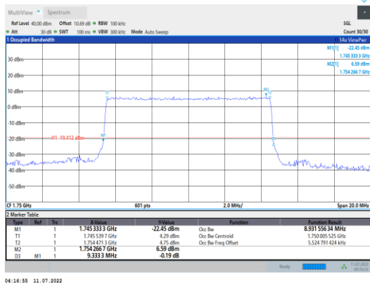
Band4-10MHz-QPSK-20350-50RB#0
