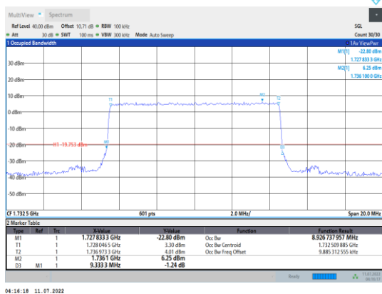
Band4-10MHz-QPSK-20175-50RB#0
