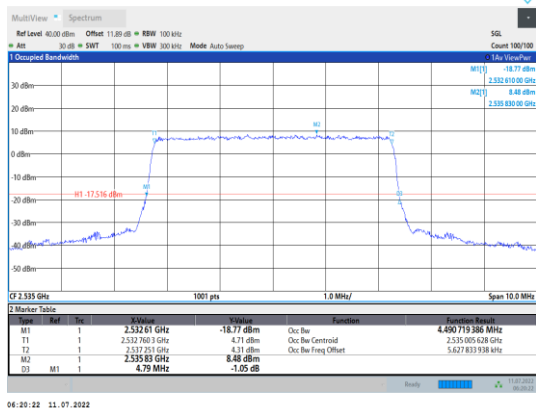
Band7-5MHz-QPSK-21100-25RB#0
