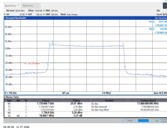
Band4-20MHz-16QAM-20300-100RB#0
