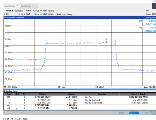
Band4-10MHz-16QAM-20175-50RB#0
