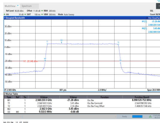
Band7-10MHz-16QAM-21400-50RB#0
