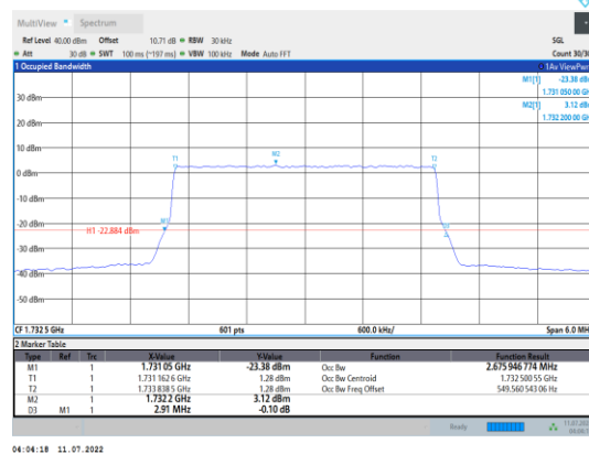
Band4-3MHz-16QAM-20175-15RB#0
