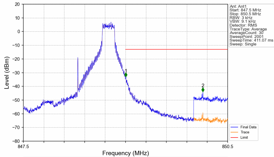
Band5_1.4MHz_QPSK_HCH_848.3MHz_RB_1_5_NTNV
