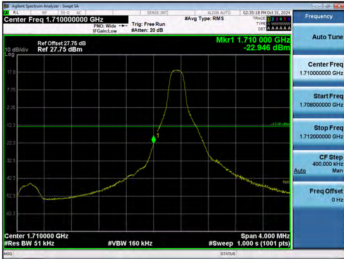
LTE B66_5 M_Band Edge_Low_QPSK_1RB
