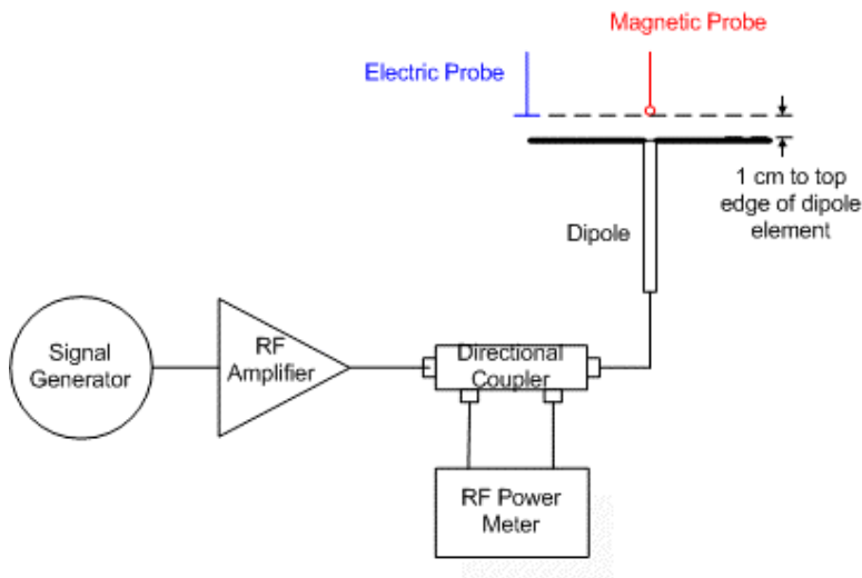
Figure 7.3 Probe Modulation Setup
