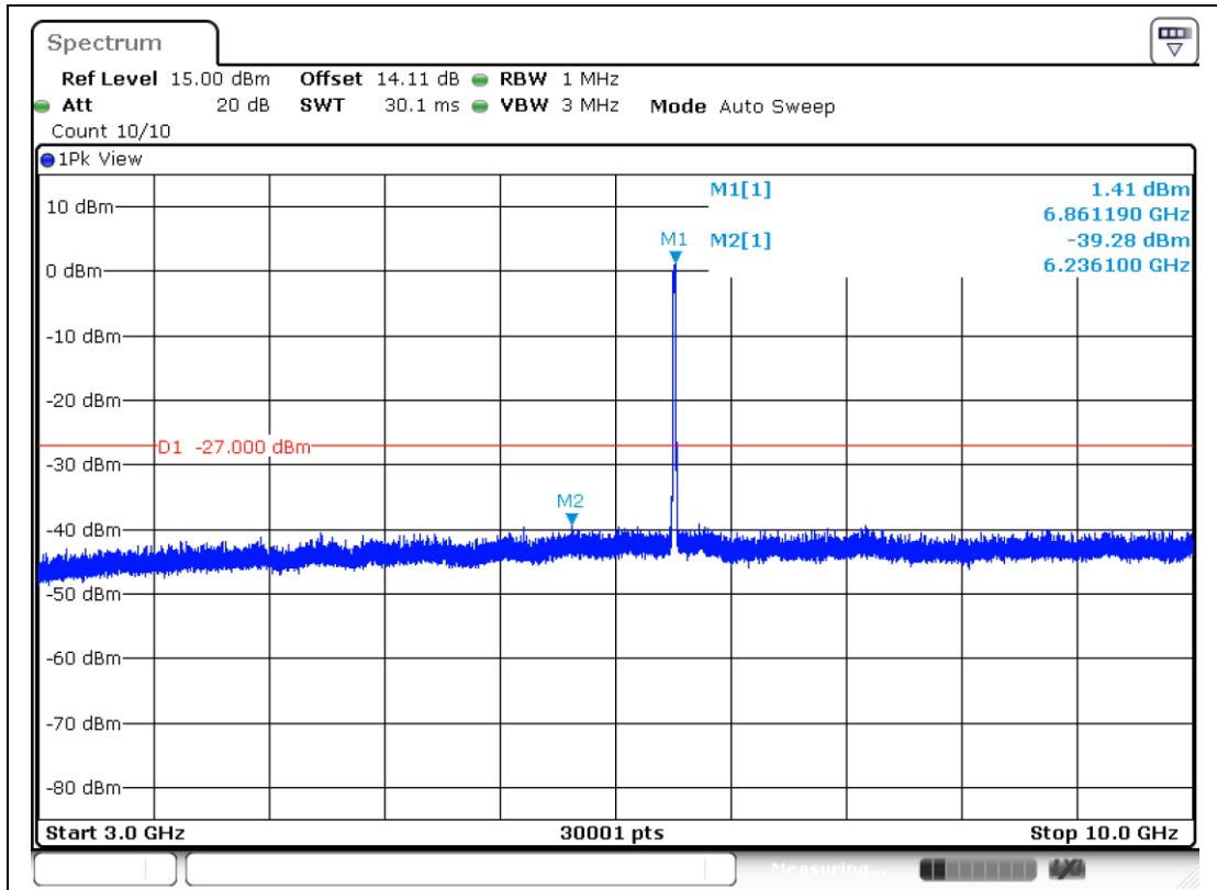
11AX20MIMO-Ant2-6855-3000~10000-PASS
