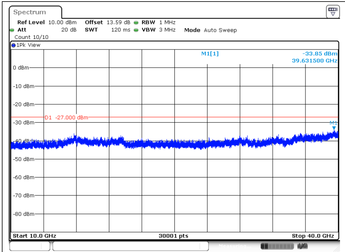
11AX20MIMO-Ant2-6535-10000~40000-PASS
