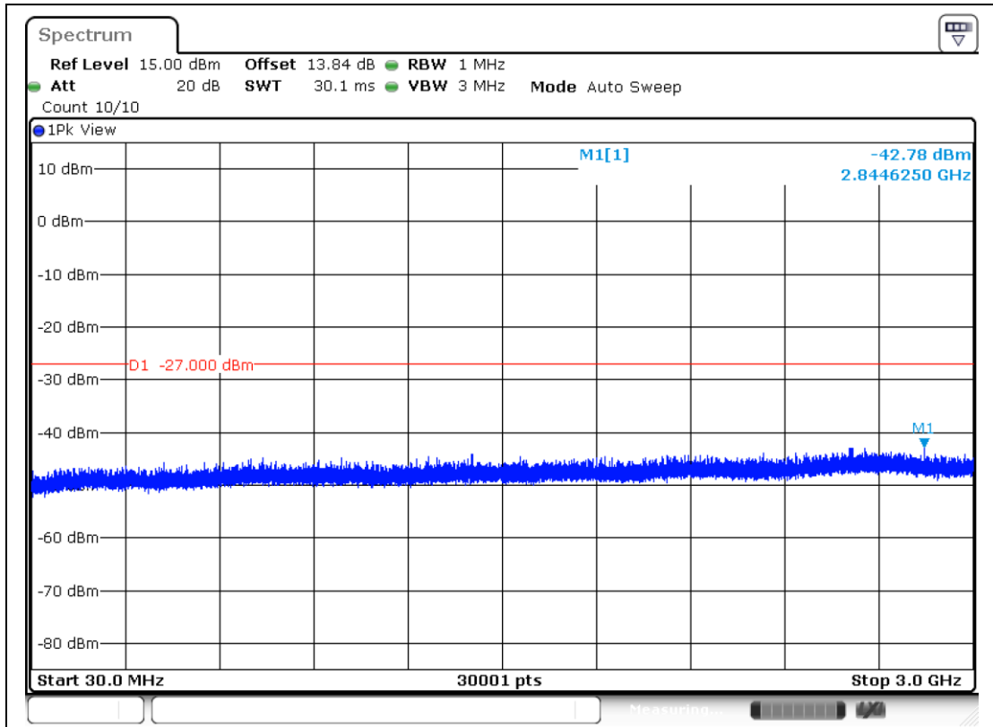
11AX20MIMO-Ant2-6995-30~3000-PASS
