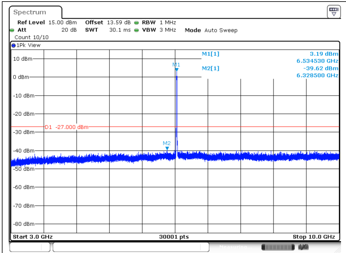
11AX20MIMO-Ant2-6535-3000~10000-PASS
