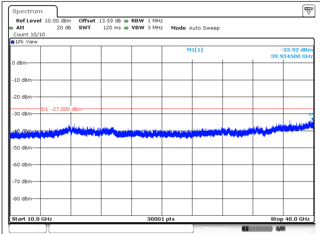
11AX20MIMO-Ant2-6515-10000~40000-PASS
