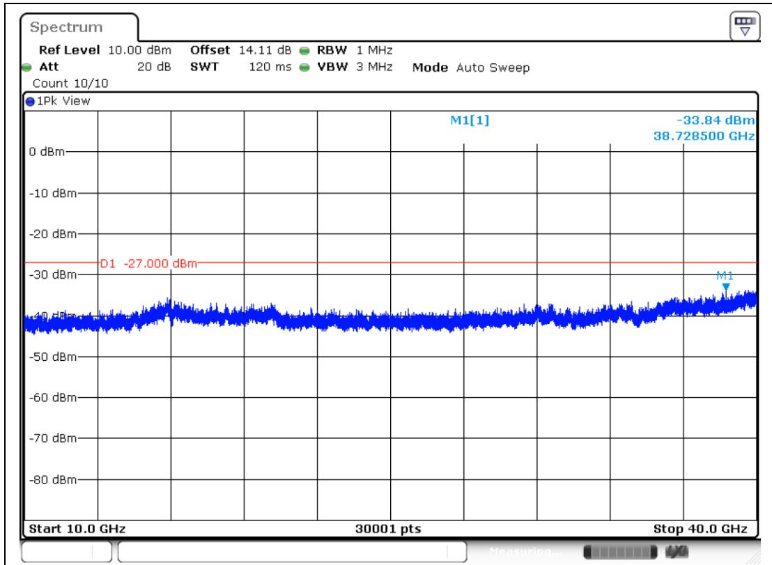
11AX20MIMO-Ant2-6895-10000~40000-PASS
