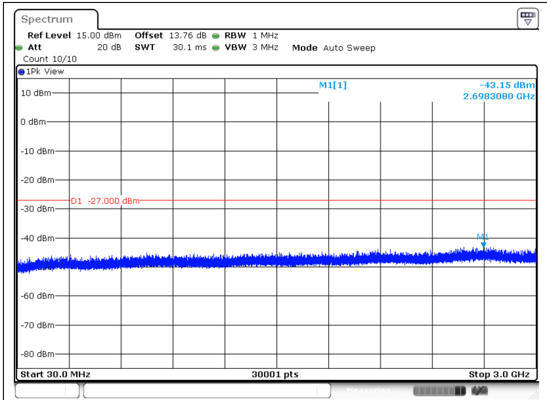
11AX20MIMO-Ant2-6475-30~3000-PASS
