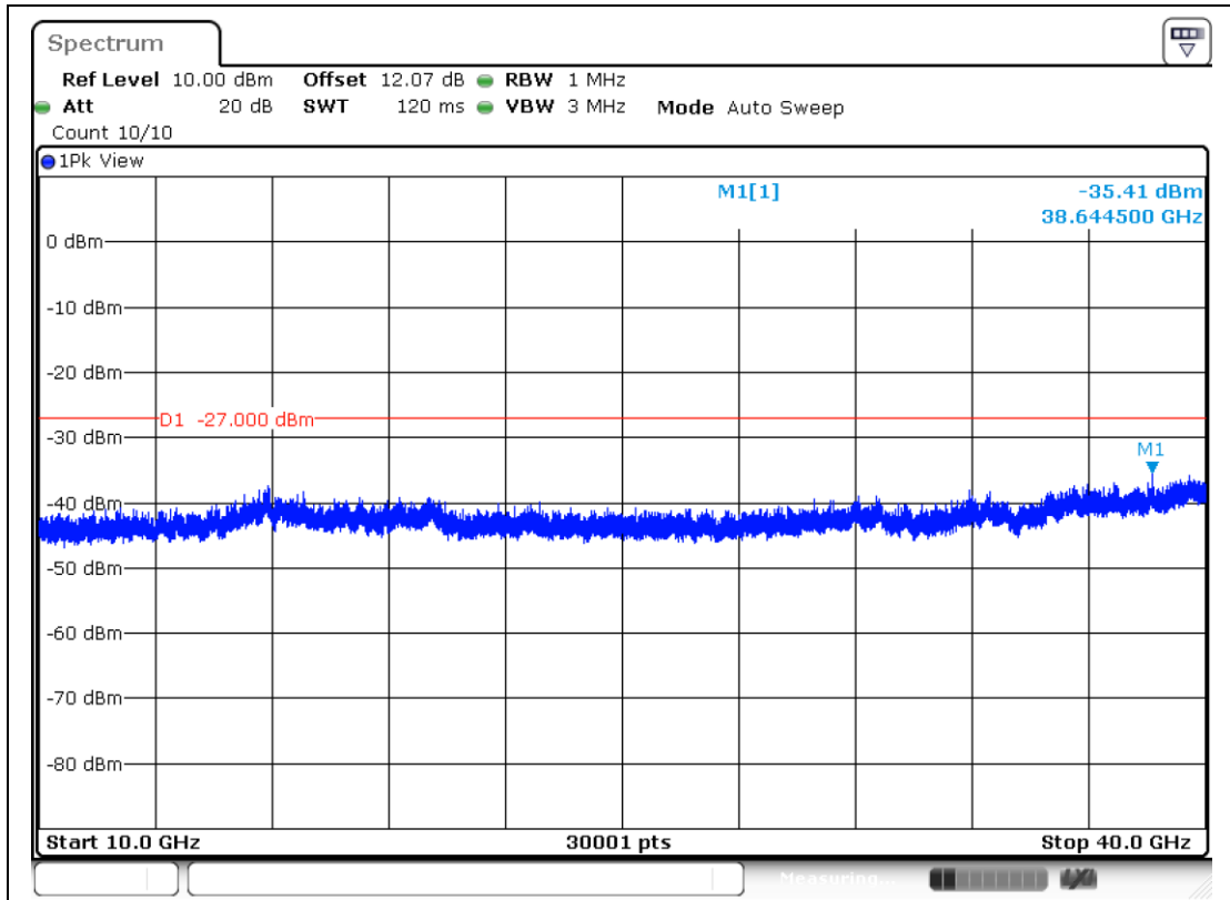
11AX20MIMO-Ant1-6175-10000~40000-PASS
