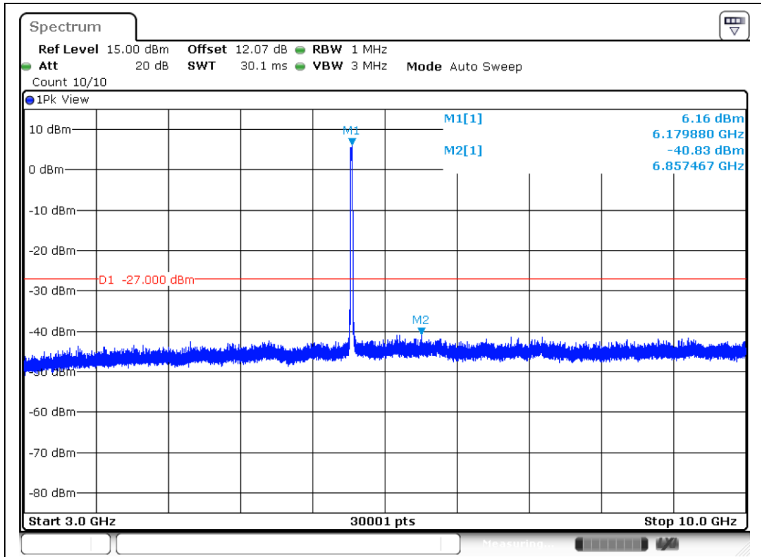
11AX20MIMO-Ant1-6175-3000~10000-PASS
