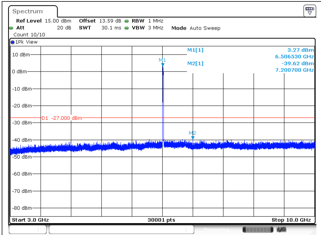
11AX20MIMO-Ant2-6515-3000~10000-PASS
