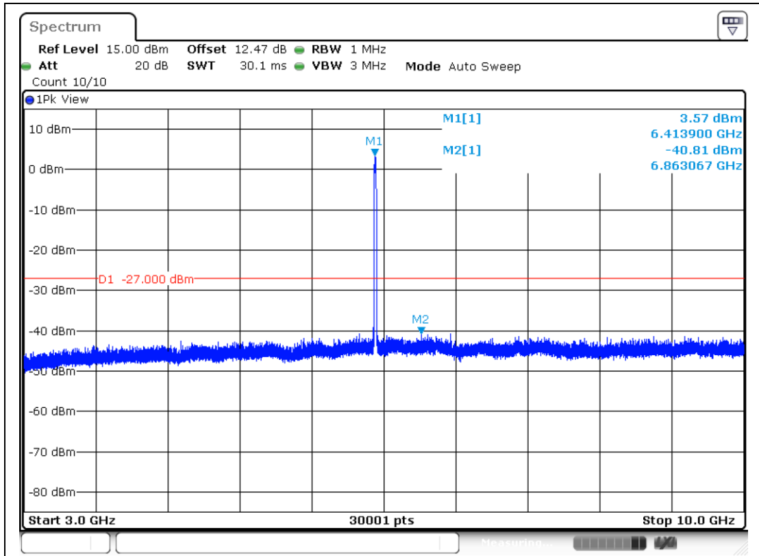
11AX20MIMO-Ant1-6415-3000~10000-PASS
