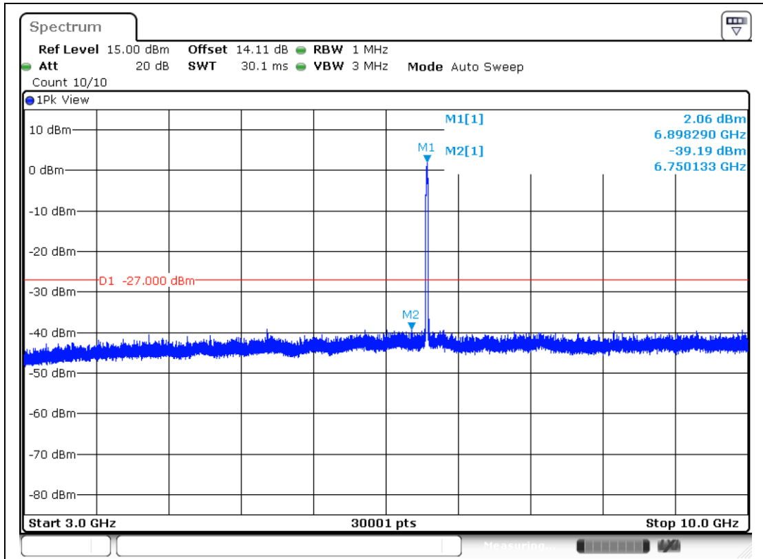
11AX20MIMO-Ant2-6895-3000~10000-PASS
