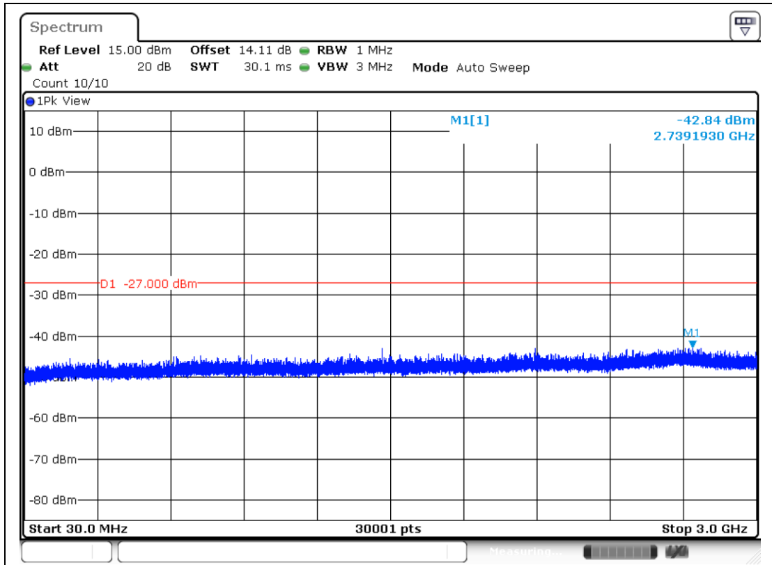
11AX20MIMO-Ant2-6875-30~3000-PASS
