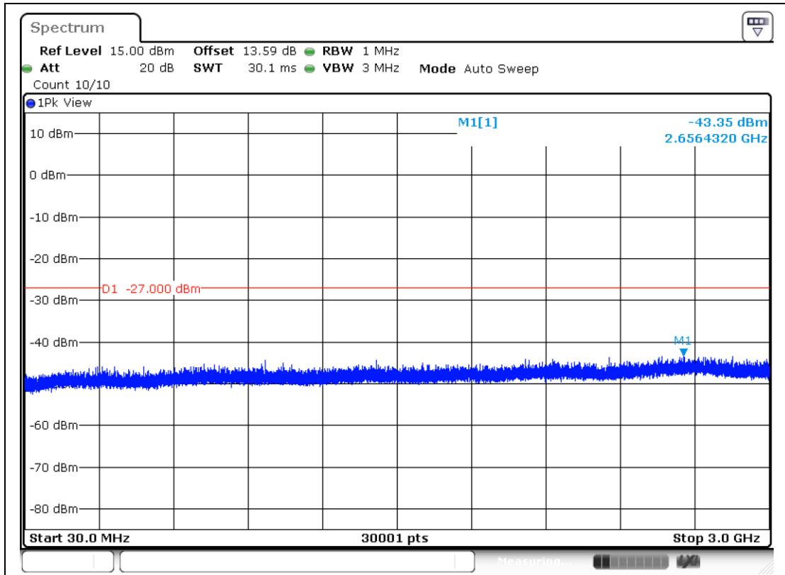
11AX20MIMO-Ant2-6515-30~3000-PASS
