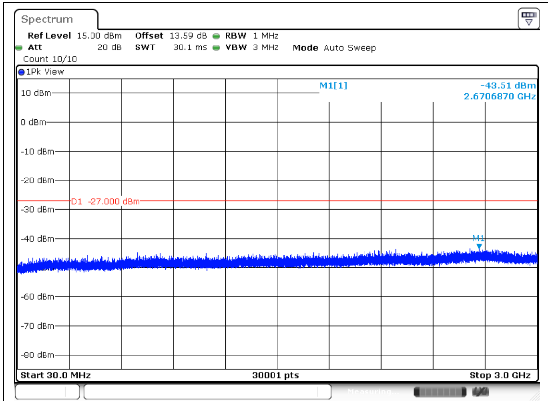
11AX20MIMO-Ant2-6695-30~3000-PASS
