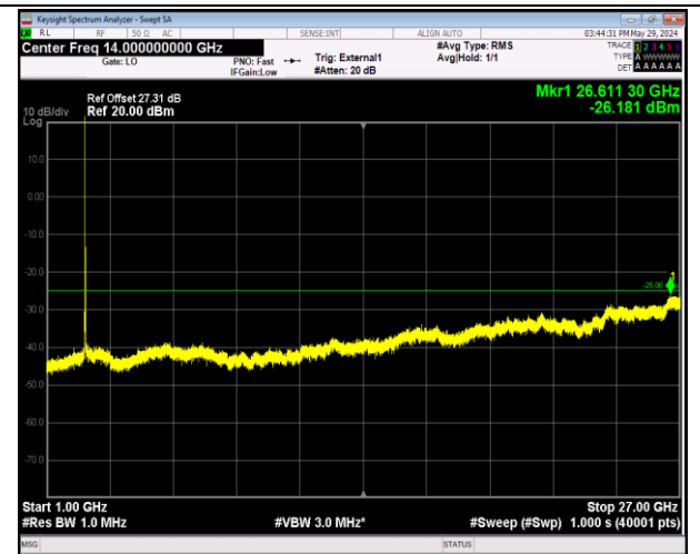
Band38_20MHz_64QAM_37850_1RB#0_1000~27000_10 00~27000
