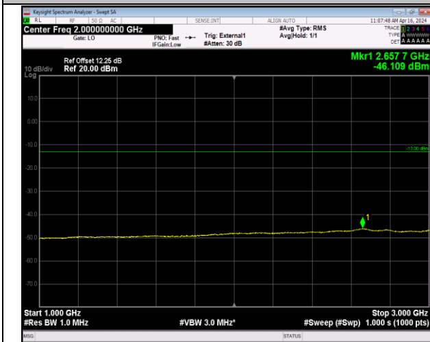
Band42_5MHz_16QAM_42115_1RB#0_1000~3000_1000~3000
