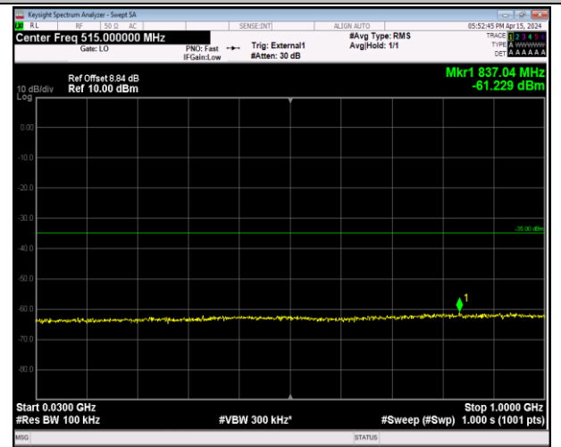
Band41_20MHz_64QAM_39750_1RB#0_30~1000_30~10 00
