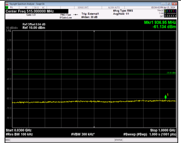
Band41_20MHz_16QAM_40620_1RB#0_30~1000_30~10 00
