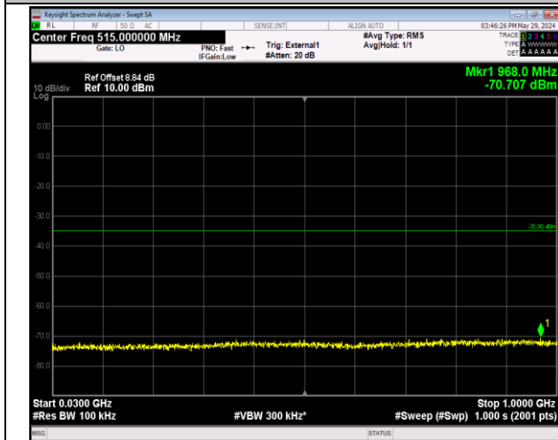
Band38_20MHz_64QAM_38000_1RB#0_30~1000_30~10 00
