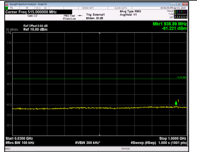
Band41_5MHz_16QAM_41565_1RB#0_30~1000_30~100 0
