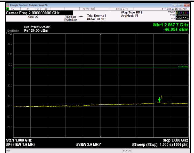
Band42_5MHz_16QAM_42590_1RB#0_1000~3000_1000~3000
