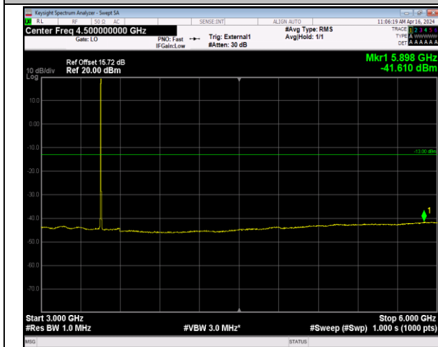
Band42_5MHz_QPSK_42115_1RB#0_3000~6000_3000~6000
