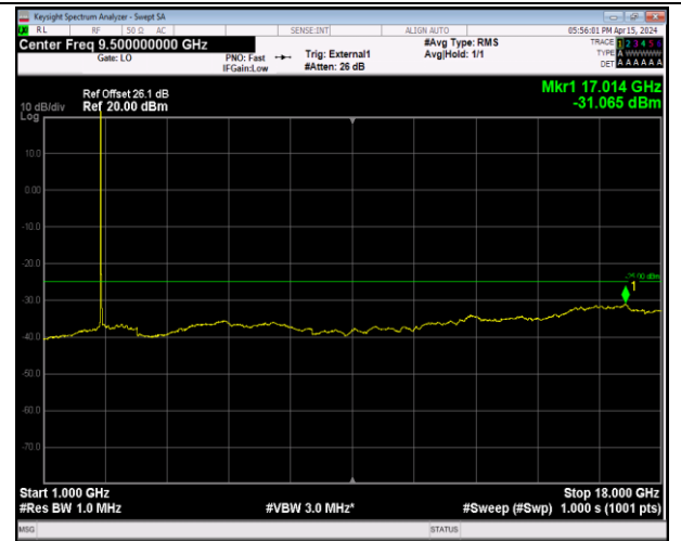
Band41_20MHz_64QAM_40620_1RB#0_1000~18000_10 00~18000
