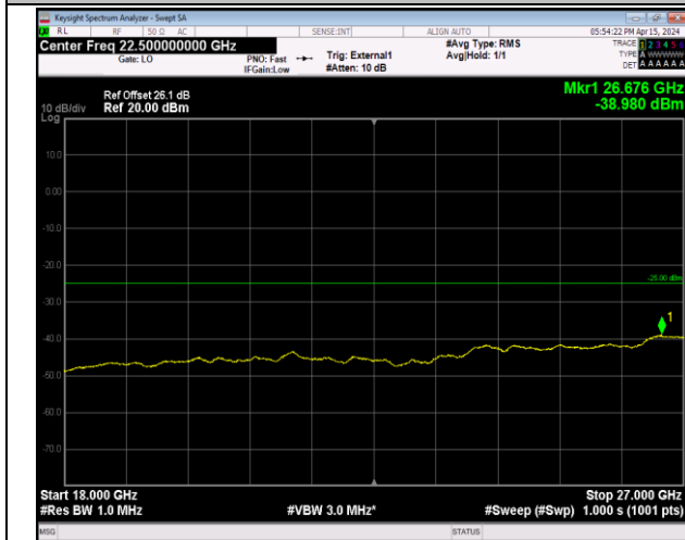
Band41_20MHz_QPSK_40620_1RB#0_18000~27000_18 000~27000
