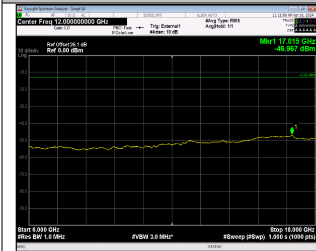
Band42_5MHz_16QAM_43065_1RB#0_6000~18000_6000~18000
