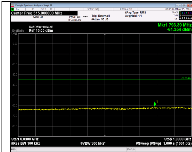
Band41_20MHz_QPSK_40620_1RB#0_30~1000_30~100 0
