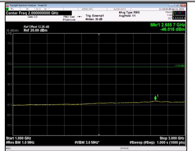
Band42_5MHz_QPSK_43065_1RB#0_1000~3000_1000~3000
