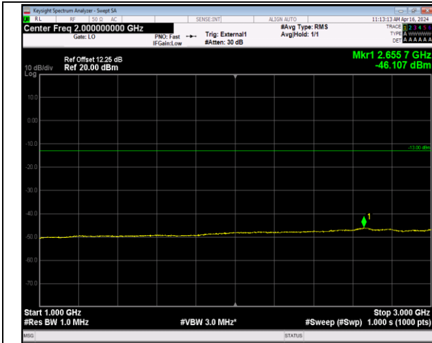
Band42_5MHz_QPSK_42590_1RB#0_1000~3000_1000~3000
