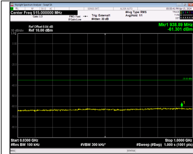
Band41_20MHz_64QAM_40620_1RB#0_30~1000_30~10 00
