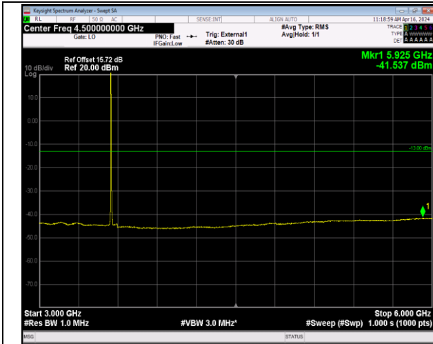
Band42_5MHz_QPSK_43065_1RB#0_3000~6000_3000~6000
