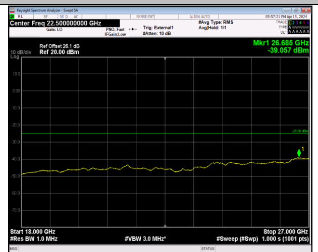
Band41_20MHz_QPSK_41490_1RB#0_18000~27000_18 000~27000
