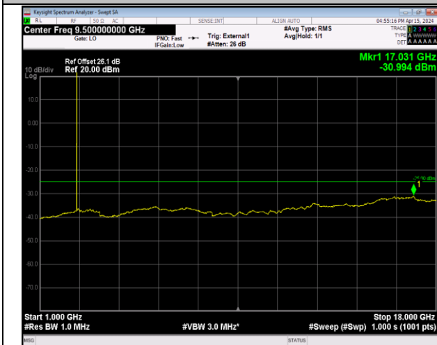
Band41_5MHz_64QAM_40620_1RB#0_1000~18000_100 0~18000
