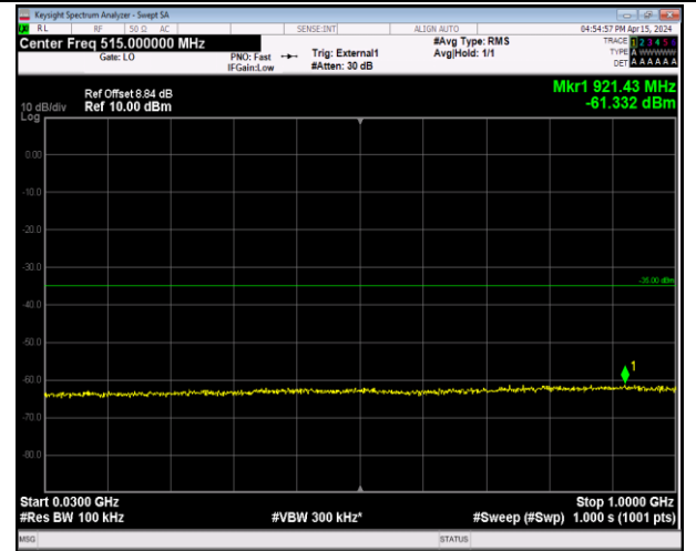
Band41_5MHz_64QAM_40620_1RB#0_30~1000_30~100 0
