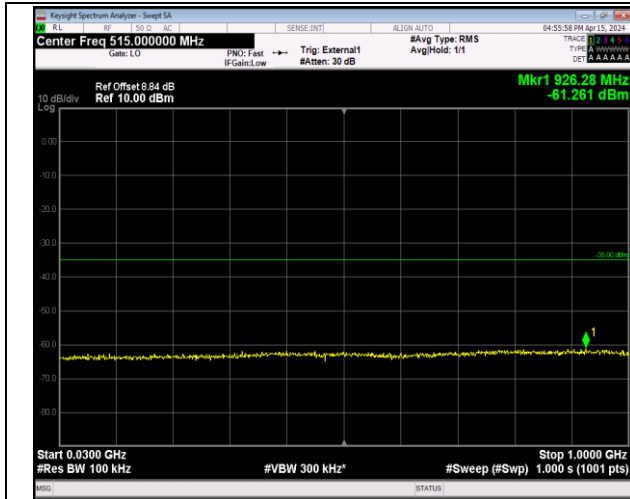
Band41_5MHz_QPSK_41565_1RB#0_30~1000_30~1000
