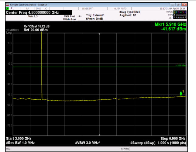
Band42_5MHz_QPSK_42590_1RB#0_3000~6000_3000~6000
