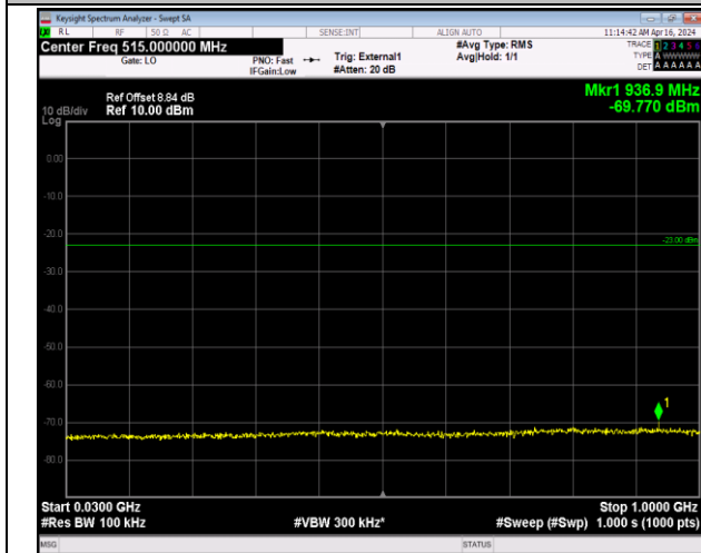
Band42_5MHz_16QAM_42590_1RB#0_30~1000_30~1000
