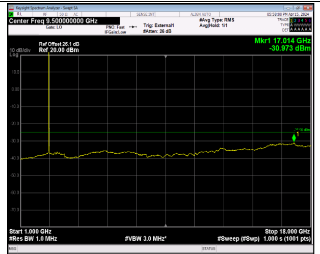
Band41_20MHz_16QAM_41490_1RB#0_1000~18000_10 00~18000
