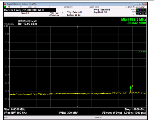
Band42_5MHz_16QAM_42115_1RB#0_30~1000_30~1000
