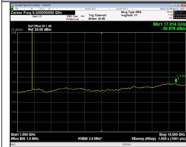
Band41_5MHz_16QAM_39675_1RB#0_1000~18000_1000~18000
