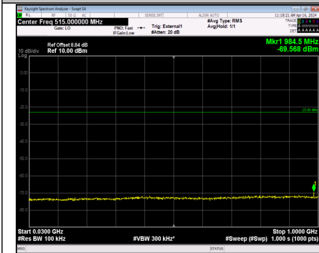
Band42_5MHz_QPSK_43065_1RB#0_30~1000_30~1000
