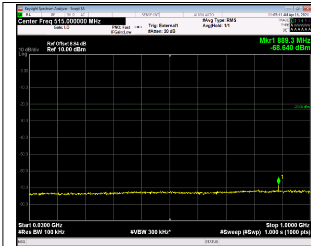
Band42_5MHz_QPSK_42115_1RB#0_30~1000_30~1000
