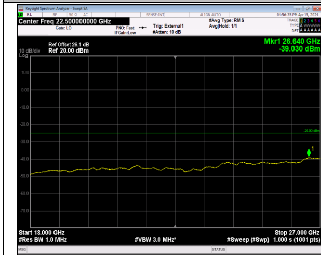
Band41_5MHz_QPSK_41565_1RB#0_18000~27000_18000~27000
