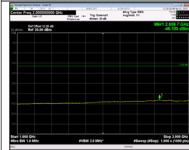
Band42_5MHz_16QAM_43065_1RB#0_1000~3000_1000~3000
