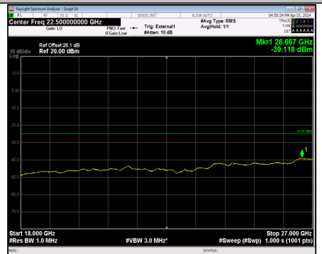
Band41_5MHz_64QAM_40620_1RB#0_18000~27000_18 000~27000
