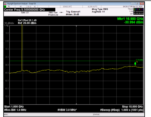
Band41_5MHz_16QAM_40620_1RB#0_1000~18000_100 0~18000
