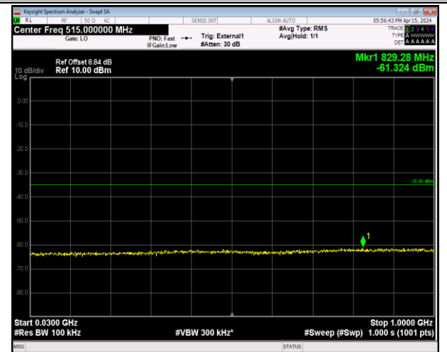
Band41_20MHz_QPSK_41490_1RB#0_30~1000_30~100 0
