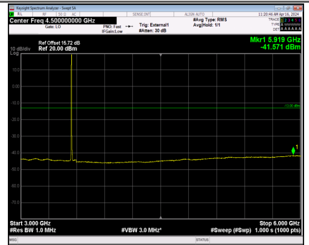
Band42_5MHz_16QAM_43065_1RB#0_3000~6000_3000~6000
