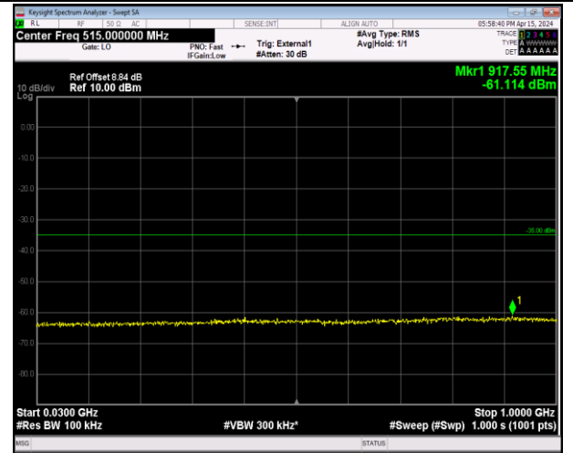
Band41_20MHz_64QAM_41490_1RB#0_30~1000_30~10 00
