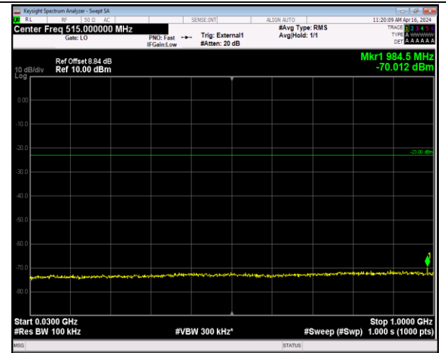
Band42_5MHz_16QAM_43065_1RB#0_30~1000_30~1000
