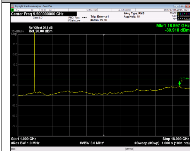
Band41_20MHz_QPSK_41490_1RB#0_1000~18000_100 0~18000
