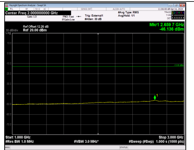
Band42_5MHz_QPSK_42115_1RB#0_1000~3000_1000~3000
