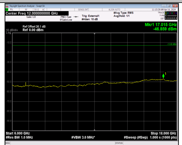
Band42_5MHz_16QAM_42590_1RB#0_6000~18000_6000~18000
