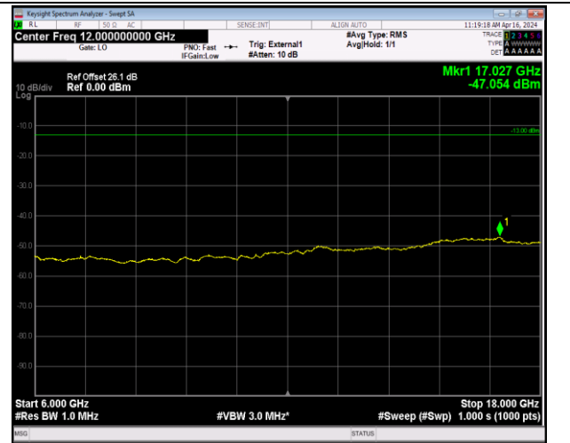
Band42_5MHz_QPSK_43065_1RB#0_6000~18000_6000~18000
