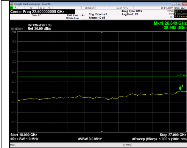
Band41_20MHz_64QAM_40620_1RB#0_18000~27000_1 8000~27000
