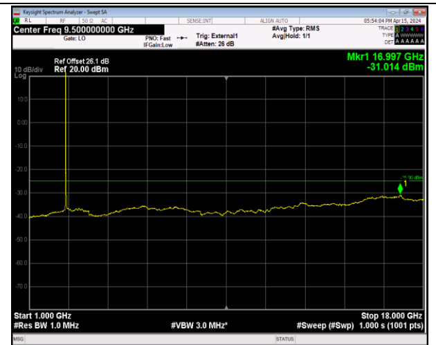
Band41_20MHz_QPSK_40620_1RB#0_1000~18000_100 0~18000
