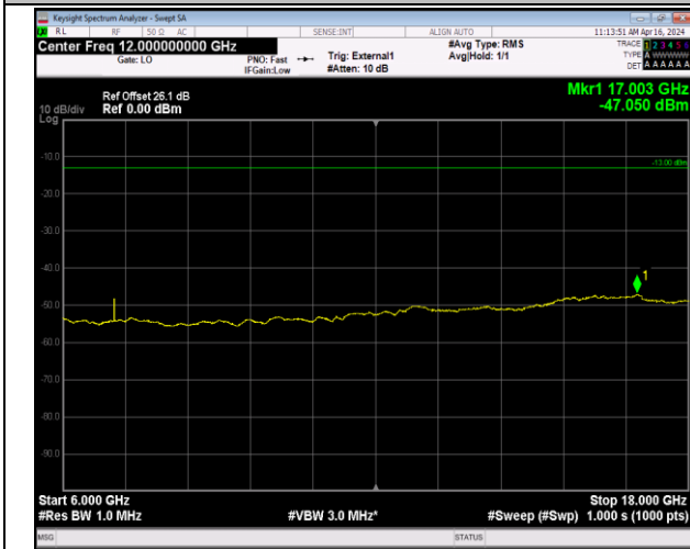
Band42_5MHz_QPSK_42590_1RB#0_6000~18000_6000~18000
