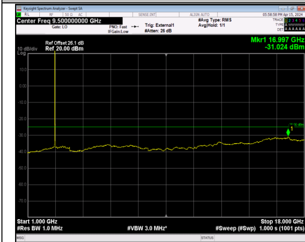
Band41_20MHz_64QAM_41490_1RB#0_1000~18000_10 00~18000
