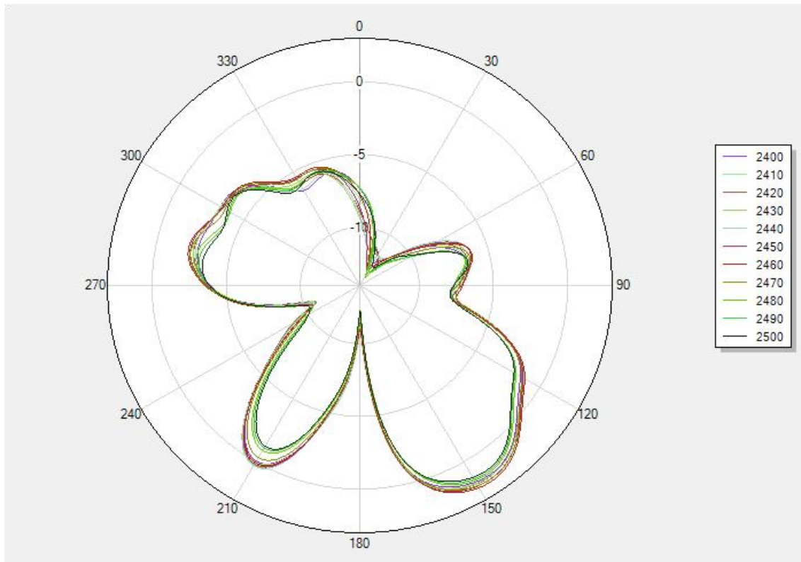
Phi 0 2D
