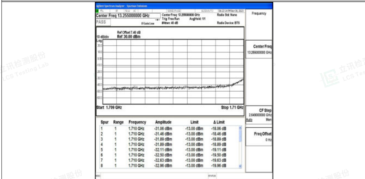
Band4_3MHz_16QAM_19965_15RB#0
