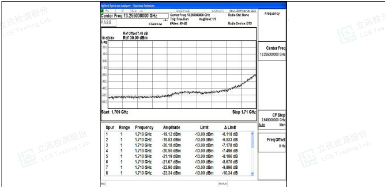
Band4_3MHz_64QAM_19965_1RB#0
