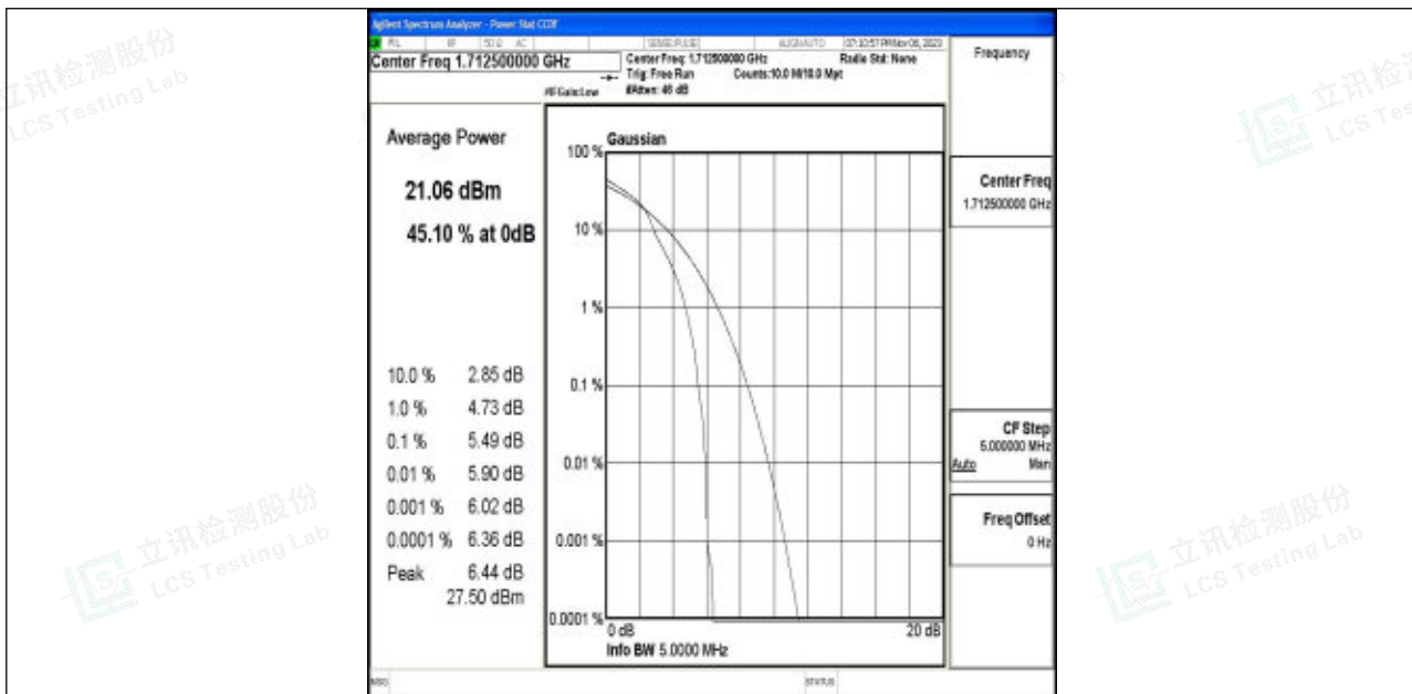
Band4-5MHz-16QAM-19975-1RB#0-PASS
