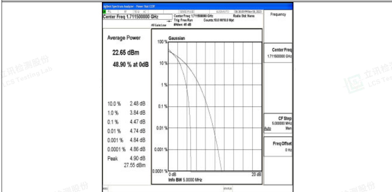
Band4-3MHz-QPSK-19965-1RB#0-PASS
