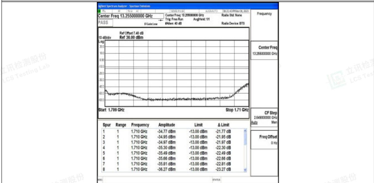
Band4_3MHz_QPSK_19965_1RB#14
