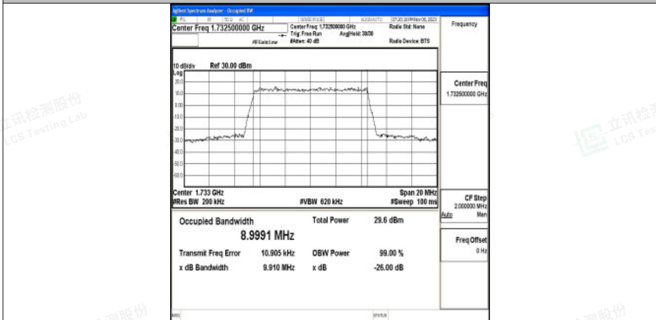
Band4-10MHz-16QAM-20175-50RB#0-PASS
