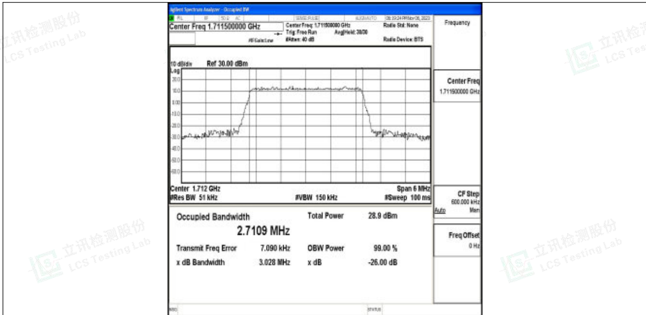
Band4-3MHz-16QAM-19965-15RB#0-PASS
