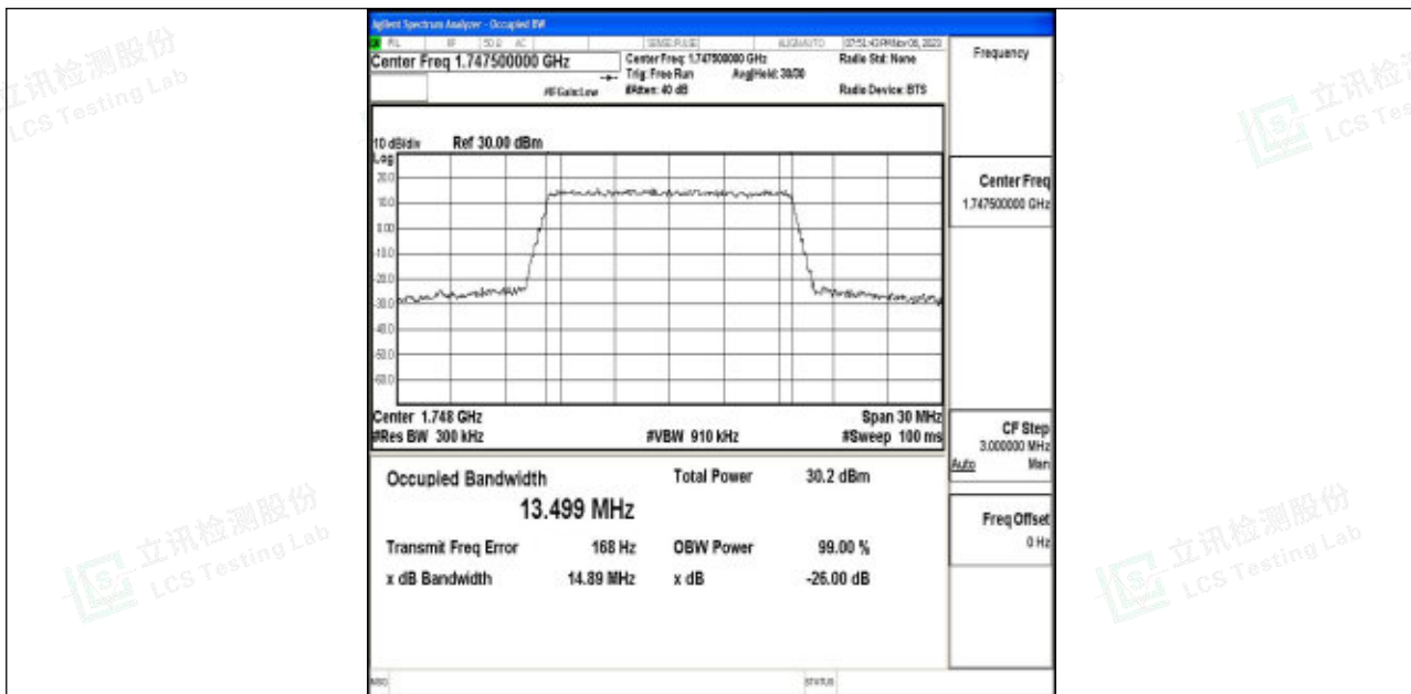
Band4-15MHz-QPSK-20325-75RB#0-PASS
