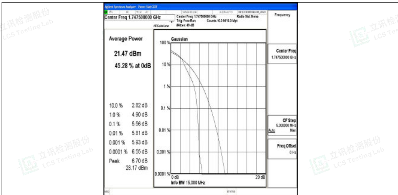
Band4-15MHz-16QAM-20325-1RB#0-PASS
