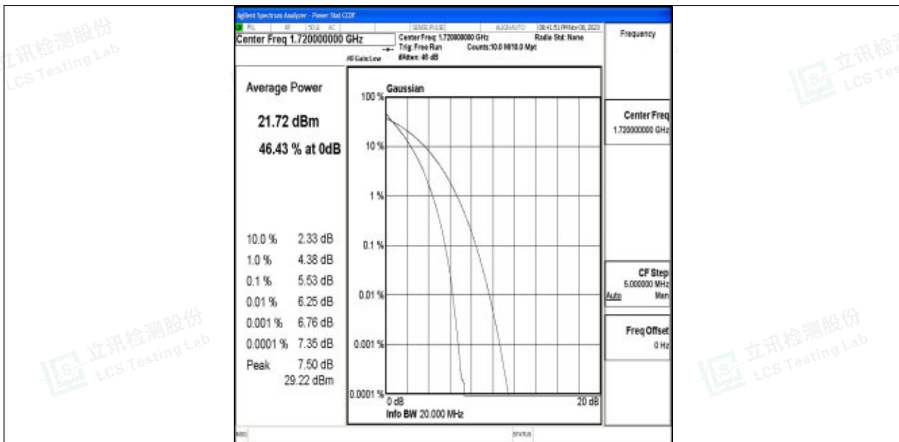
Band4-20MHz-64QAM-20050-100RB#0-PASS
