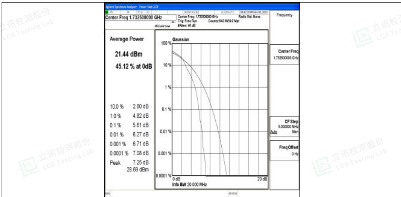
Band4-20MHz-16QAM-20175-1RB#0-PASS
