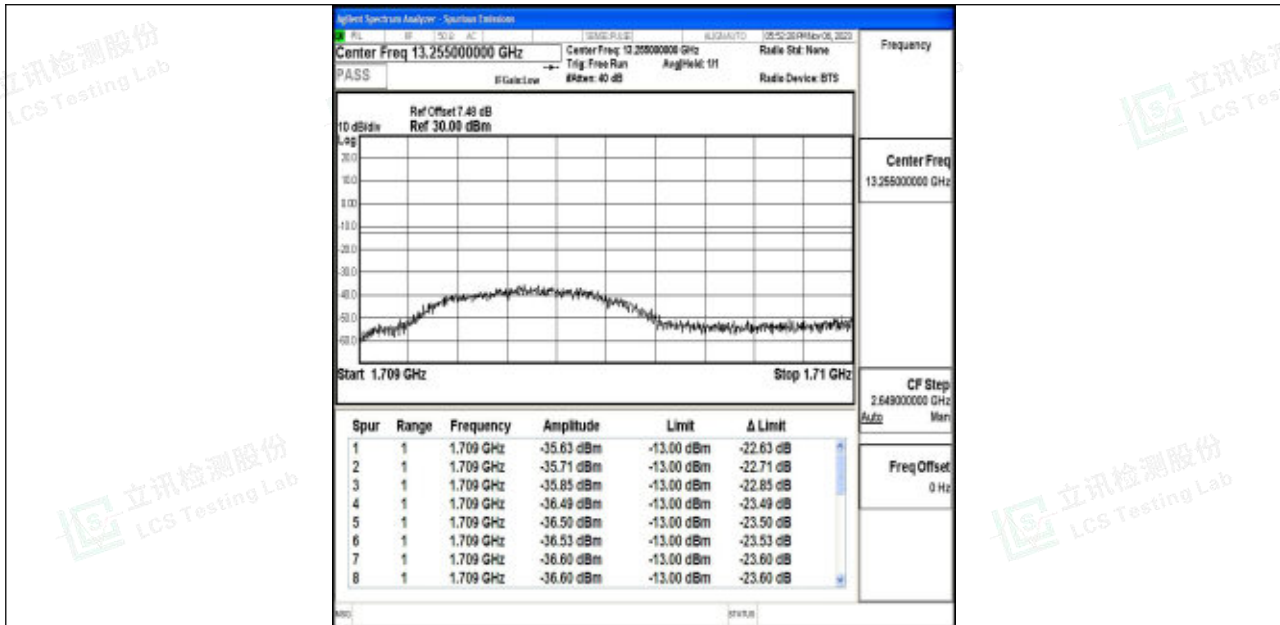
Band4_1.4MHz_16QAM_19957_1RB#5
