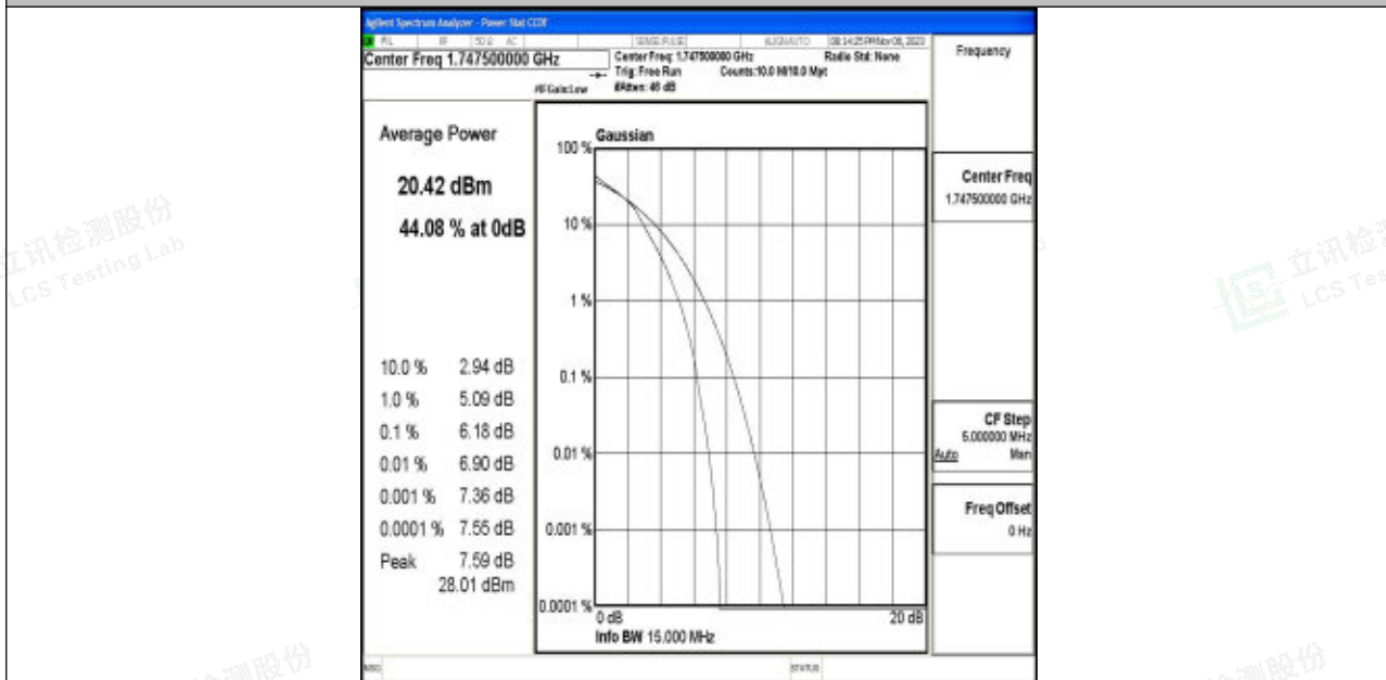
Band4-15MHz-16QAM-20325-75RB#0-PASS
