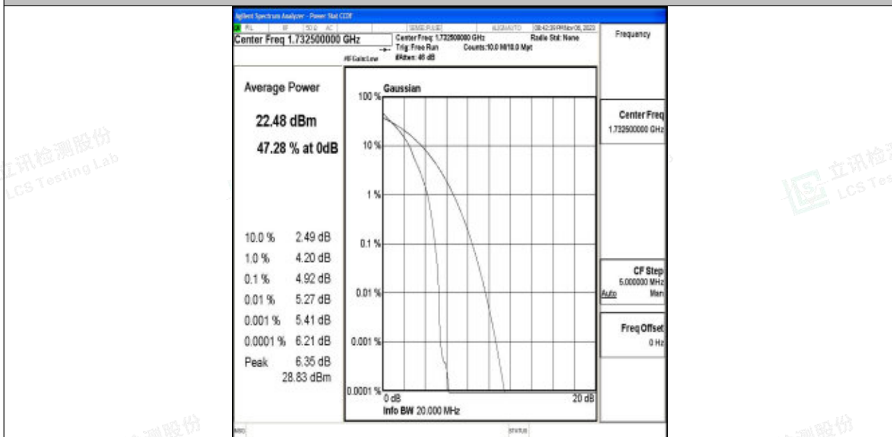
Band4-20MHz-64QAM-20175-1RB#0-PASS
