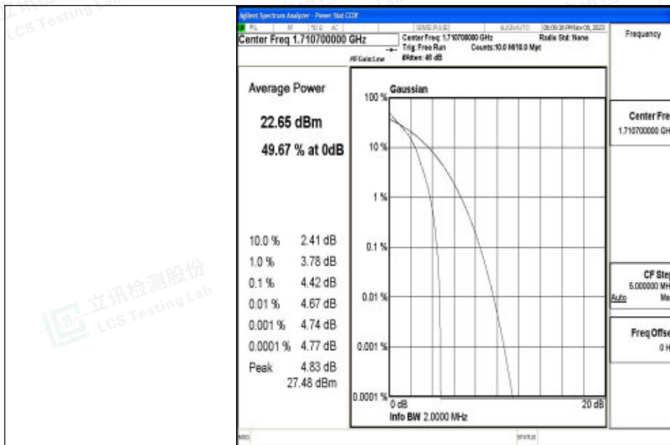
Band4-1.4MHz-QPSK-19957-1RB#0-PASS
