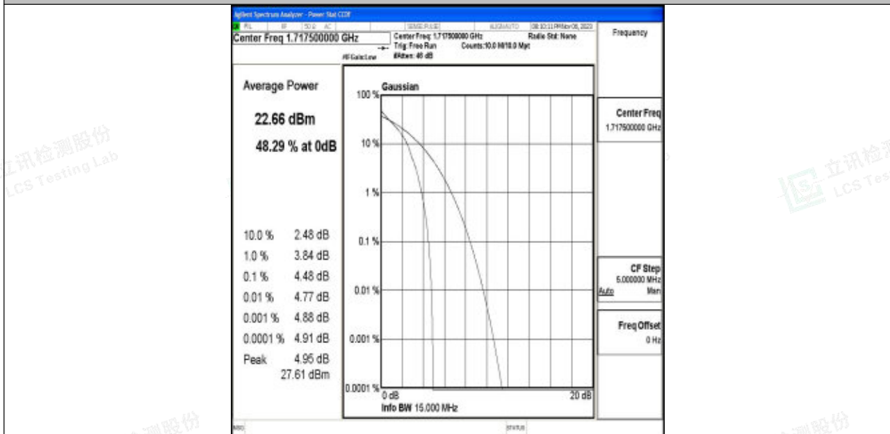
Band4-15MHz-64QAM-20025-1RB#0-PASS
