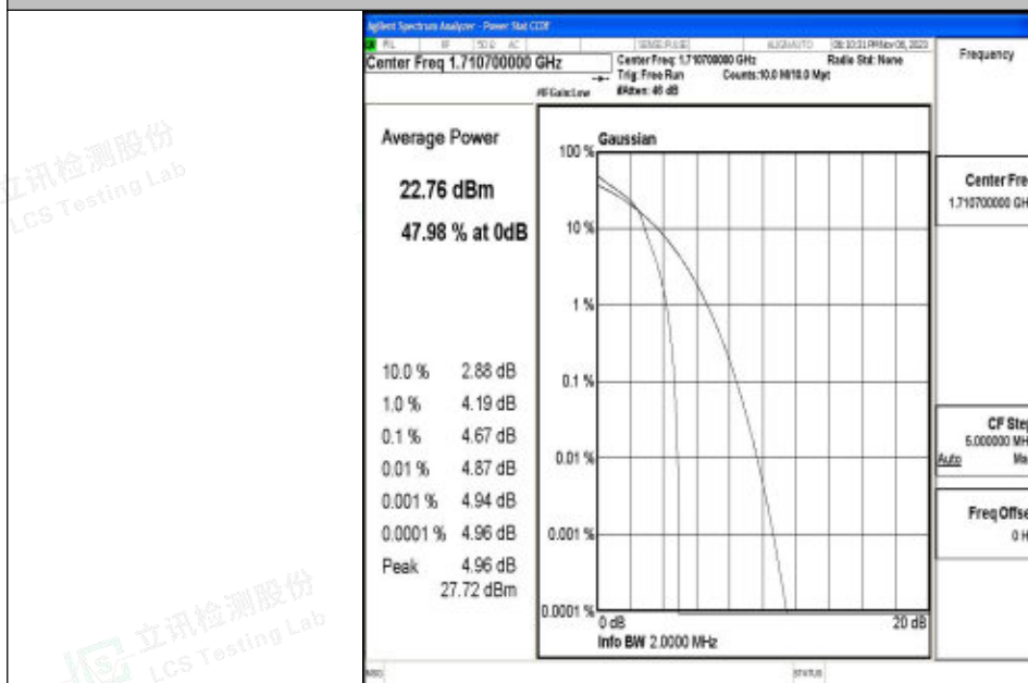
Band4-1.4MHz-16QAM-19957-1RB#0-PASS
