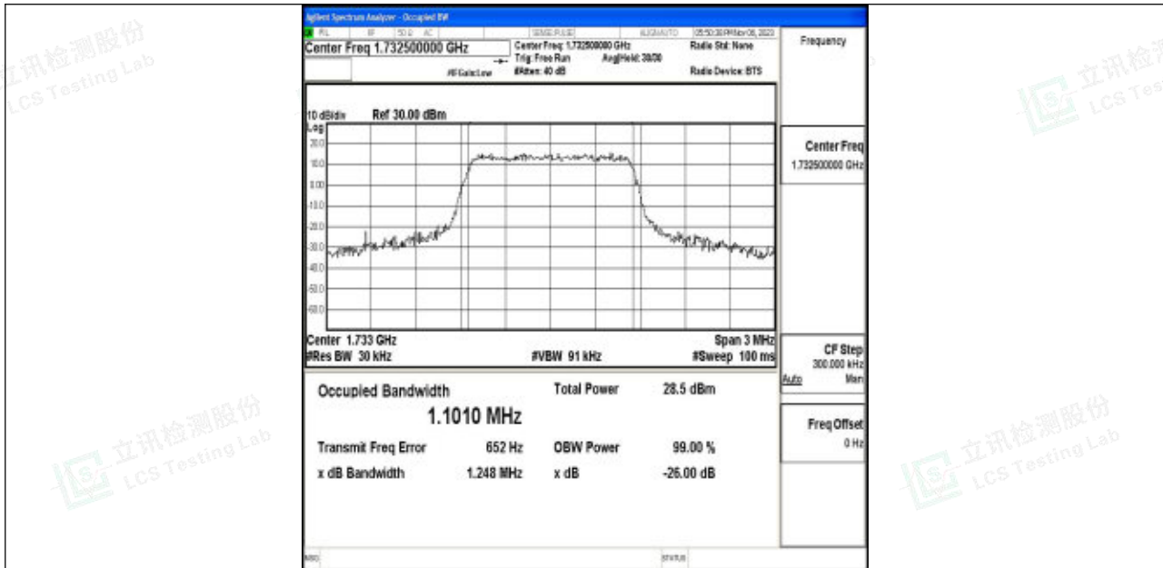
Band4-1.4MHz-16QAM-20175-6RB#0-PASS
