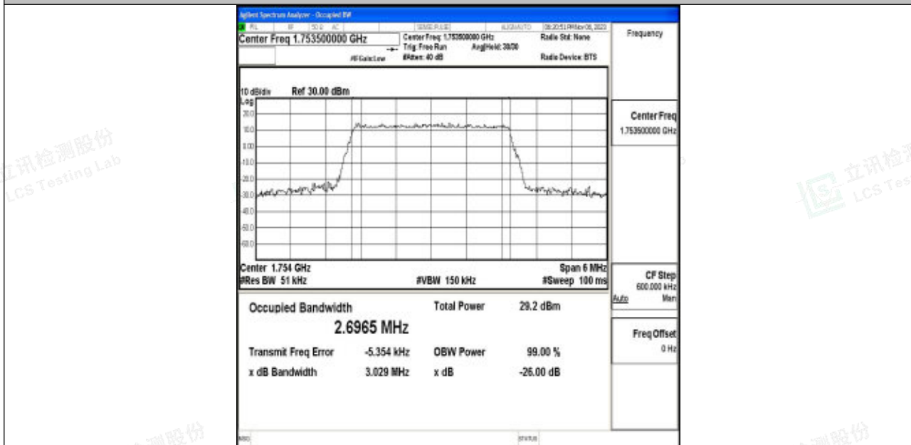
Band4-3MHz-64QAM-20385-15RB#0-PASS
