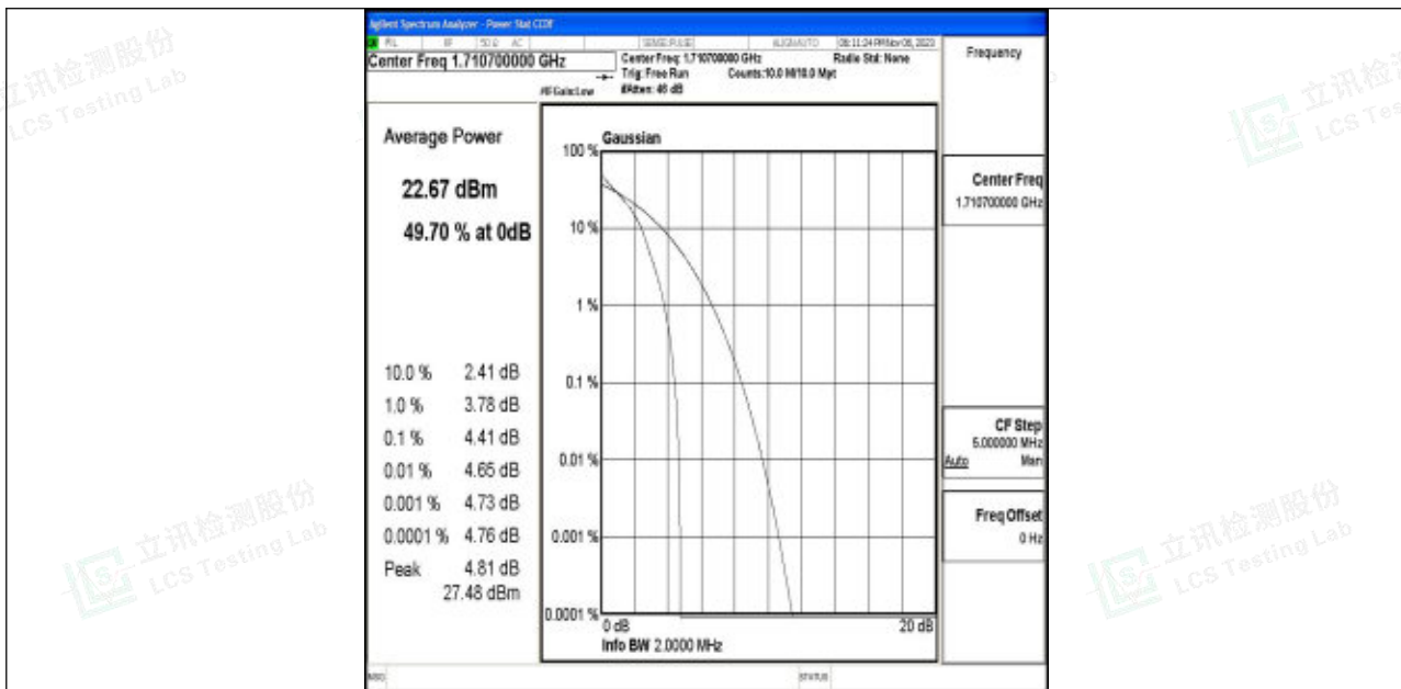
Band4-1.4MHz-64QAM-19957-1RB#0-PASS
