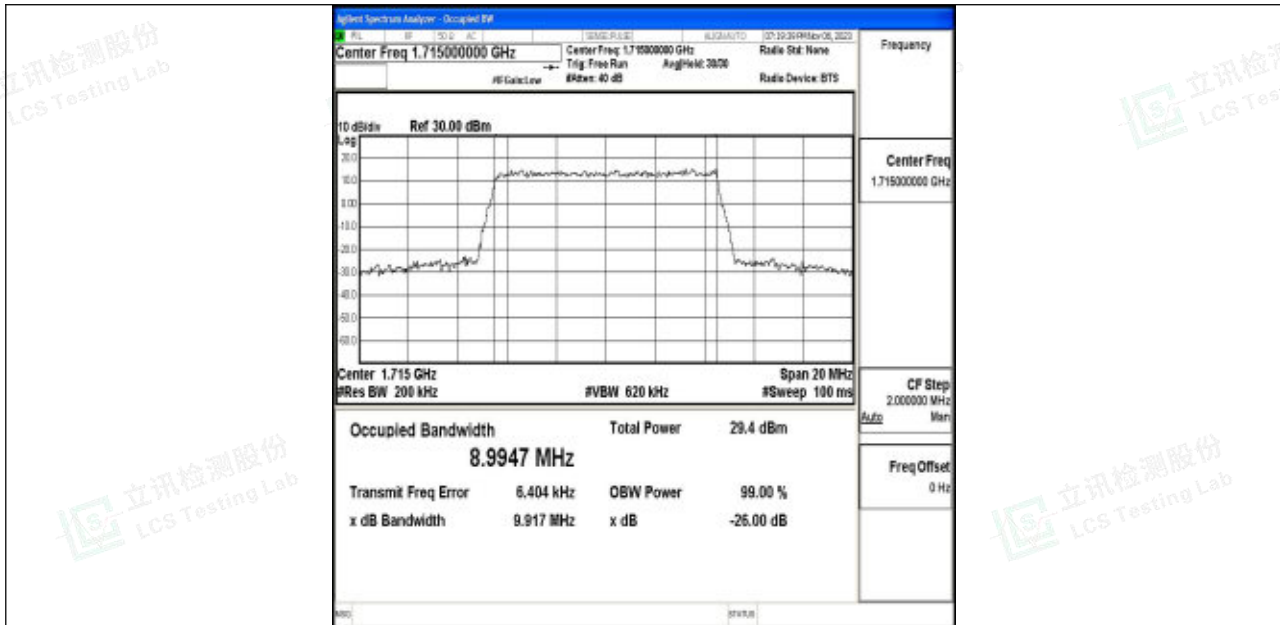
Band4-10MHz-16QAM-20000-50RB#0-PASS
