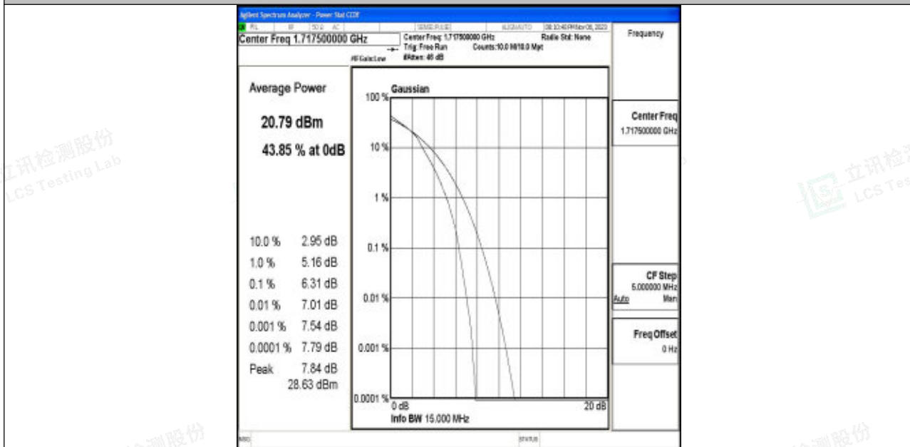
Band4-15MHz-16QAM-20025-75RB#0-PASS
