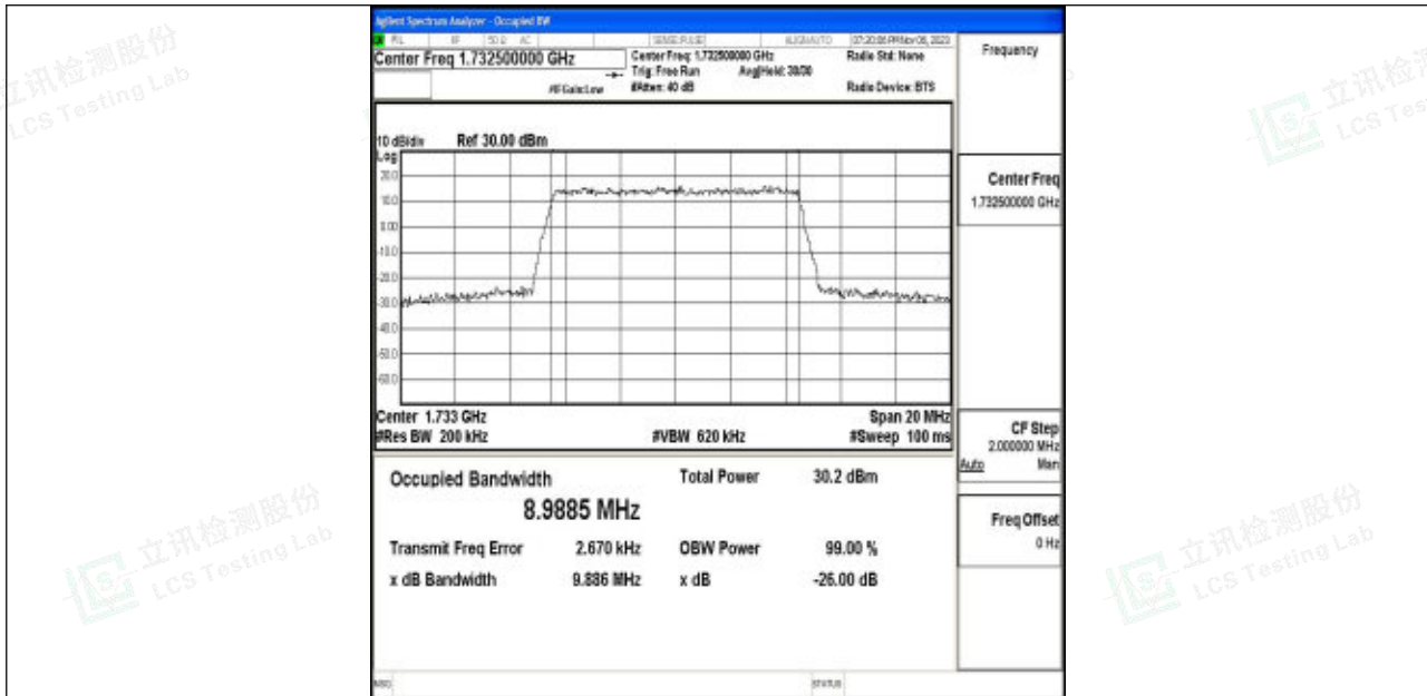
Band4-10MHz-QPSK-20175-50RB#0-PASS
