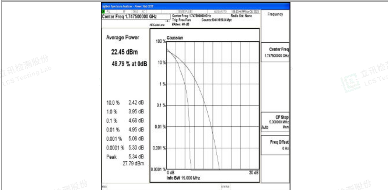
Band4-15MHz-64QAM-20325-1RB#0-PASS
