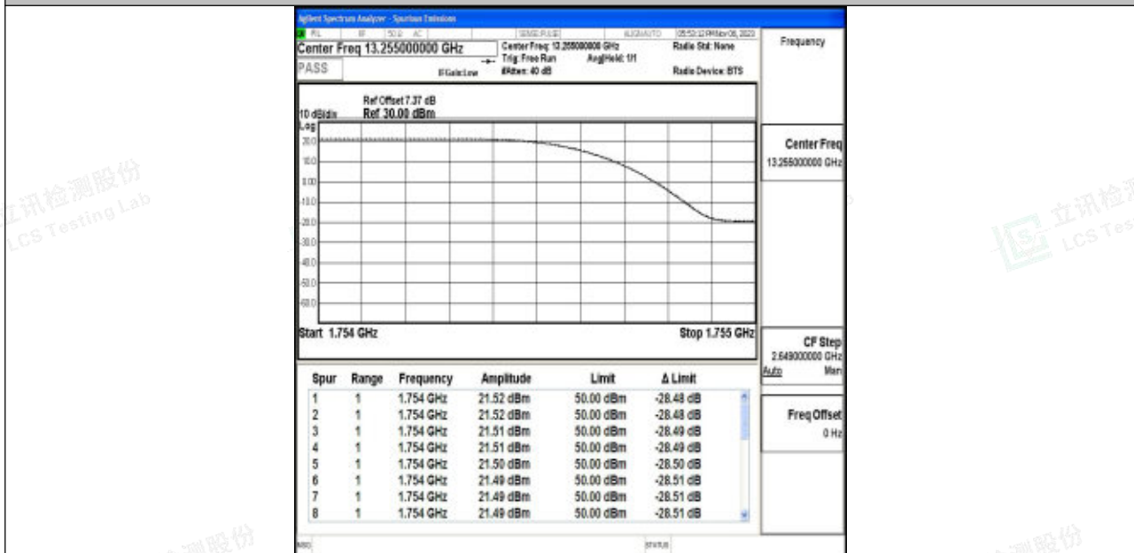
Band4_1.4MHz_QPSK_20393_1RB#0
