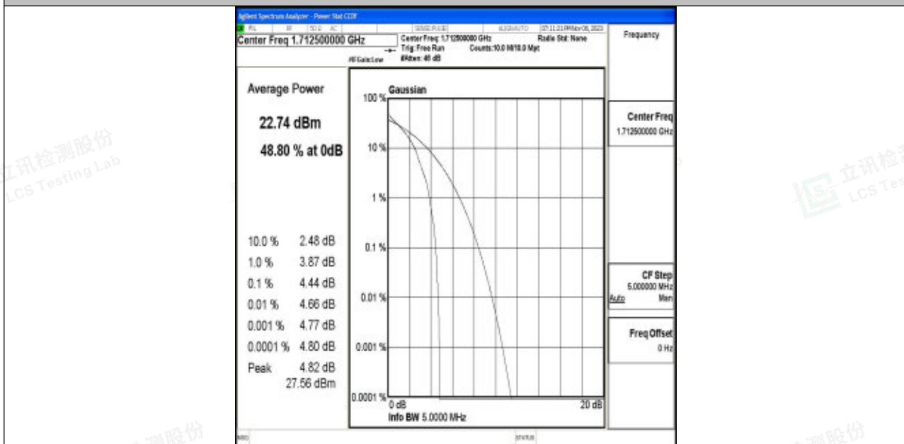
Band4-5MHz-64QAM-19975-1RB#0-PASS
