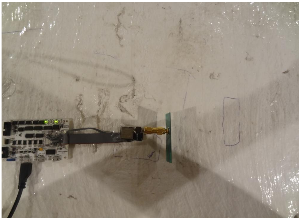
Test Setup
