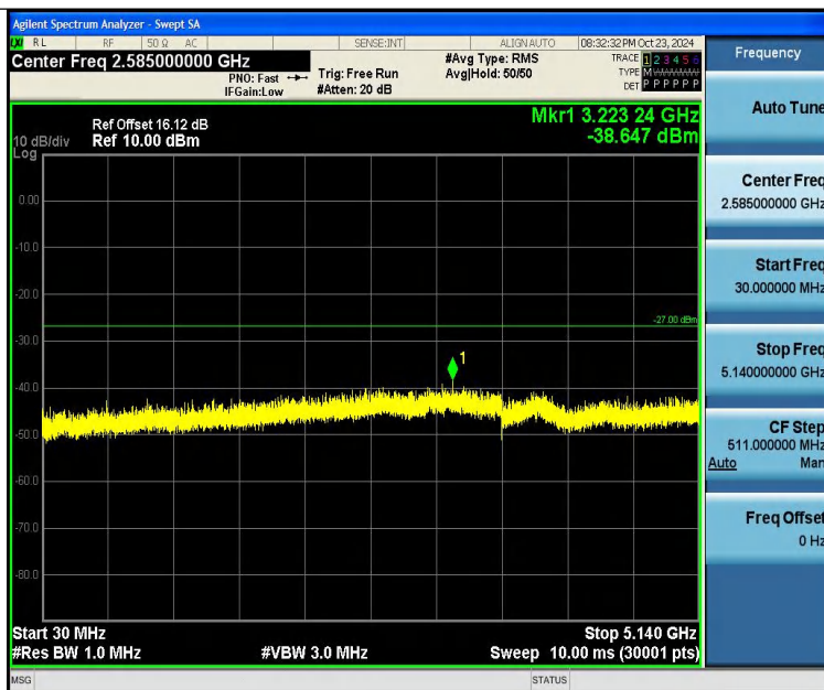
11N40SISO-Ant2-5230-30~5140-PASS
