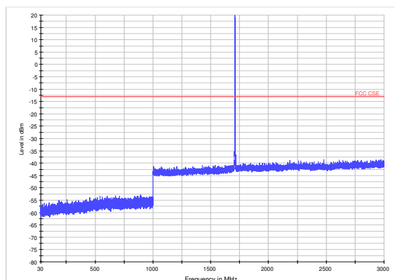
LTE Band 4 1.4MHz CH-Low 30MHz~3GHz
