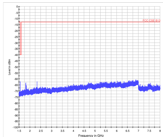
LTE Band 13 5MHz CH-Middle 1.5GHz~8GHz
