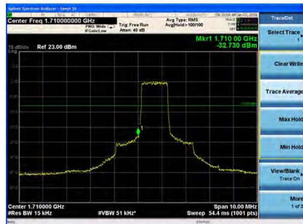
LTE Band 4 QPSK 3MHz CH-Low, 1 RB
