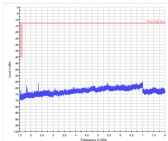
LTE Band 13 5MHz CH-High 1.5GHz~8GHz
