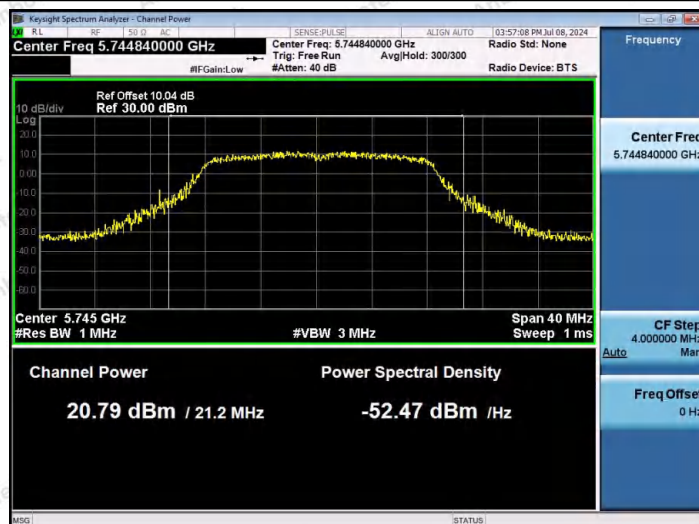
11A-Ant1-5745-PASS
