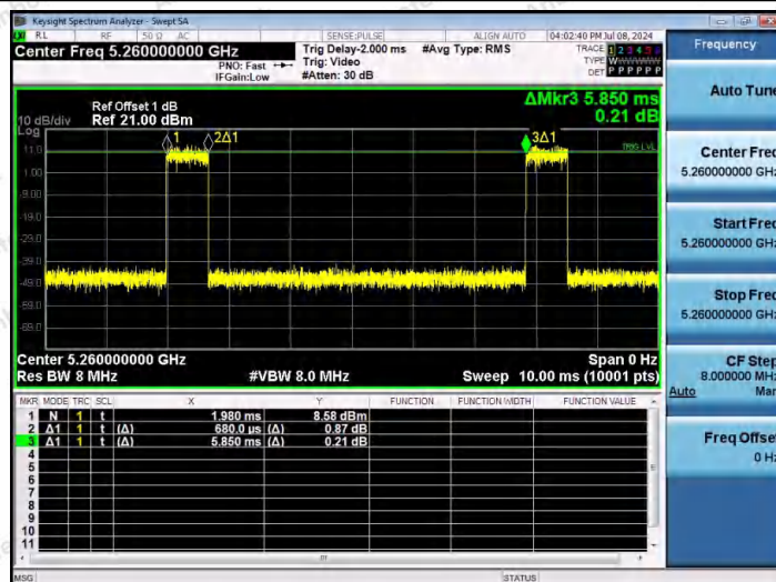
NTNV-11N20SISO-Ant1-5260
