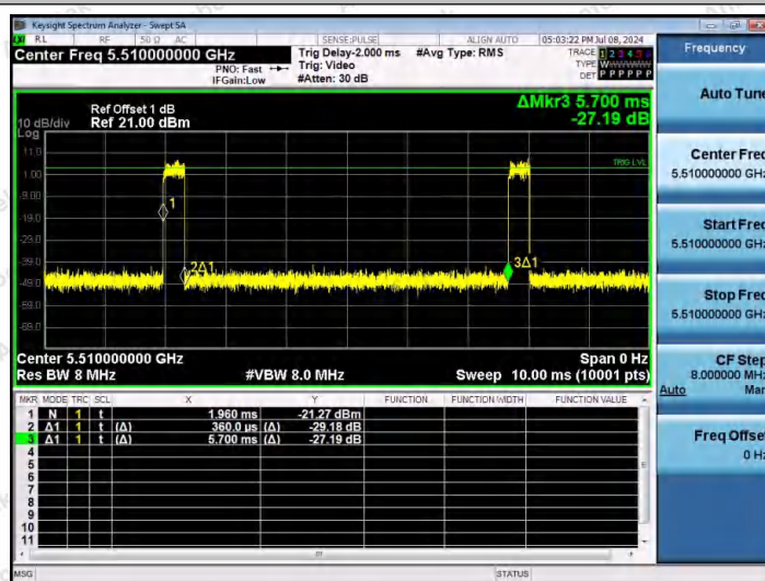
NTNV-11AC40SISO-Ant1-5510
