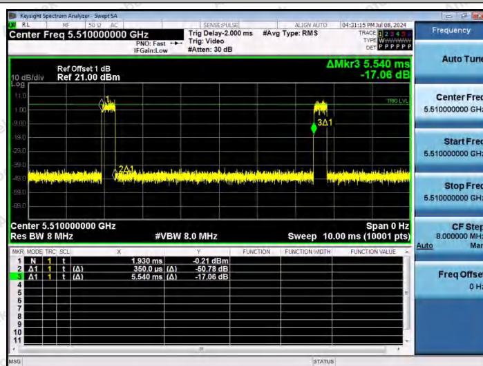
NTNV-11N40SISO-Ant1-5510
