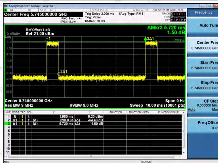
NTNV-11AC20SISO-Ant1-5745
