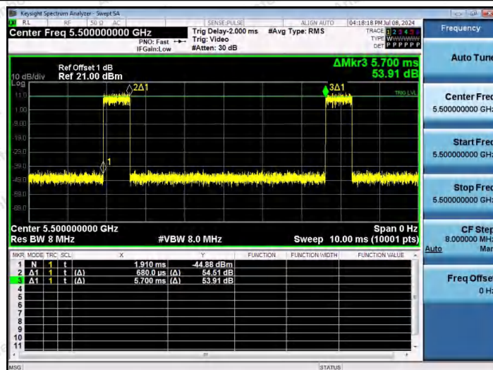
NTNV-11N20SISO-Ant1-5500
