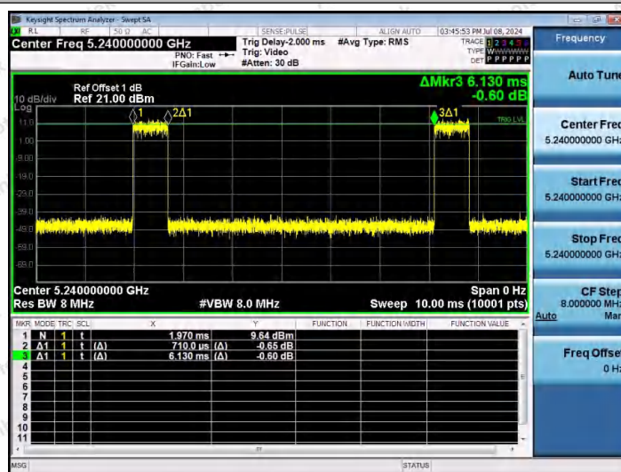
NTNV-11A-Ant1-5240
