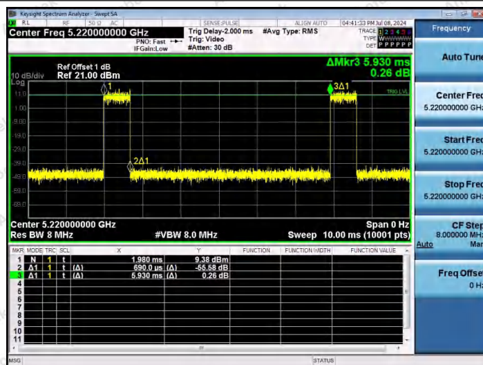
NTNV-11AC20SISO-Ant1-5220
