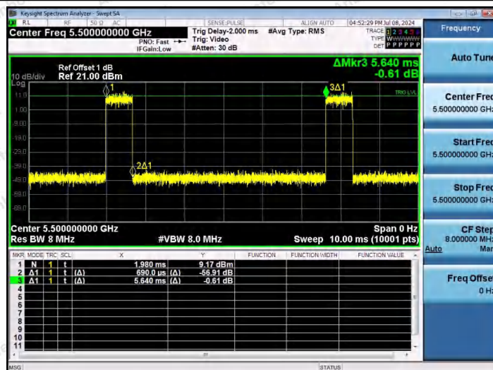
NTNV-11AC20SISO-Ant1-5500
