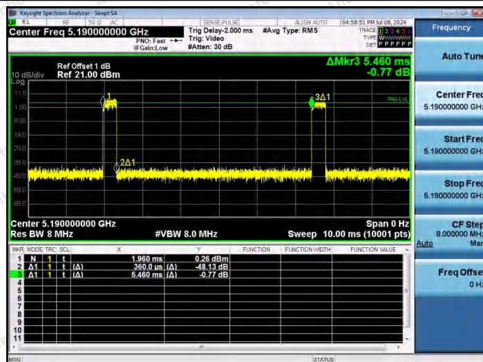
NTNV-11AC40SISO-Ant1-5190
