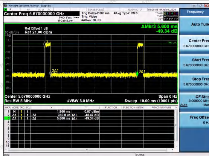
NTNV-11AC40SISO-Ant1-5670
