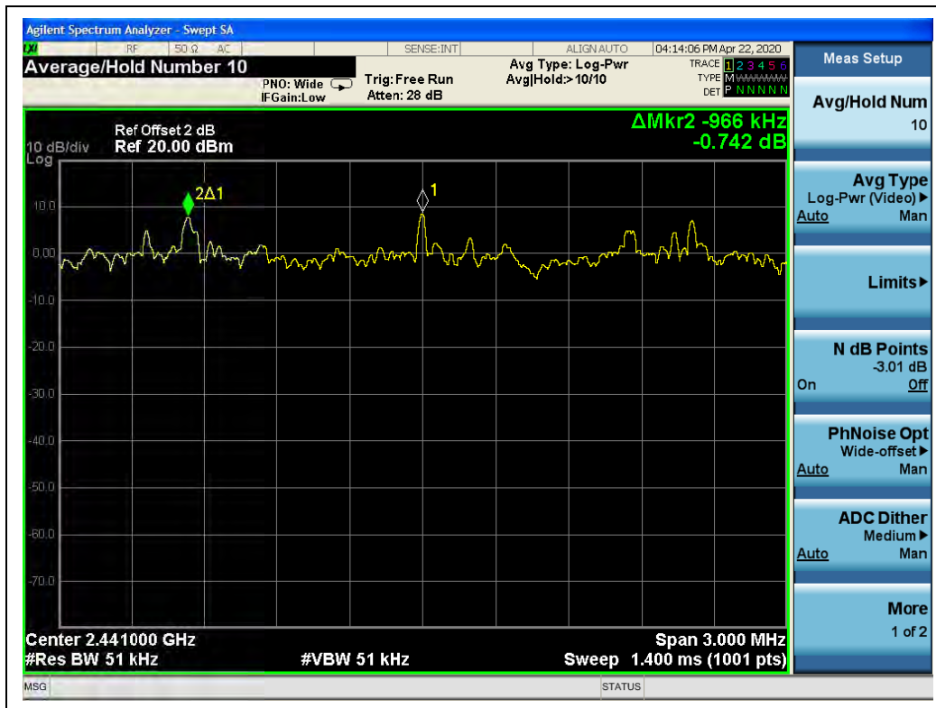
(\pi/4\text{-DQPSK})
