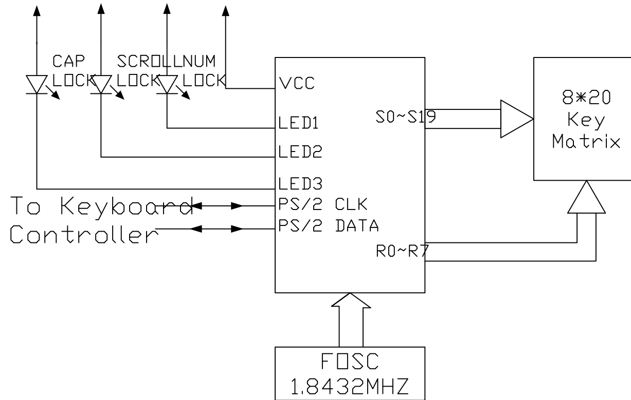
K3010 PS2 block diagram
