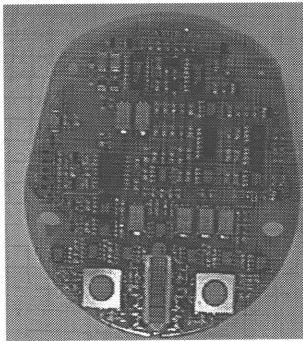
Figure 5 : RF Head (Top Side)
