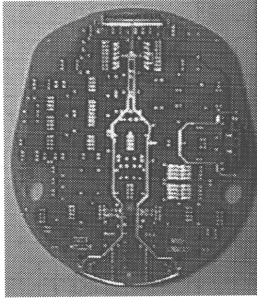
Figure 6 : RF Head (Bottom Side)
