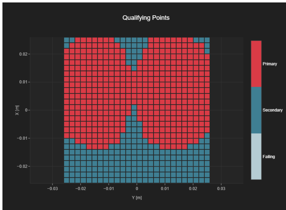
Fig A.9 T-Coil LTE-Band 7
