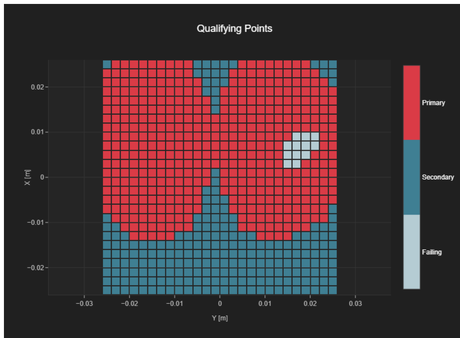
Fig A.12 T-Coil LTE-Band 17
