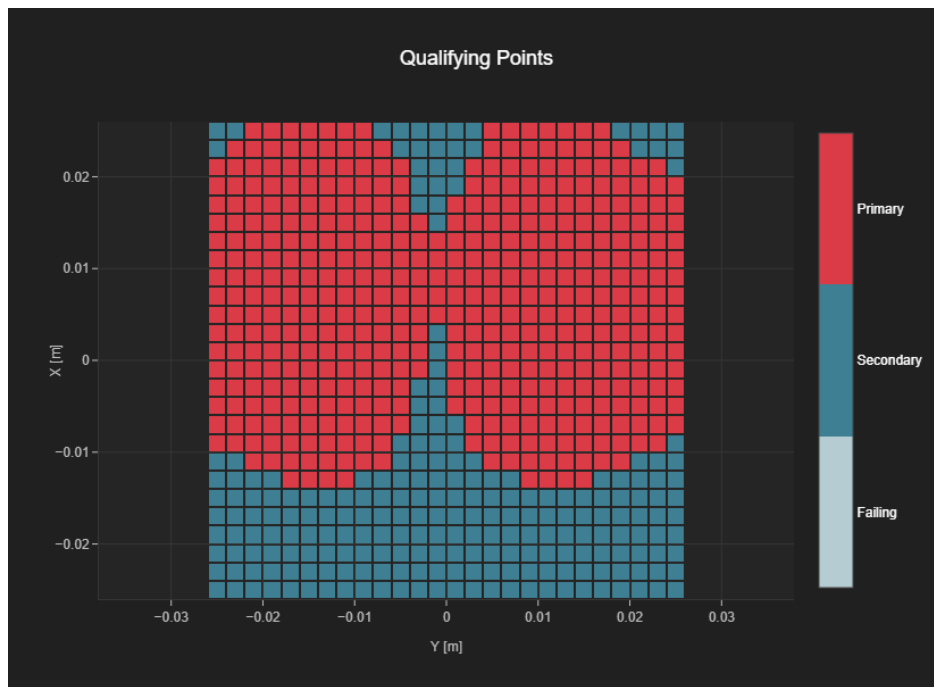
Fig A.10 T-Coil LTE-Band 12
