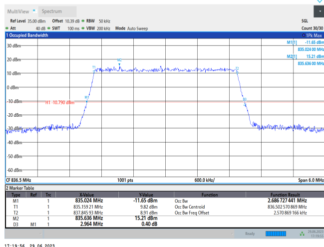
Band5-3MHz-64QAM-20525-15RB#0
