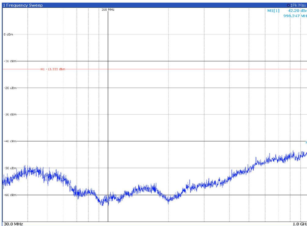
Channel: MIDDLE, Modulation: 64QAM, BW=90MHz, Range: 30MHz - 1GHz, Polarization: Horizontal
