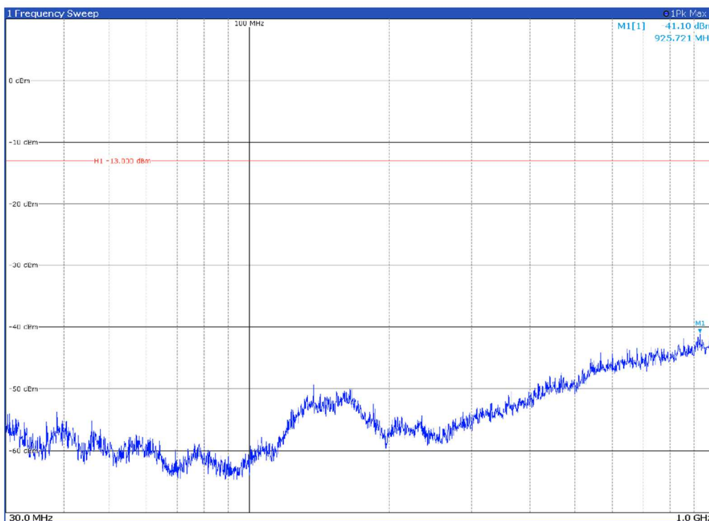
Channel: MIDDLE, Modulation: 64QAM, BW=90MHz, Range: 30MHz - 1GHz, Polarization: Vertical
