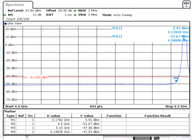
11AC20SISO-Ant3-5180-PASS
