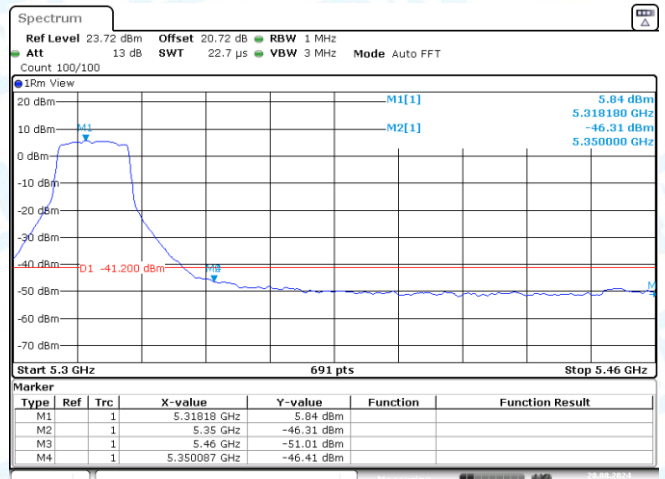
11N20SISO-Ant3-5320-PASS
