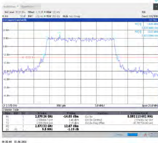
1-N38--30-10-L-3-DFT-16QAM-Outer_Full-24@0- Ant1-8.592-9.500≤10-PASS
