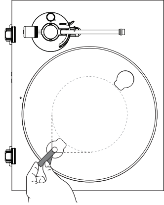
2. Fit the belt around the motor pulley
