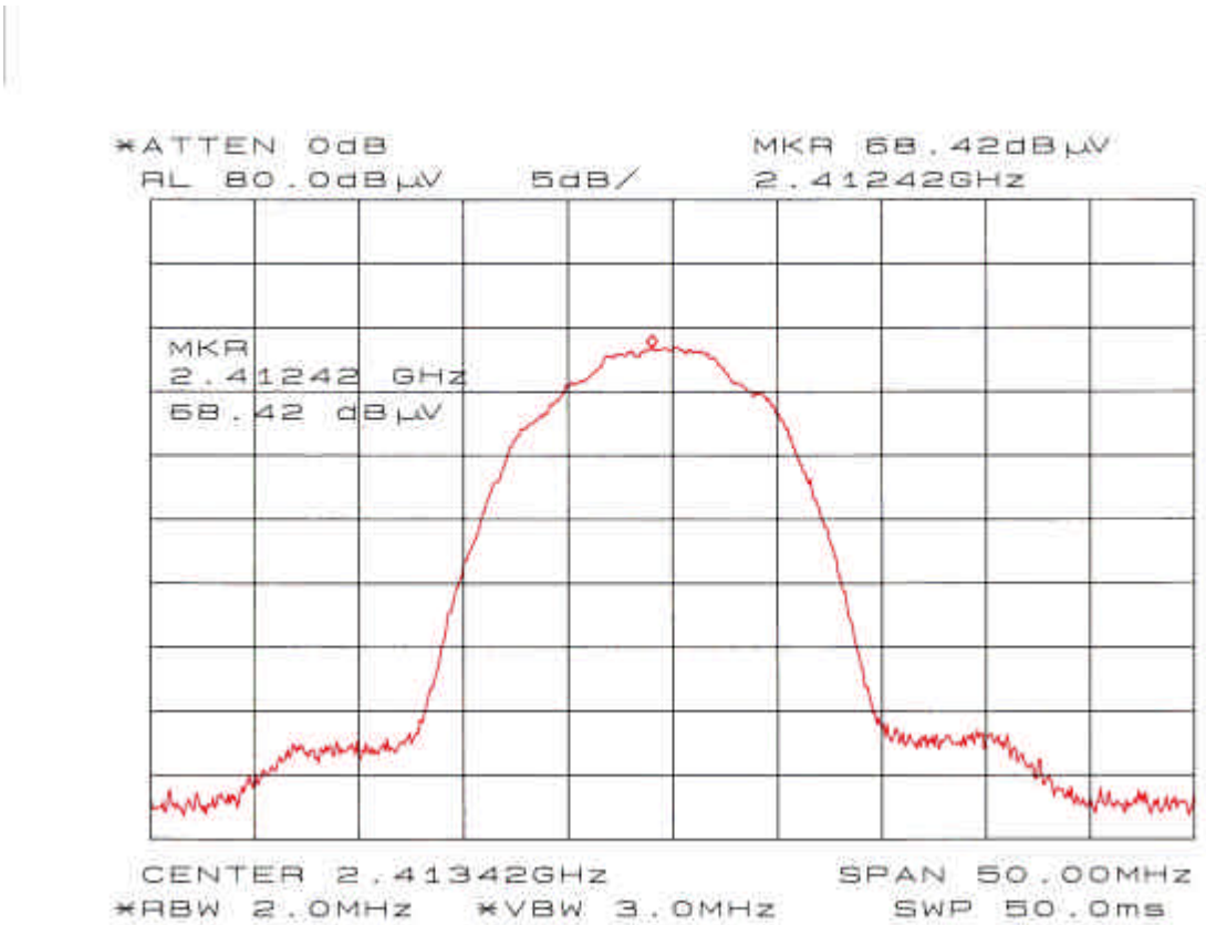
Chart of Maximum Peak Output Power in ch 1 and 11Mbps data rate
