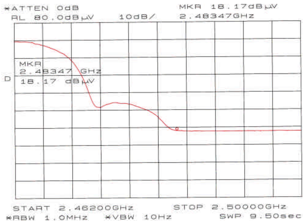
Chart of Restricted Bands of Operation in ch 11 and 11Mbps data rate
