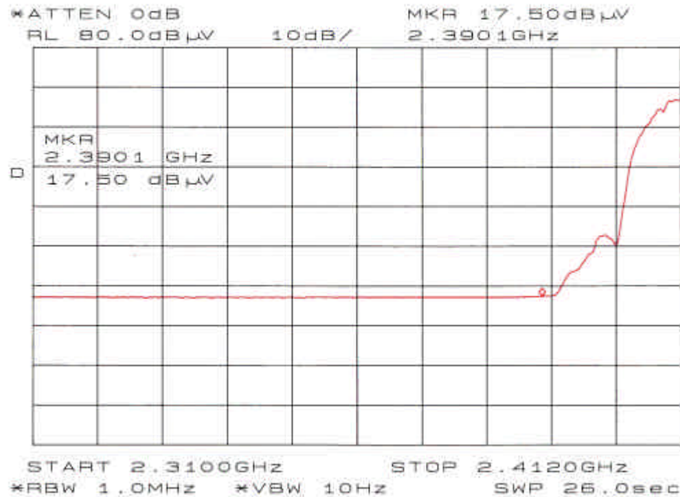
Chart of Restricted Bands of Operation in ch 1 and 11Mbps data rate
