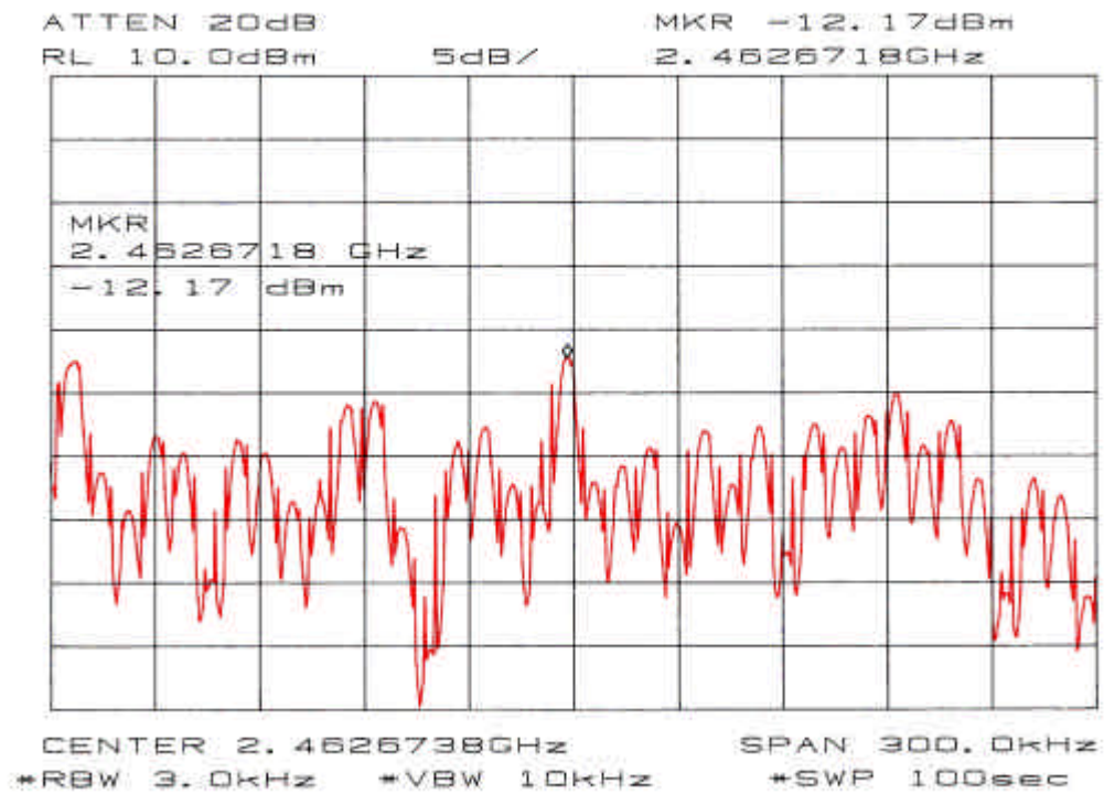
Chart of Power Spectral Density in ch 11 and 11Mbps data rate
