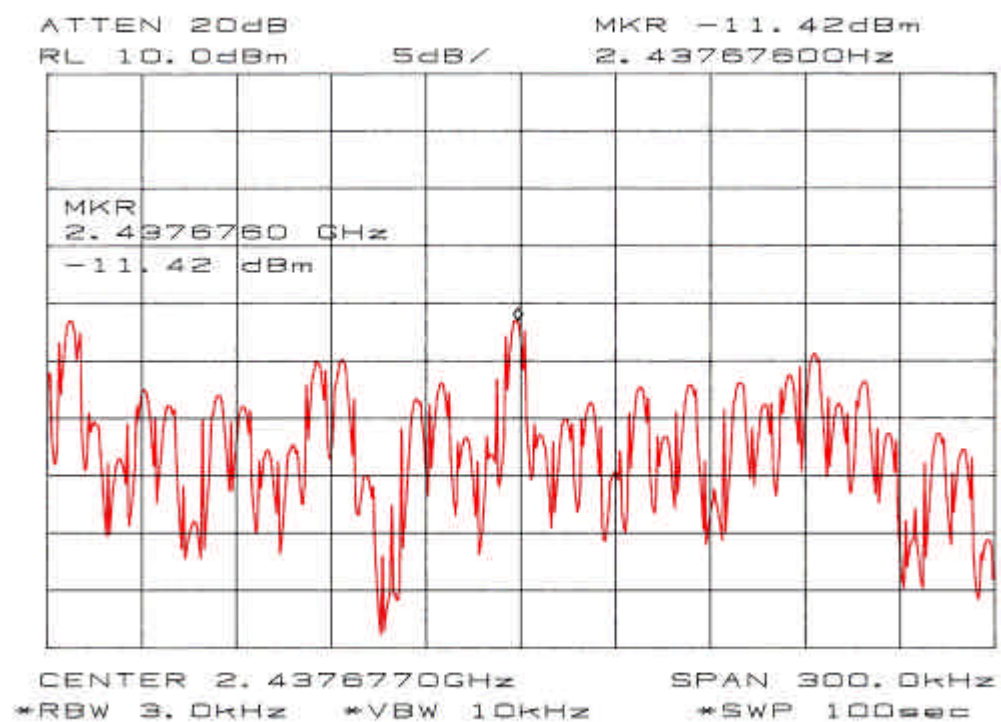
Chart of Power Spectral Density in ch 6 and 2Mbps data rate
