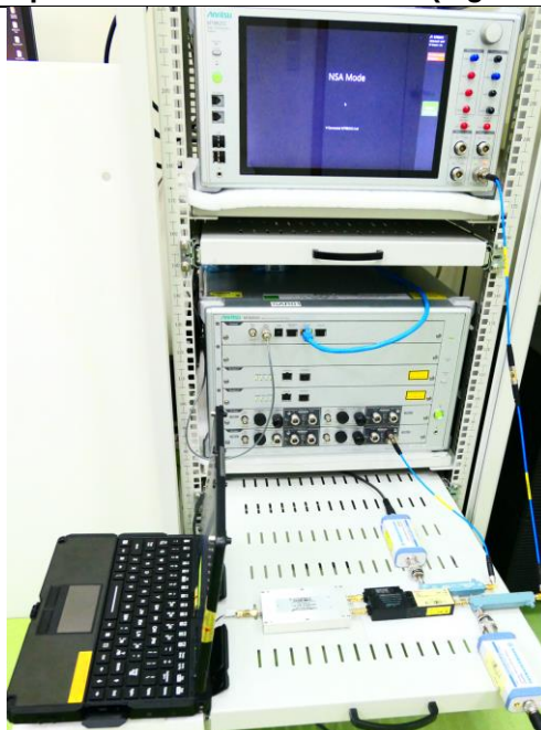
Setup for Conducted Power Test (Figure 4-3)
