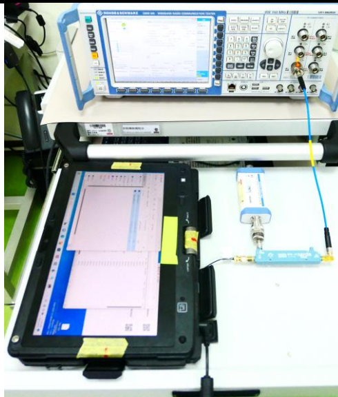
Setup for Conducted Power Test (Figure 4-1)
