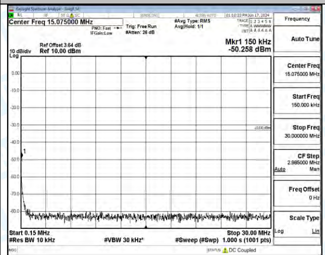
Band4_20MHz_16QAM_20050_1RB#99_1000-3000_1000-3000
