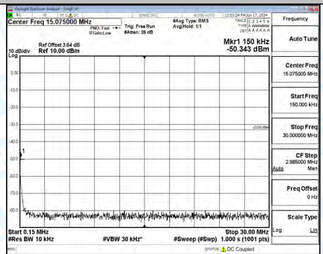
Band4_15MHz_QPSK_20325_1RB#74_1000~3000_1000~3000
