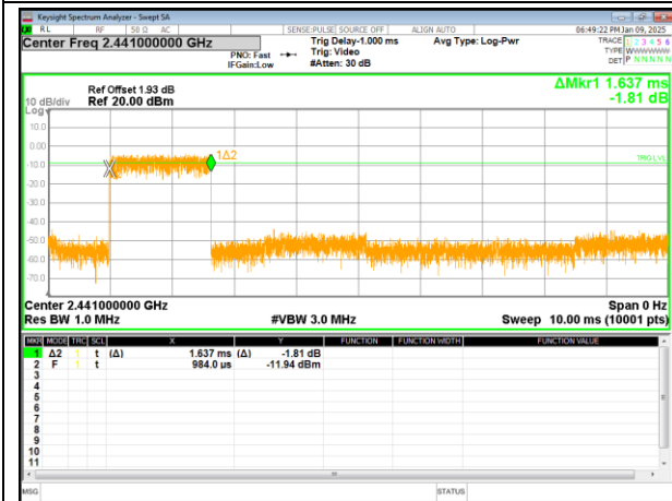
2DH5-2441MHz-One burst
