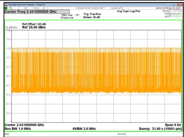
2DH3-2441MHz-Accumulated
