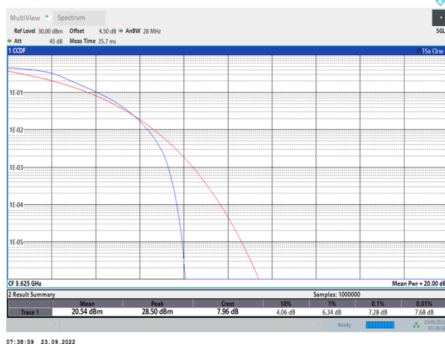
Band48-20MHz-QPSK-55990-100RB#0
