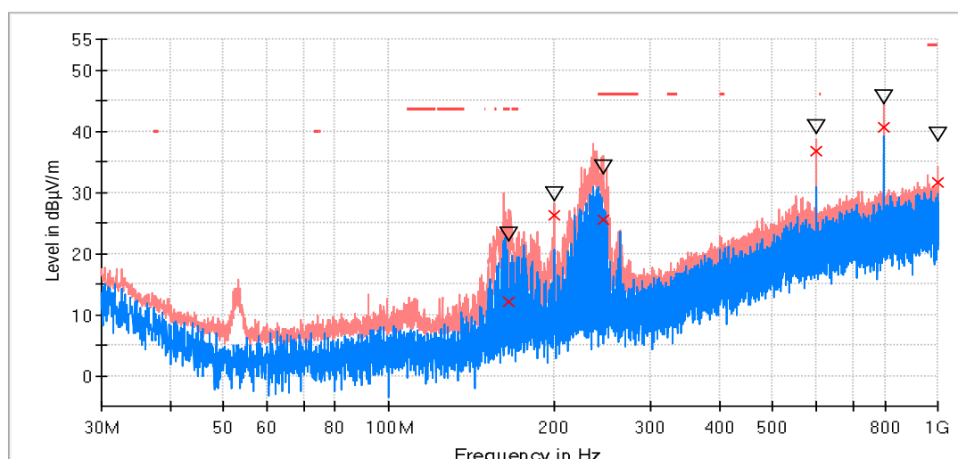
RF_FCC_15.247_E Field_30MHz_1GHz
