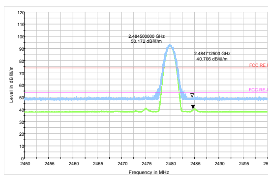
3DH5-Channel 78: Peak + Average
