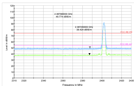
3DH5-Channel 0: Peak + Average
