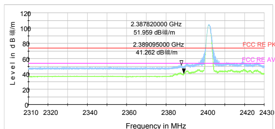
DH5-Channel 0: Peak + Average
