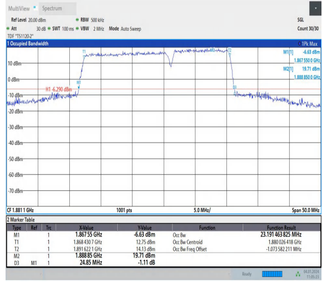
2-2-15MHz-10MHz-64QAM-64QAM-18851-18971-75RB#0-50 RB#0-PASS
