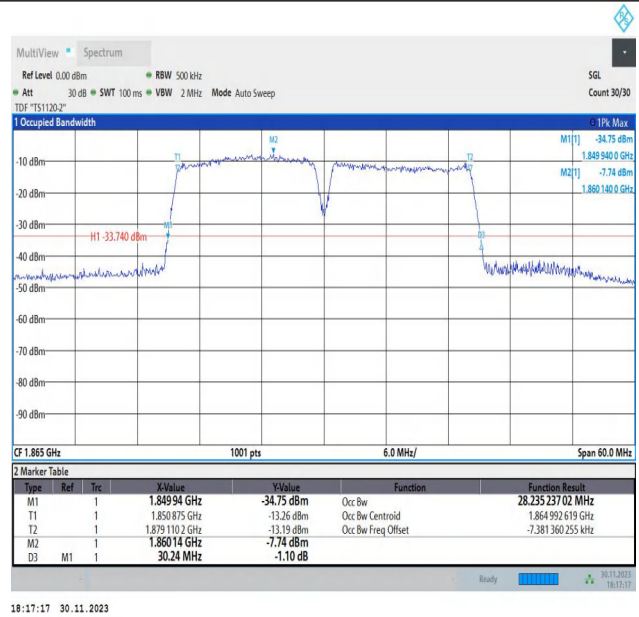
2-2-15MHz-15MHz-QPSK-QPSK-18675-18825-75RB#0-75RB #0-PASS
