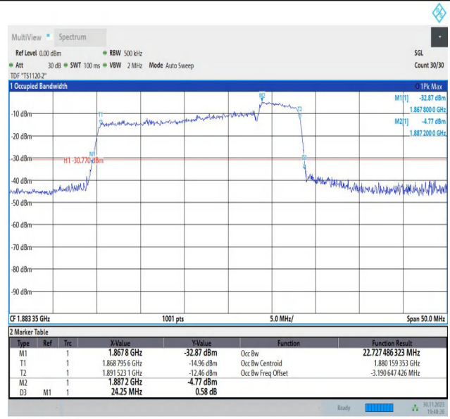
2-2-20MHz-5MHz-QPSK-QPSK-18875-18992-100RB#0-25RB #0-PASS
