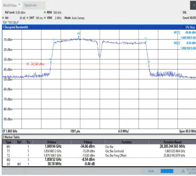
2-2-15MHz-15MHz-16QAM-16QAM-18675-18825-75RB#0-75 RB#0-PASS
