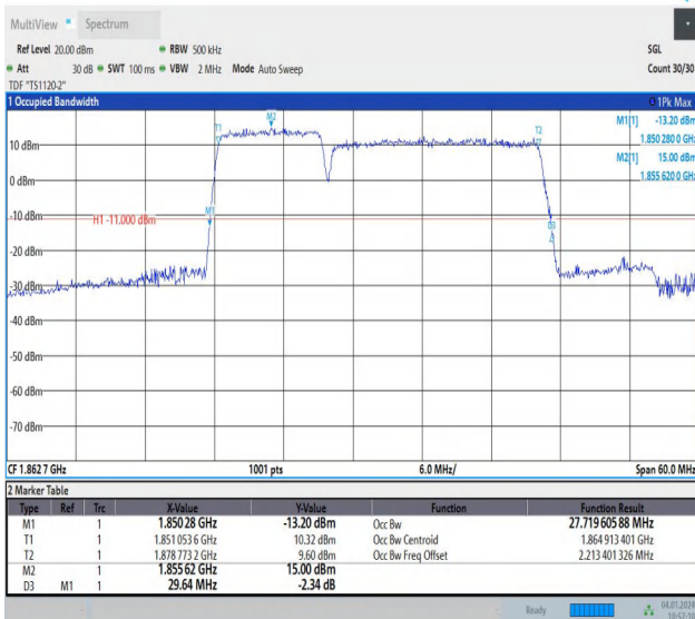
2-2-10MHz-20MHz-64QAM-64QAM-18655-18799-50RB#0-10 ORB#0-PASS
