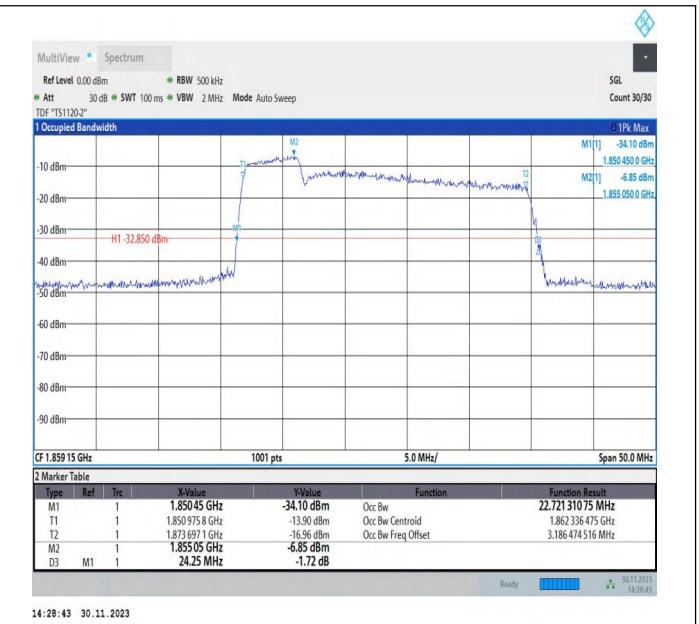
2-2-5MHz-20MHz-16QAM-16QAM-18633-18750-25RB#0-100 RB#0-PASS
