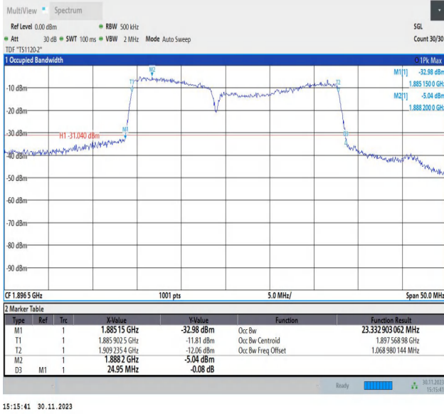
2-2-10MHz-15MHz-16QAM-16QAM-19005-19125-50RB#0-75 RB#0-PASS
