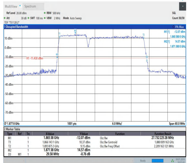
2-2-10MHz-20MHz-64QAM-64QAM-18806-18950-50RB#0-10 ORB#0-PASS
