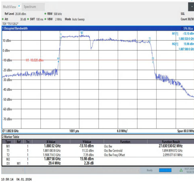
2-2-10MHz-20MHz-64QAM-64QAM-18956-19100-50RB#0-10 0RB#0-PASS
