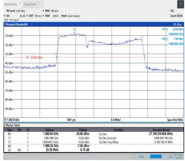
2-2-10MHz-20MHz-16QAM-16QAM-18956-19100-50RB#0-10 0RB#0-PASS
