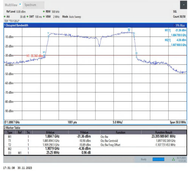
2-2-15MHz-10MHz-QPSK-QPSK-19027-19147-75RB#0-50RB #0-PASS
