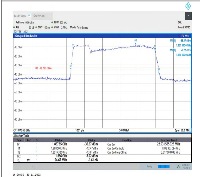
2-2-5MHz-20MHz-QPSK-QPSK-18808-18925-25RB#0-100RB #0-PASS
