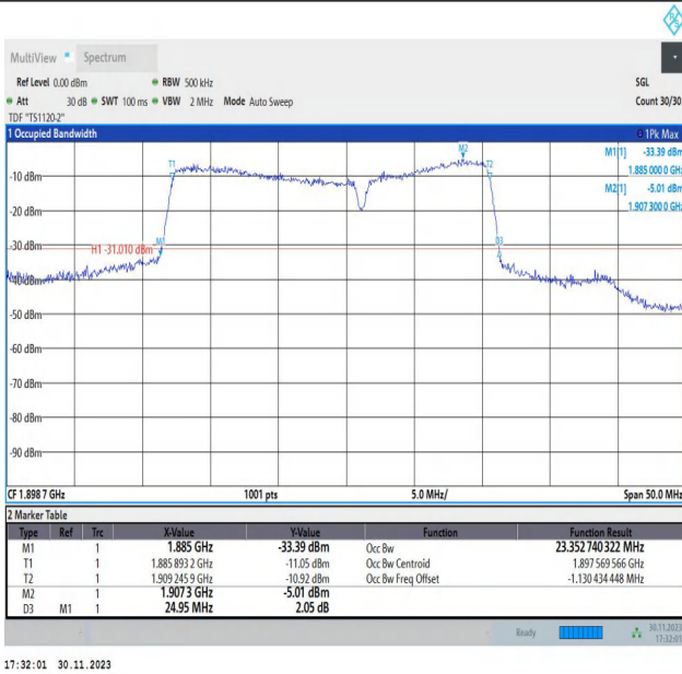
2-2-15MHz-10MHz-16QAM-16QAM-19027-19147-75RB#0-50 RB#0-PASS
