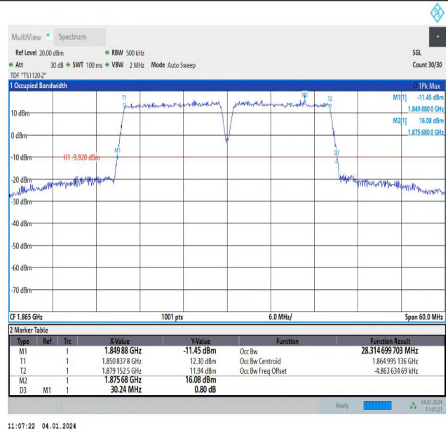
2-2-15MHz-15MHz-64QAM-64QAM-18675-18825-75RB#0-75 RB#0-PASS
