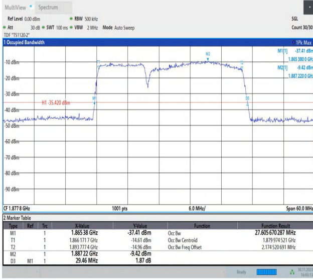
2-2-10MHz-20MHz-16QAM-16QAM-18806-18950-50RB#0-10 ORB#0-PASS
