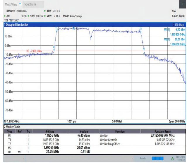
2-2-10MHz-15MHz-64QAM-64QAM-19005-19125-50RB#0-75 RB#0-PASS
