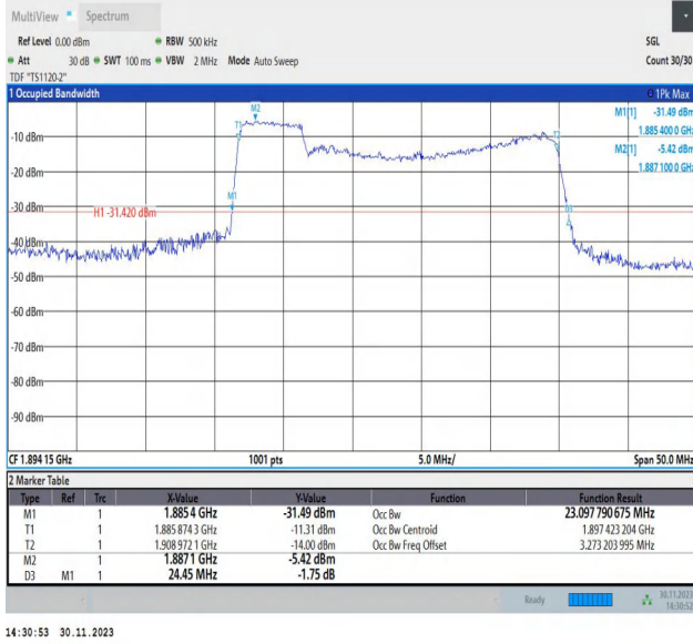
2-2-5MHz-20MHz-QPSK-QPSK-18983-19100-25RB#0-100RB #0-PASS
