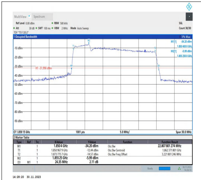
2-2-5MHz-20MHz-QPSK-QPSK-18633-18750-25RB#0-100RB #0-PASS
