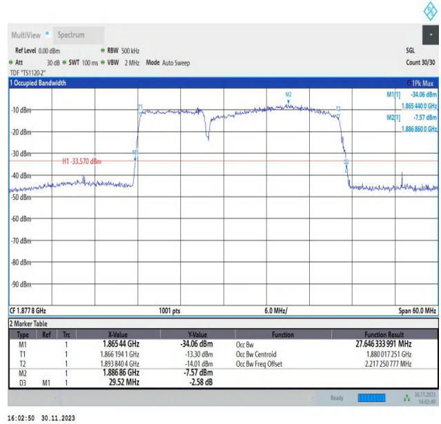
2-2-10MHz-20MHz-QPSK-QPSK-18806-18950-50RB#0-100R B#0-PASS
