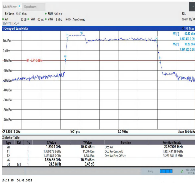
2-2-5MHz-20MHz-64QAM-64QAM-18633-18750-25RB#0-100 RB#0-PASS
