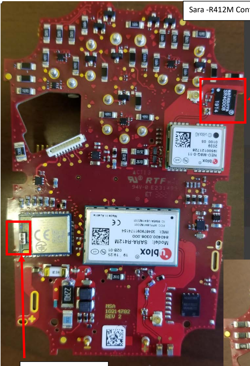
Bluetooth Antenna
