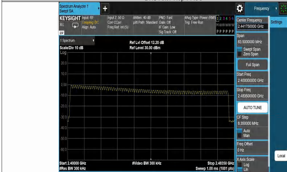
2DH5-Ant1-Hop-PASS
