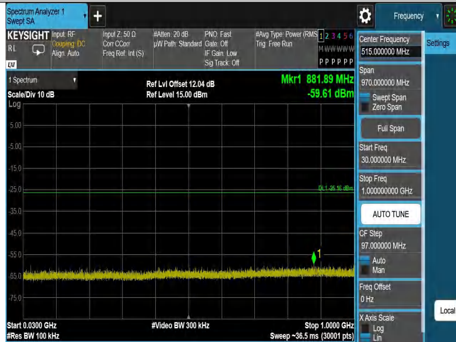
DH5-Ant1-2480-30~1000-PASS
