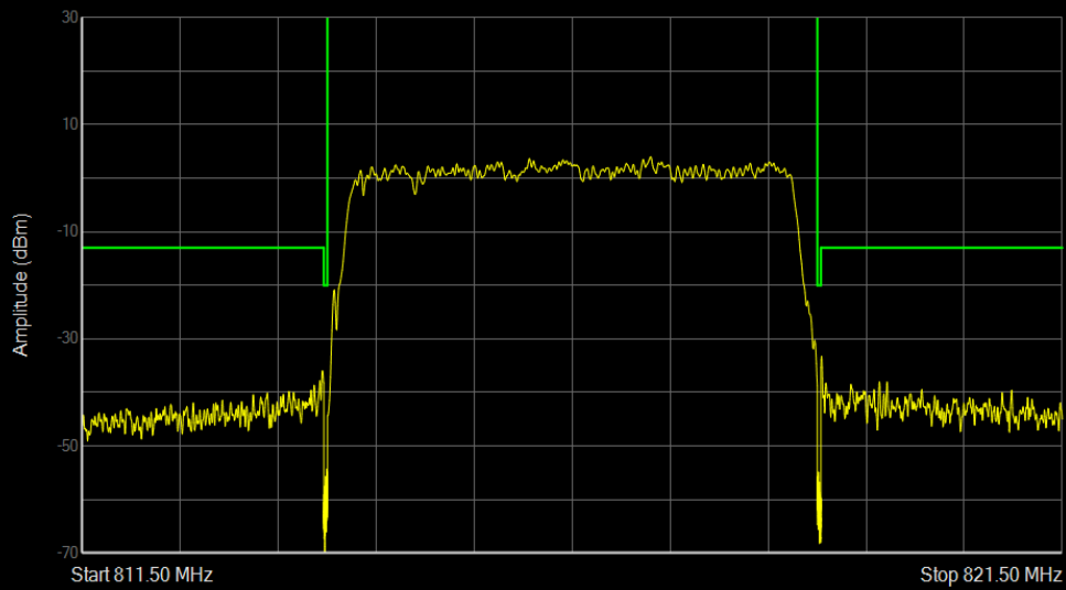
Band26a 16QAM BW=5MHz Channel=26715 RB Size=25 Position=#0
