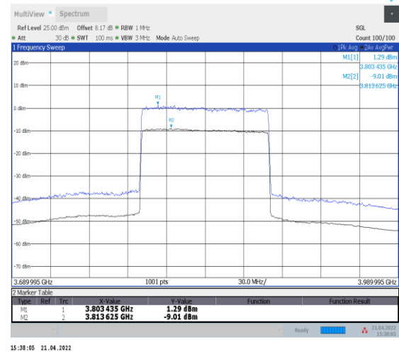
1-N77-3700-3980--30-100-M-2-CP-256QAM-Outer_Full-273@0-Ant0-10.30-100%-0.00-10.30-PASS-≤13
