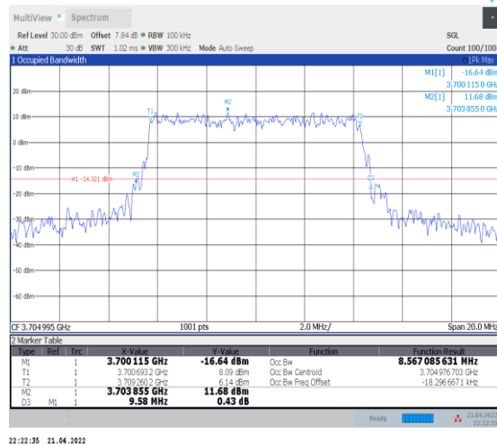
1-N77-3700-3980--30-10-L-4-DFT-64QAM-Outter_Full -24@0-Ant0-8.567-9.580-≤10-PASS
