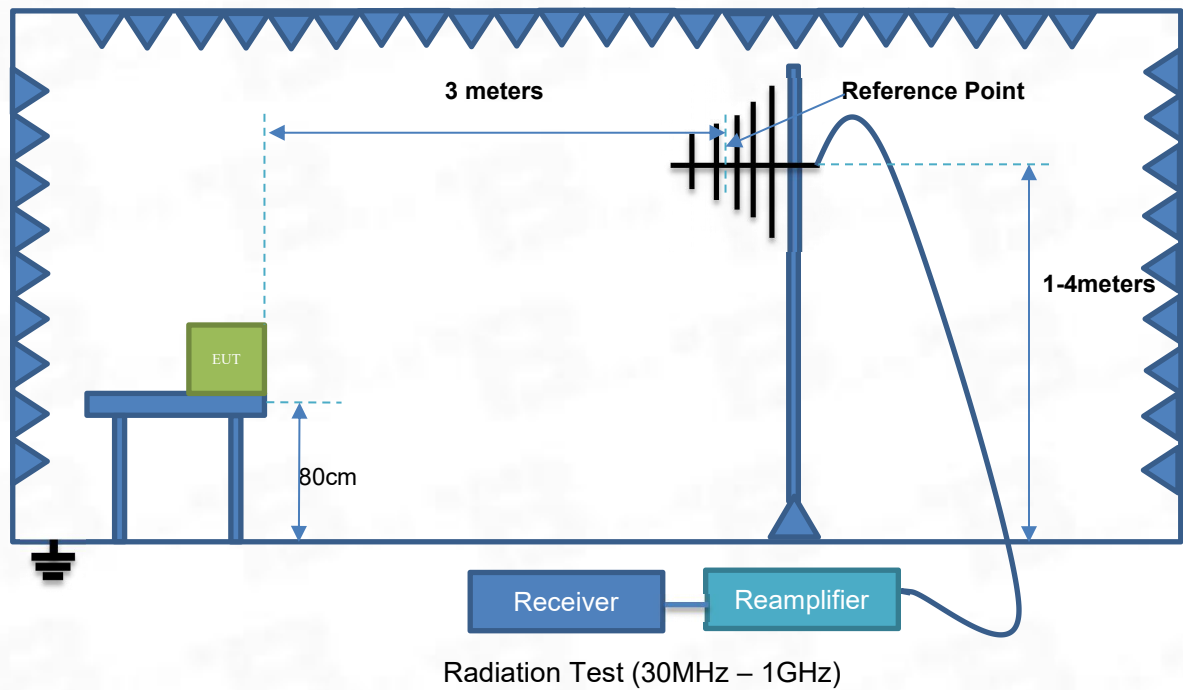
Test Setup 1
