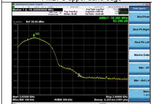
11 MBPS upper band-edge
